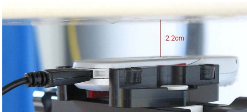
Fig. 52: Body worn configuration ARC, GPRS mode (2 TX slots) with data cable, antenna towards the phantom.
