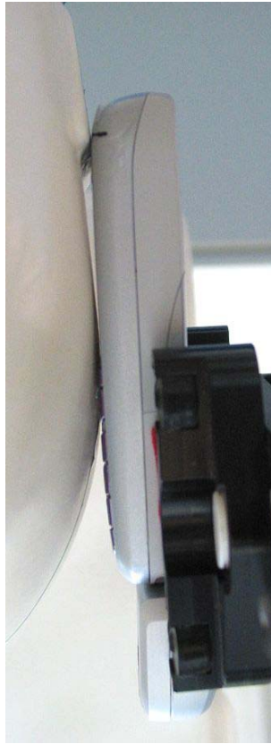
Fig. 43: Cheek position, left side, ARC with flash.
