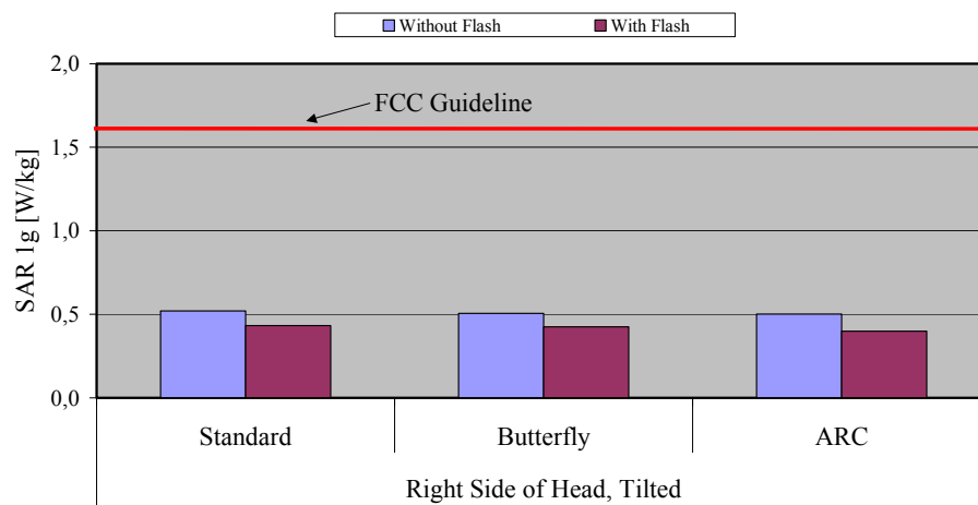
Fig. 11: The measured head phantom SAR values for the Siemens C65 without and with flash for PCS 1900 in comparison to the FCC exposure limit.
