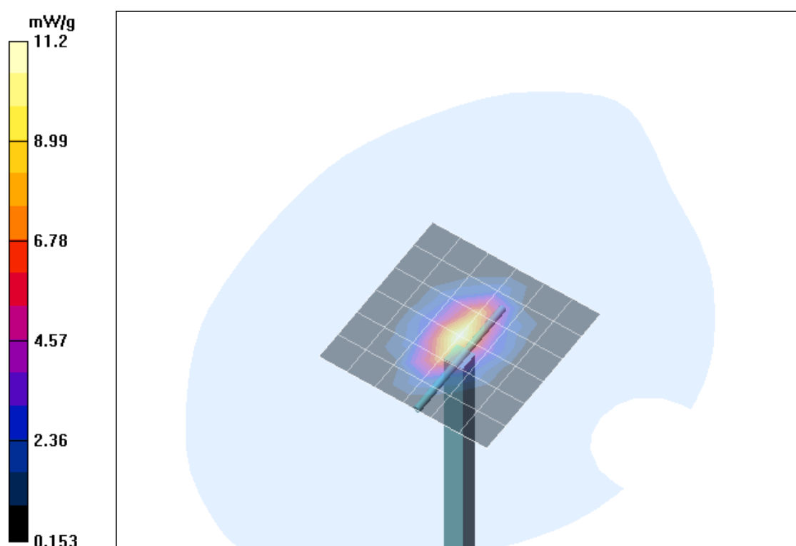
Fig. 13: Validation measurement 1900 MHz Head (May 11, 2004), coarse grid. Ambient Temperature: 20.2° C, Liquid Temperature: 19.6° C.
