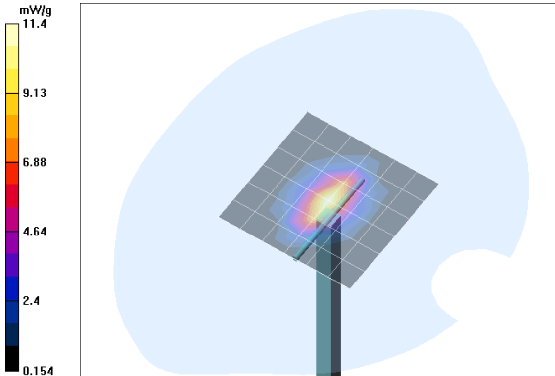
Fig. 14: Validation measurement 1900 MHz Head (May 12, 2004), coarse grid. Ambient Temperature: 20.0° C, Liquid Temperature: 19.4° C.
