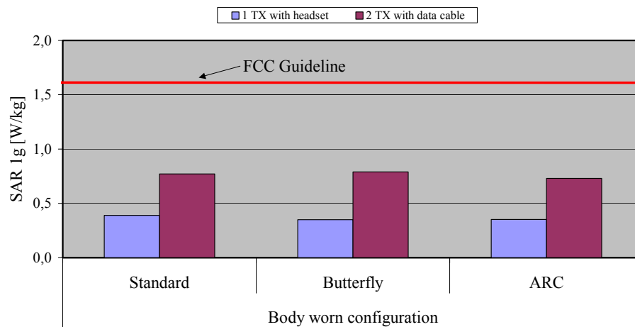
Fig. 12: The measured SAR values in body-worn configuration for the Siemens C65 for PCS 1900 (1 TX slot with headset and 2 TX slots with data cable, gap = 22 mm) in comparison to the FCC exposure limit.
