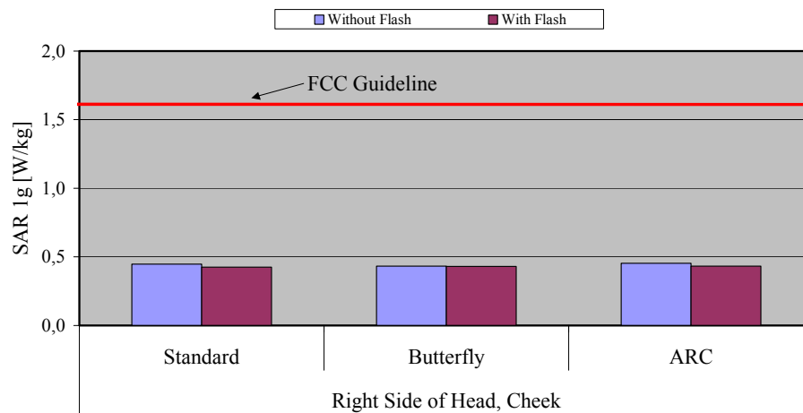
Fig. 10: The measured head phantom SAR values for the Siemens C65 without and with flash for PCS 1900 in comparison to the FCC exposure limit.
