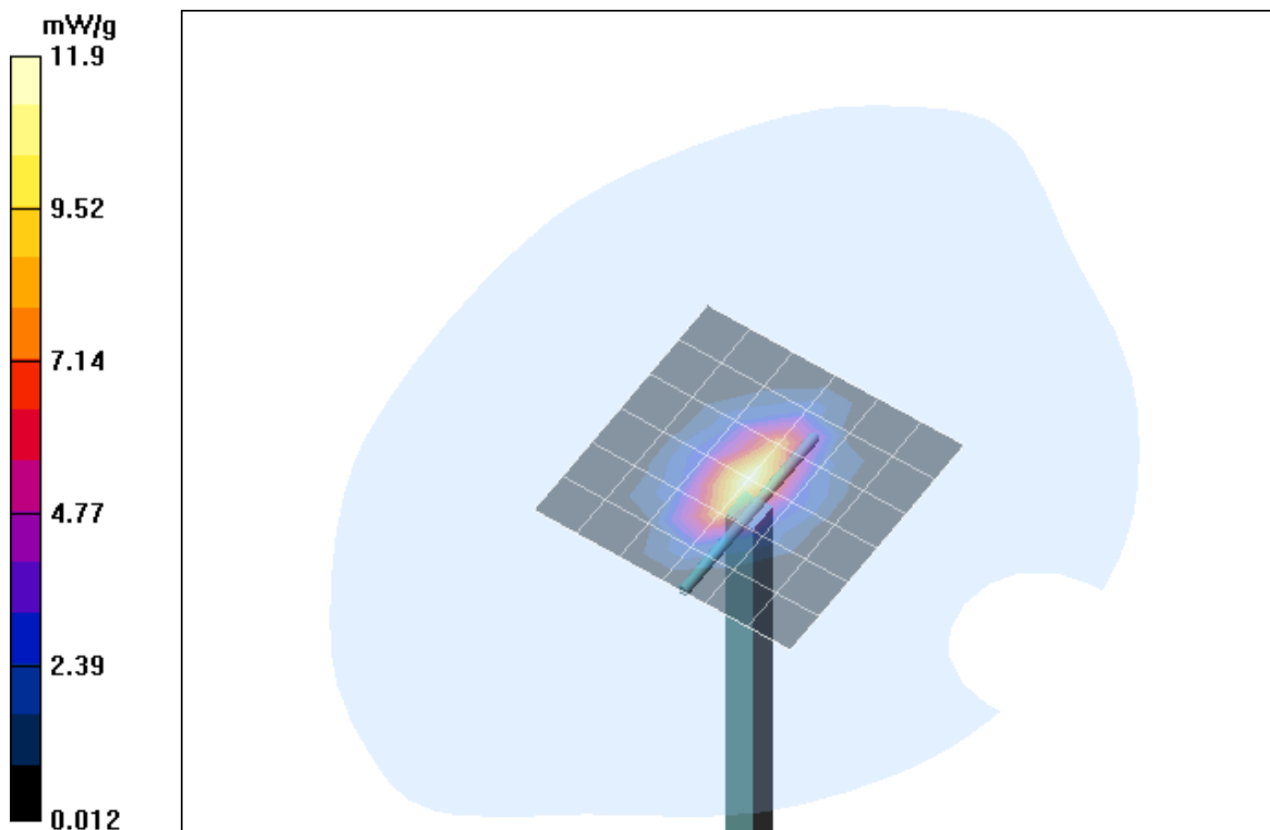
Fig. 15: Validation measurement 1900 MHz body (May 06, 2004), coarse grid. Ambient Temperature: 20.1° C, Liquid Temperature: 19.1° C.
