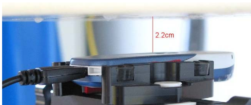
Fig. 50: Body worn configuration Standard, GPRS mode (2 TX slots) with data cable, antenna towards the phantom.
