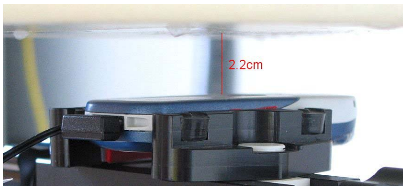
Fig. 47: Body worn configuration Standard, GSM mode (1 TX slot) with headset, antenna towards the phantom.
