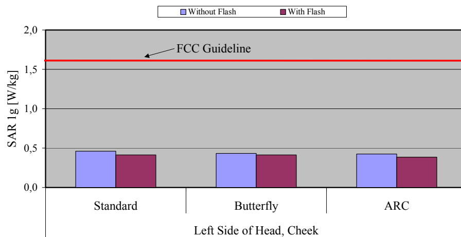
Fig. 8: The measured head phantom SAR values for the Siemens C65 without and with flash for PCS 1900 in comparison to the FCC exposure limit.
