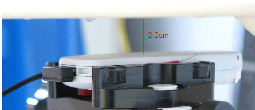
Fig. 48: Body worn configuration Butterfly, GSM mode (1 TX slot) with headset, antenna towards the phantom.
