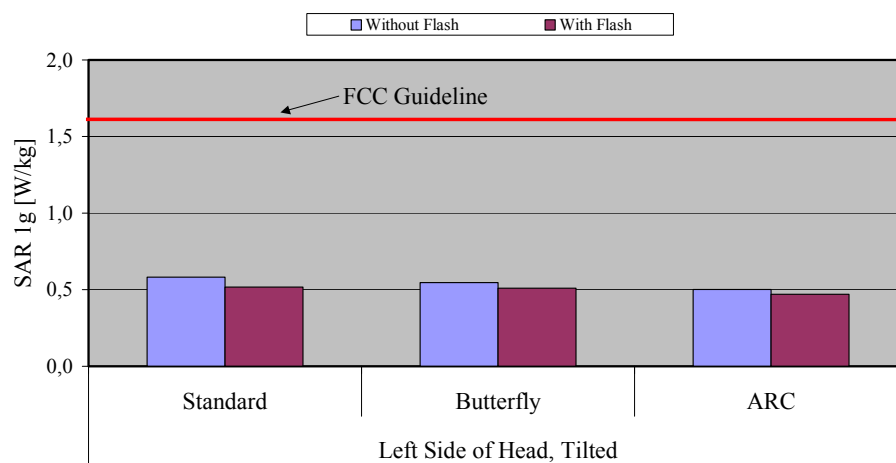
Fig. 9: The measured head phantom SAR values for the Siemens C65 without and with flash for PCS 1900 in comparison to the FCC exposure limit.
