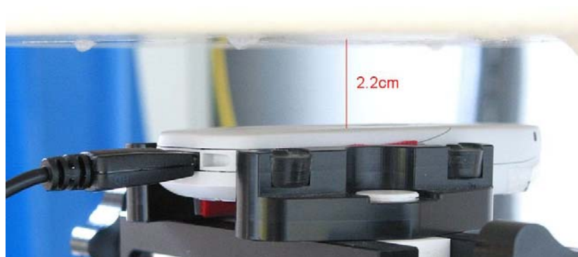
Fig. 51: Body worn configuration Butterfly, GPRS mode (2 TX slots) with data cable, antenna towards the phantom.
