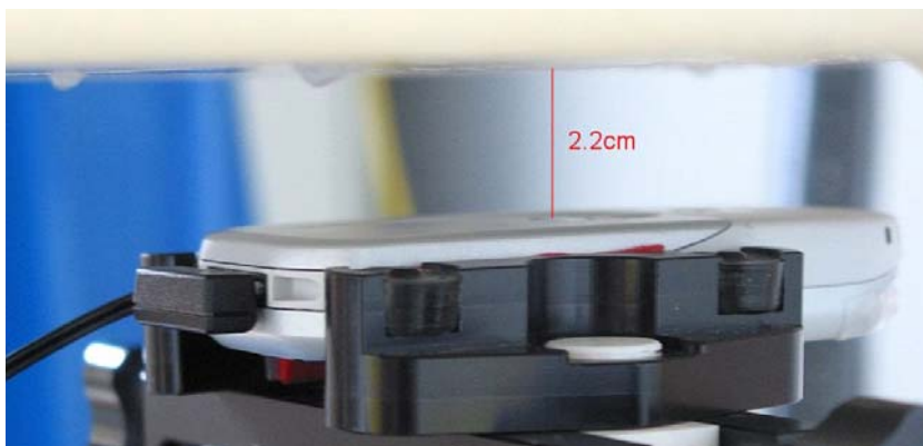
Fig. 49: Body worn configuration ARC, GSM mode (1 TX slot) with headset, antenna towards the phantom.
