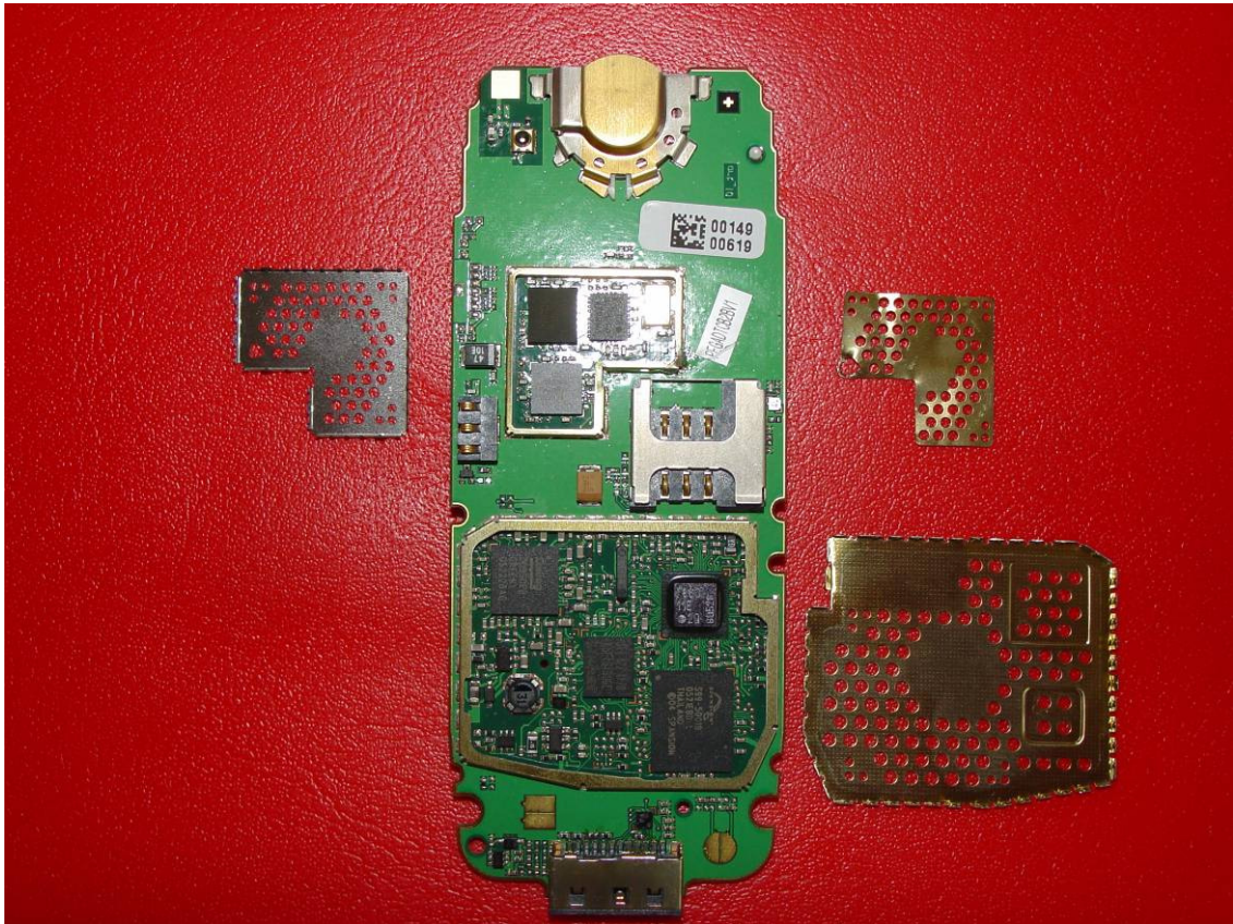
AX72 Back view shields removed
