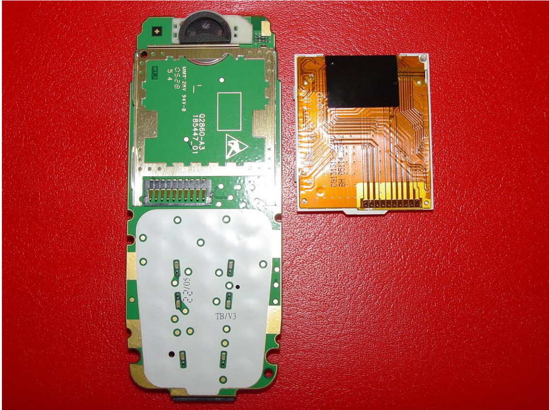
AX72 Display module removed
