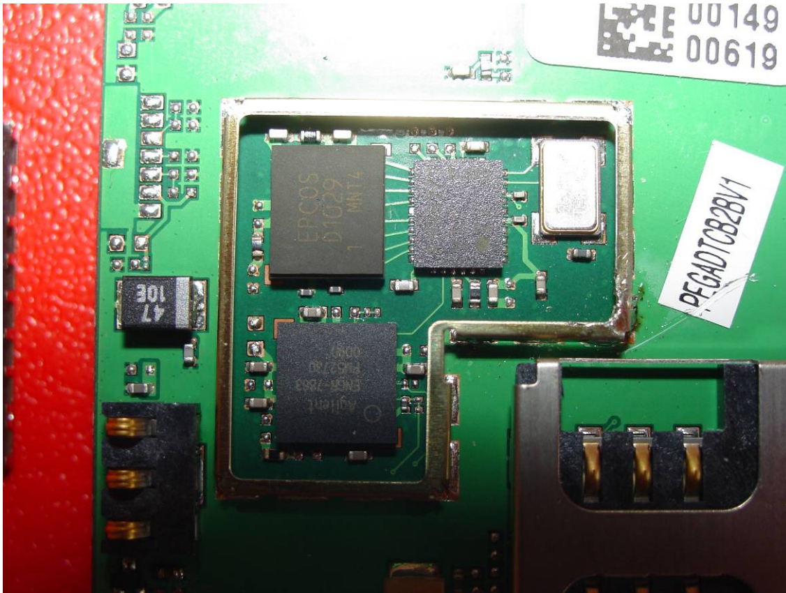
AX72 RF module chamber
