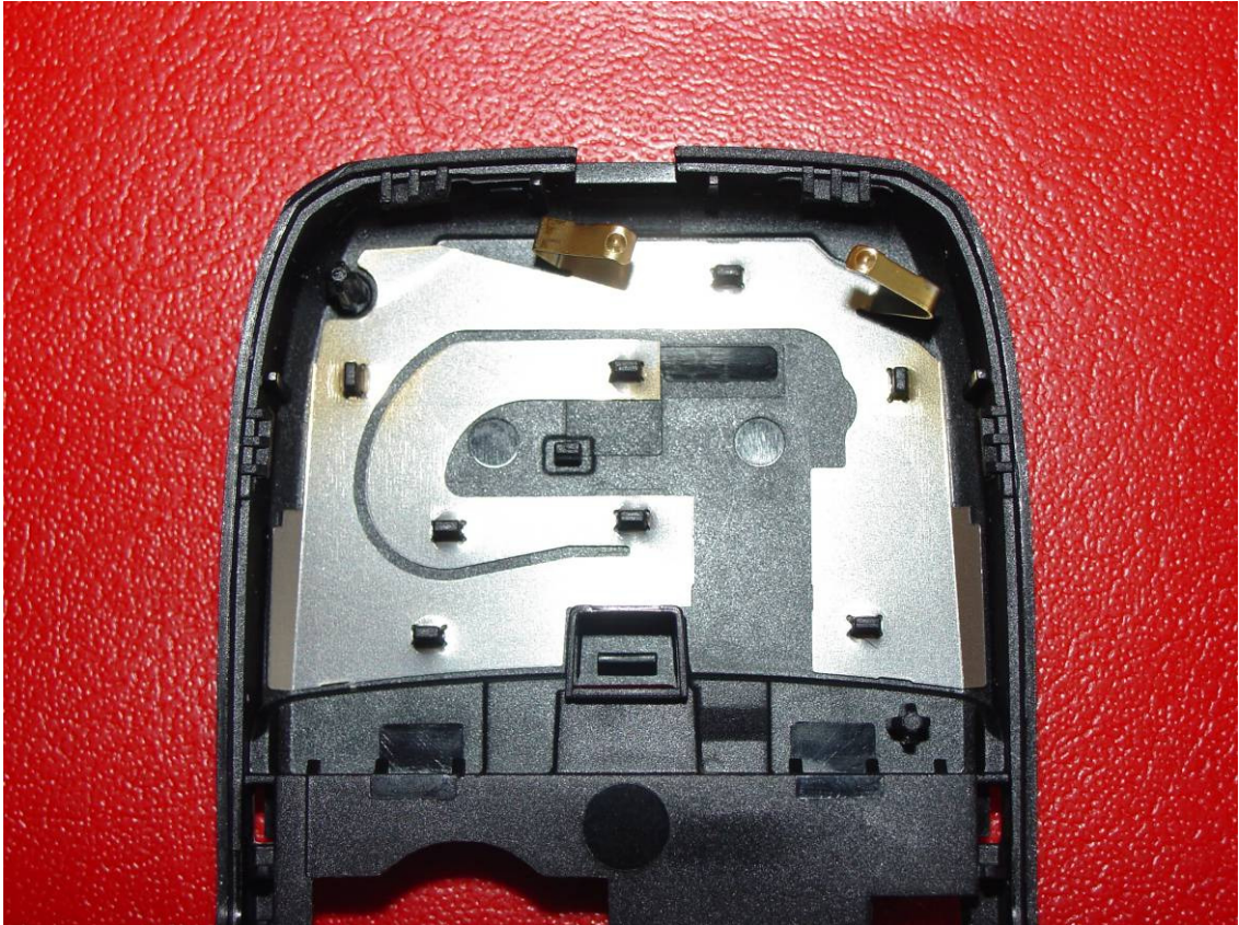
AX72 Tri-Band Antenna
