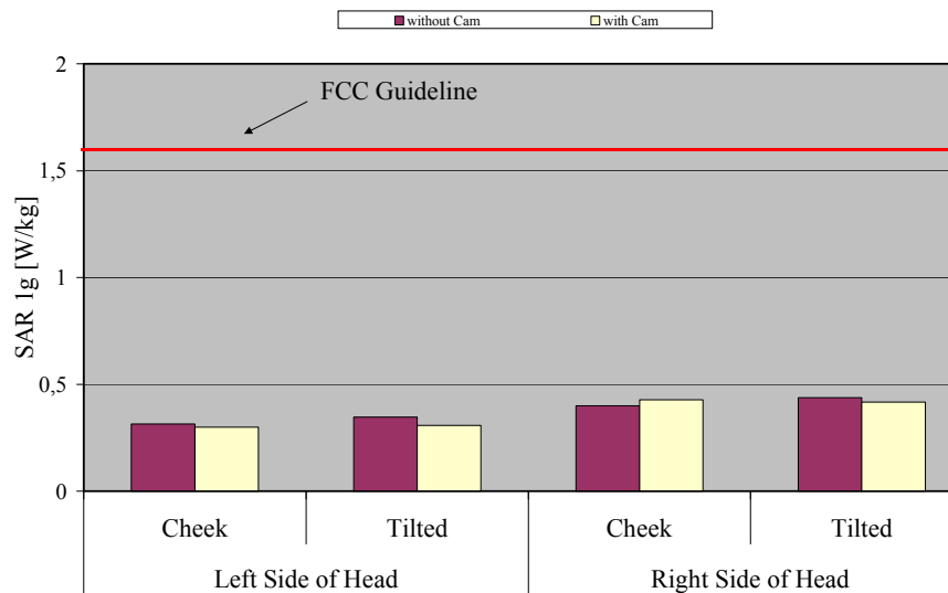
Fig. 8: The measured head phantom SAR values for the Siemens A65 without and with Cam for PCS 1900 in comparison to the FCC exposure limit.
