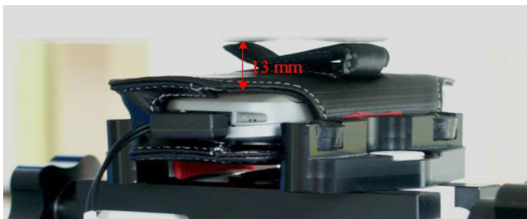
Fig. 27: Body worn configuration, GSM mode (1 TX slot) with headset, antenna towards the phantom and FCL 600 carry case.
