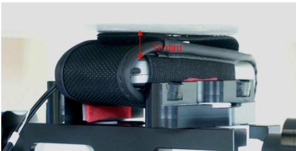
Fig. 26: Body worn configuration, GSM mode (1 TX slot) with headset, antenna towards the phantom and FCT 650 carry case.
