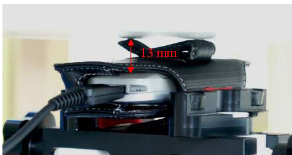
Fig. 28: Body worn configuration, GPRS mode (1 TX slot) with data cable, antenna towards the phantom and FCL 600 carry case.
