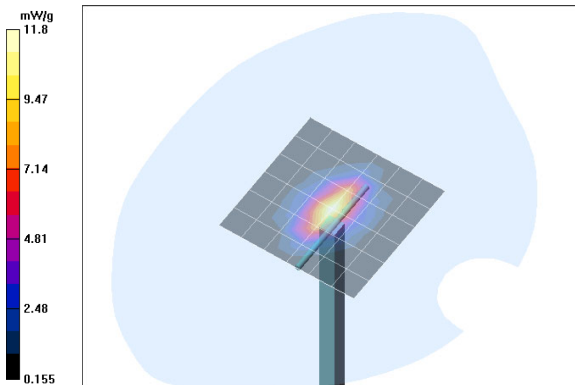
Fig. 11: Validation measurement 1900 MHz body (July 15, 2004), coarse grid. Ambient Temperature: 21.1° C, Liquid Temperature: 20.6° C.
