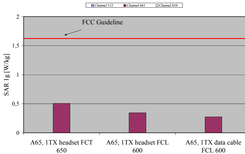
Fig. 9: The measured SAR values in body-worn configuration for the Siemens A65 for PCS 1900 in comparison to the FCC exposure limit.
