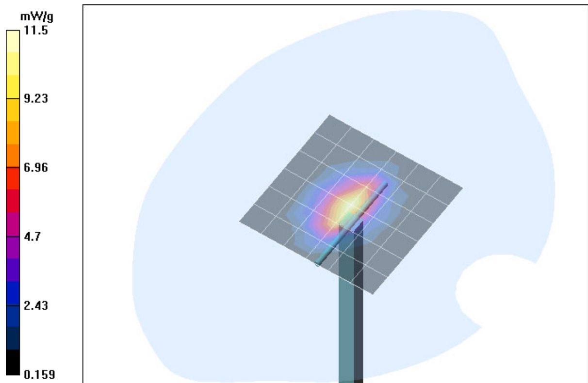
Fig. 10: Validation measurement 1900 MHz Head (July 23, 2004), coarse grid. Ambient Temperature: 21.0° C, Liquid Temperature: 20.5 C.
