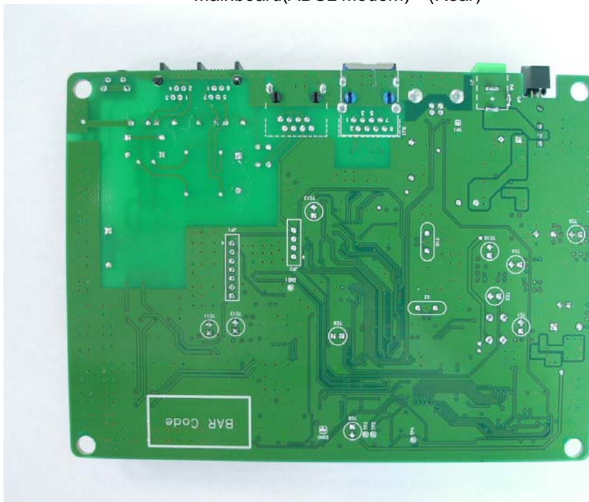
Mainboard(ADSL Modem) (Rear)
