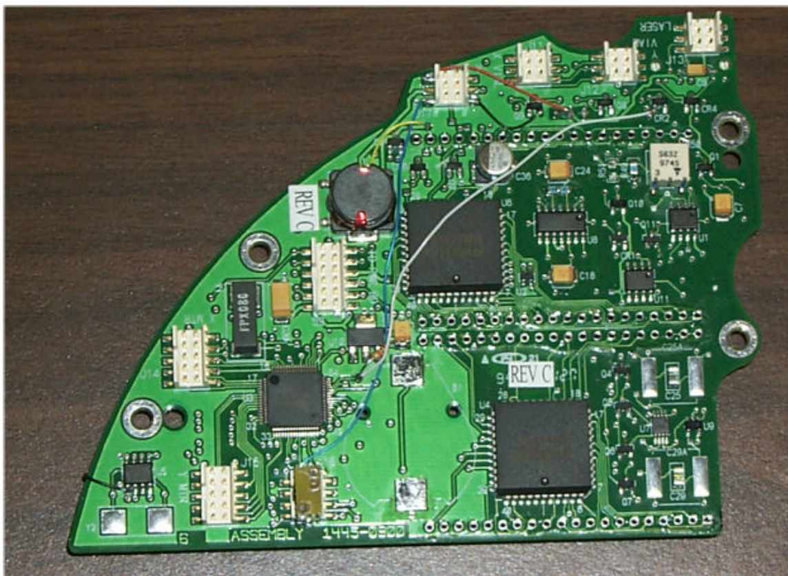
1445-0900 back with battery removed
