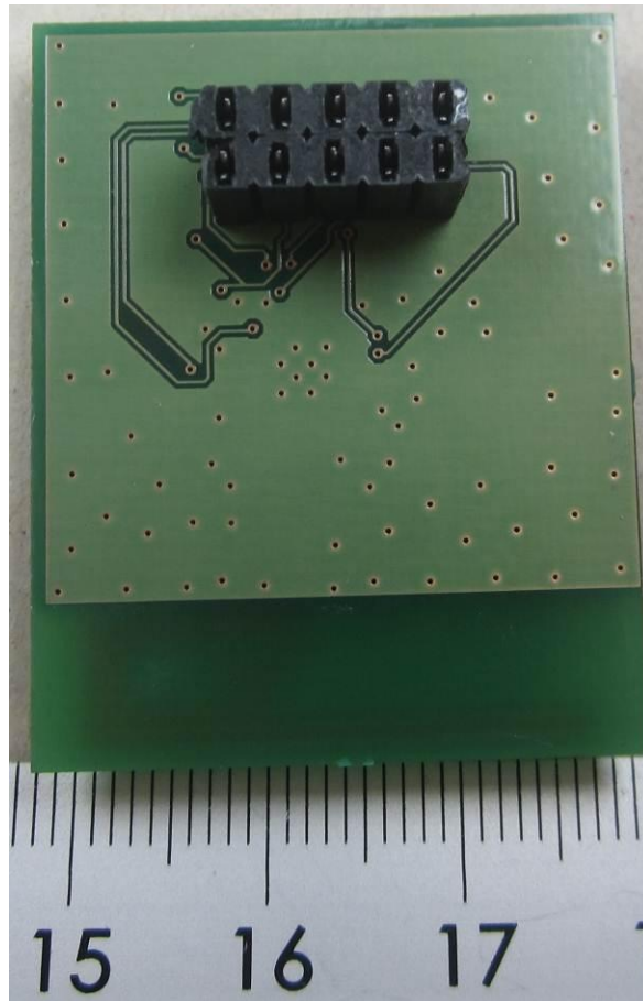
140852_09.JPG: EUT – bottom view
