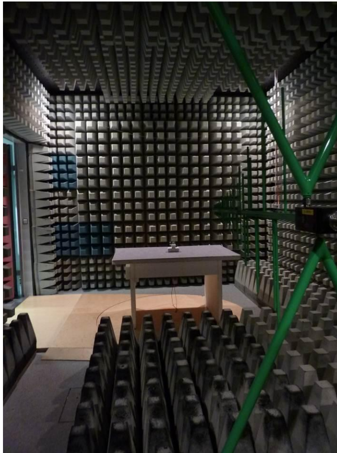
140852_02: Test setup - Radiated emission (fully anechoic chamber)
