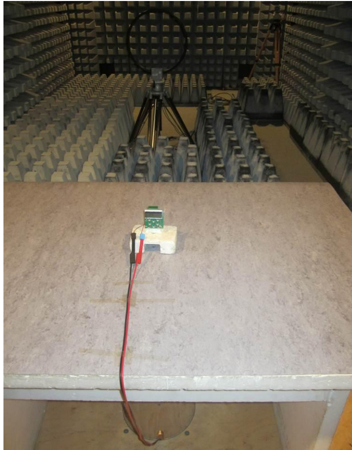
140852_01: Test setup - Radiated emission (fully anechoic chamber)
