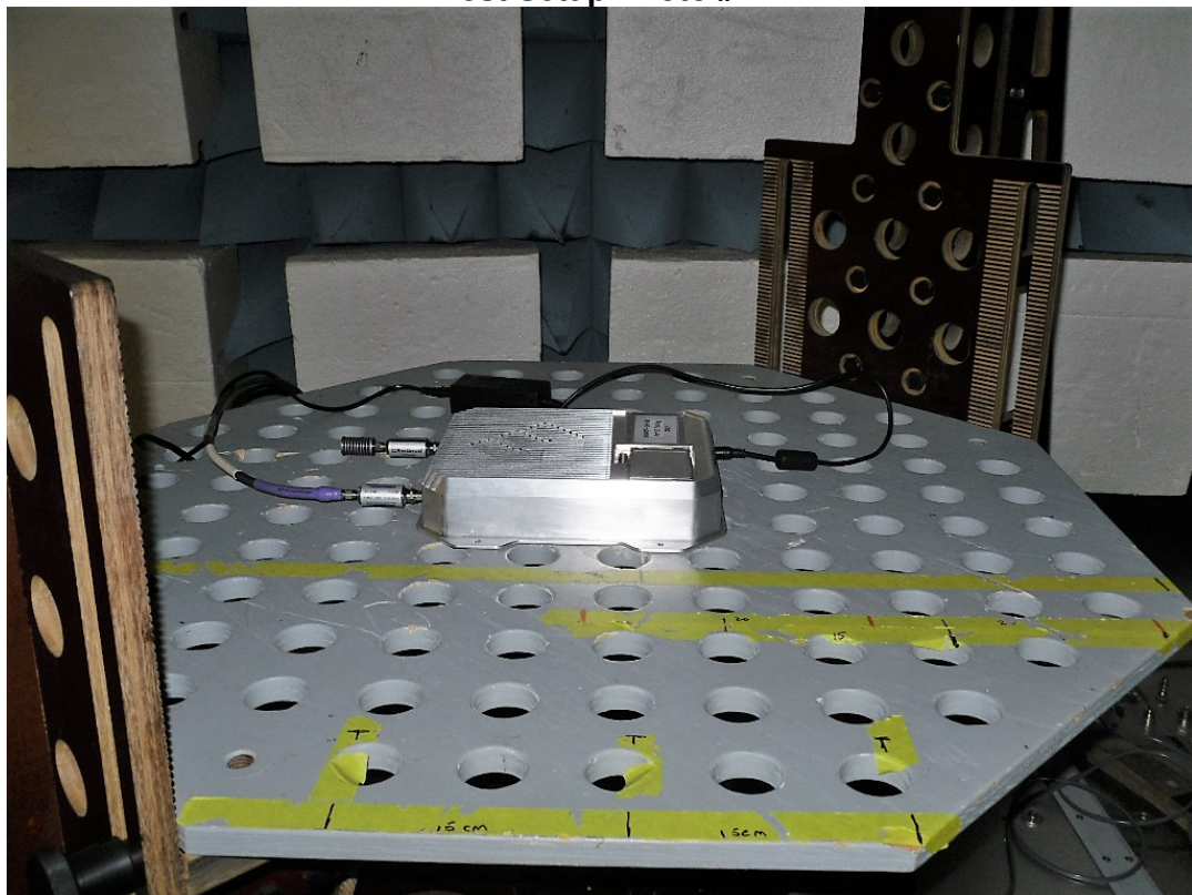
Test Setup Photo # 4
