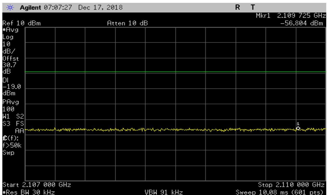
Plot 58 – 2110-2155MHz Band – GSM Downlink Lower Band Edge
