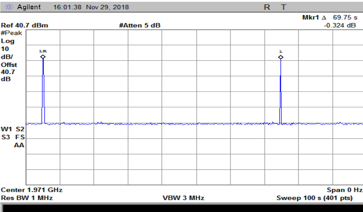
Plot 229 – 1930-1995MHz Band –Downlink Restart Time
