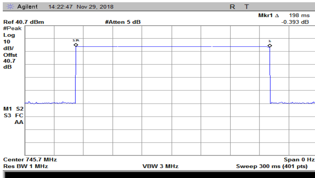
Plot 216 – 728-746MHz Band – Downlink Oscillation Detection Time
