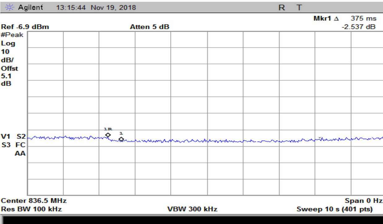
Plot 133 – 824-849MHz Band – Variable Uplink Noise Timing
