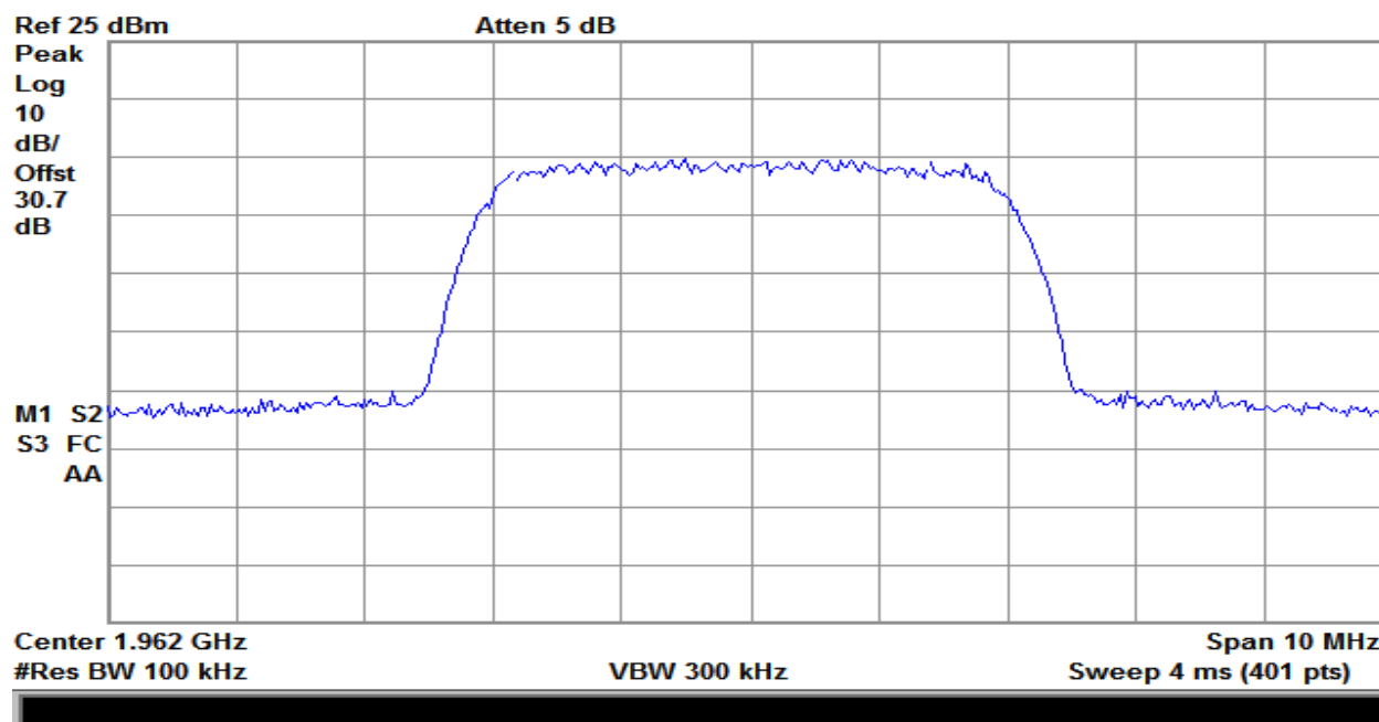
Plot 198 – 1930-1995MHz Band – Downlink Output – LTE
