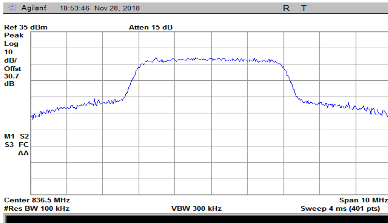
Plot 186 – 824-849MHz Band – Uplink Output – LTE
