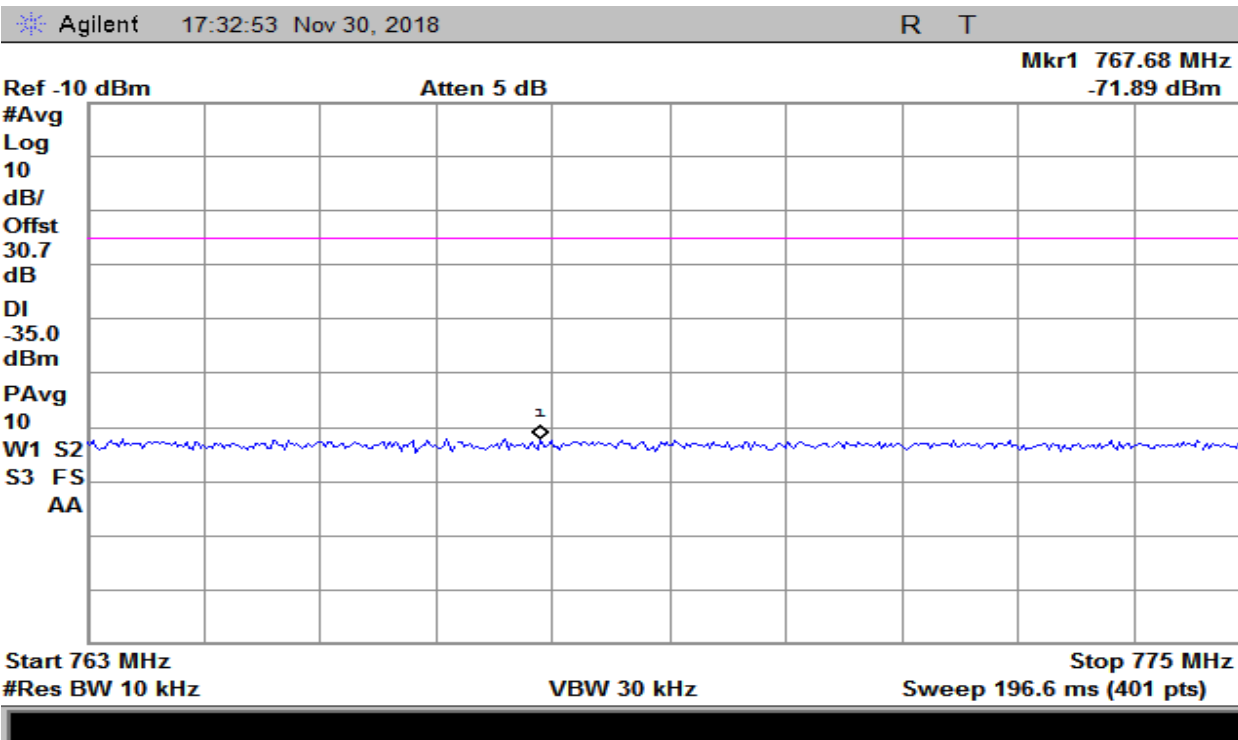
Plot 120 -27.53c4 – Downlink
