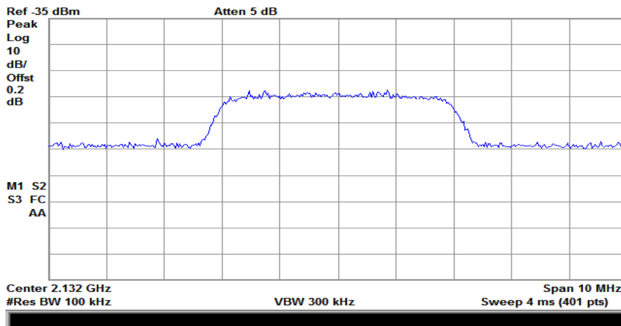
Plot 199 – 2110-2155MHz Band – Downlink Input – LTE
