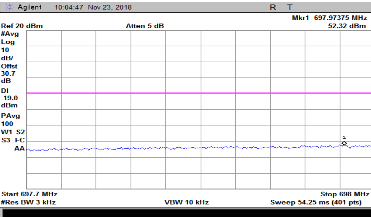
Plot 30 – 698-716MHz Band – CDMA Uplink Lower Band Edge
