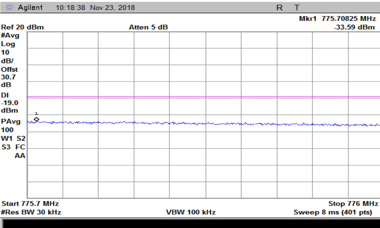
Plot 32 – 776-787MHz Band – CDMA Uplink Lower Band Edge
