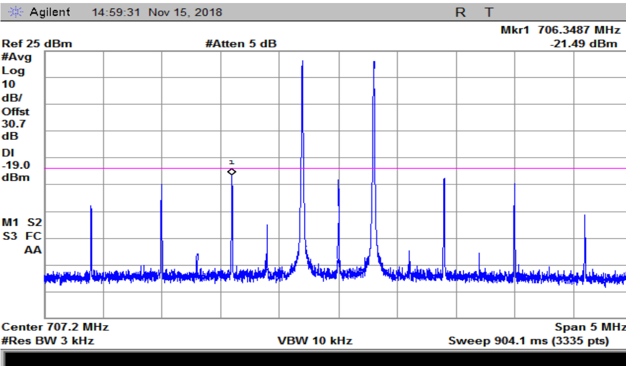
Plot 11 698-716MHz Band – Uplink
