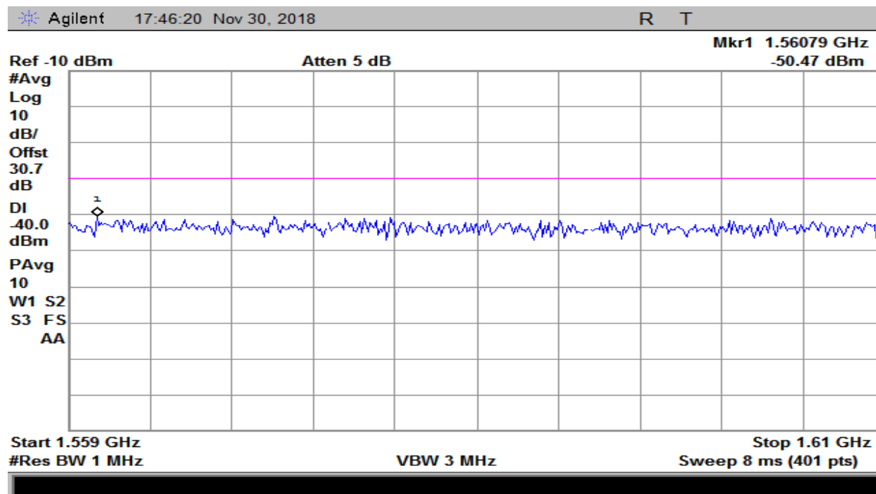
Plot 119 -27.53f – Downlink Wideband
