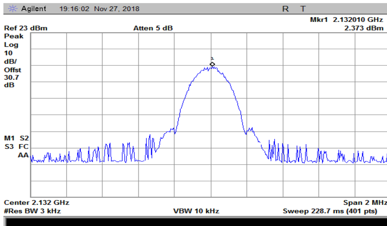
Plot 160 – 2110-2155MHz Band – Downlink Output – GSM
