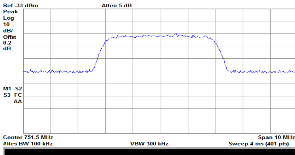
Plot 193 – 746-757MHz Band – Downlink Input – LTE
