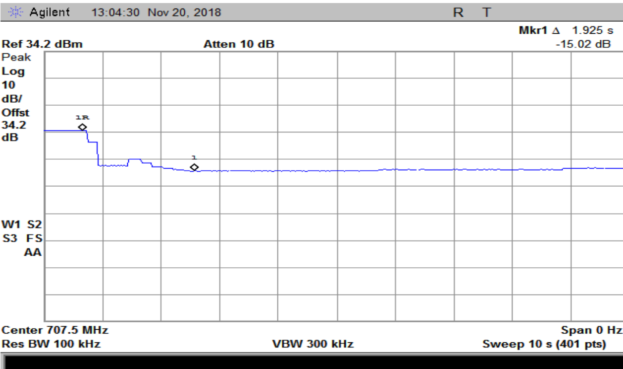
Plot 136 – 698-716MHz Band – Uplink Gain Timing
