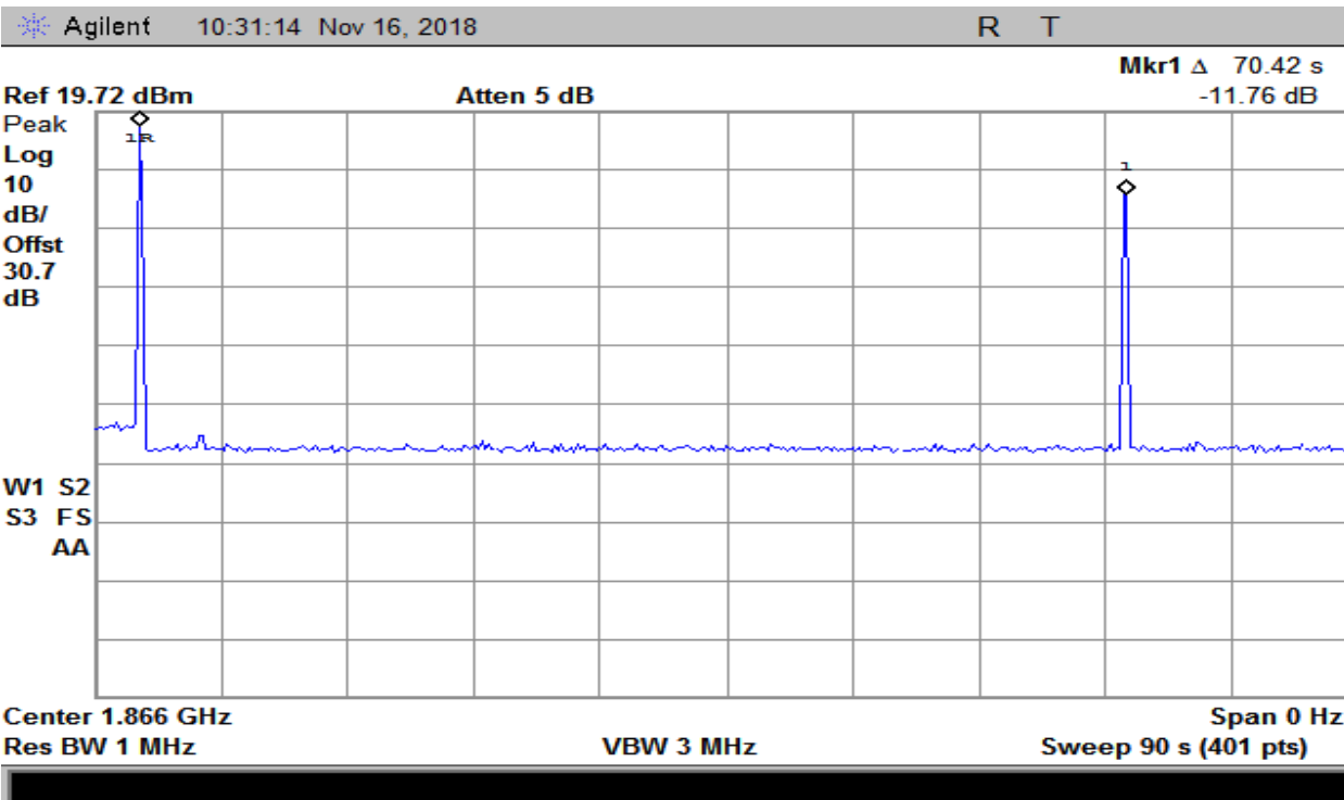
Plot 225 – 1850-1915MHz Band –Uplink Restart Time
