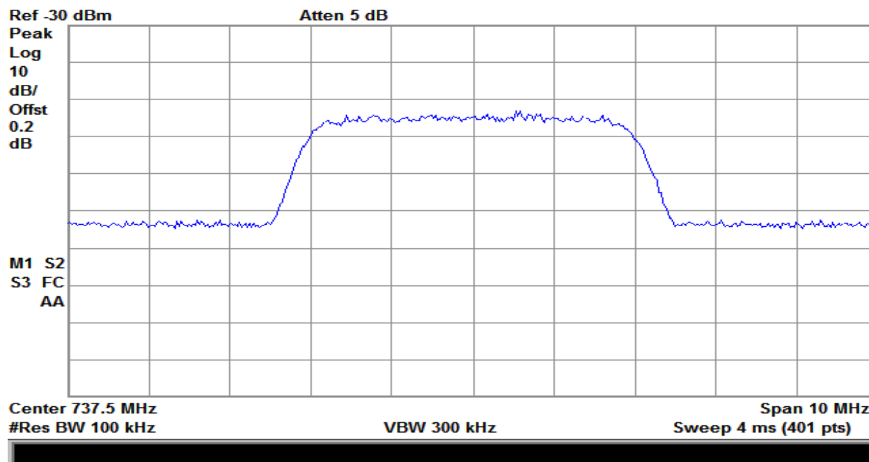
Plot 191 – 728-746MHz Band – Downlink Input – LTE
