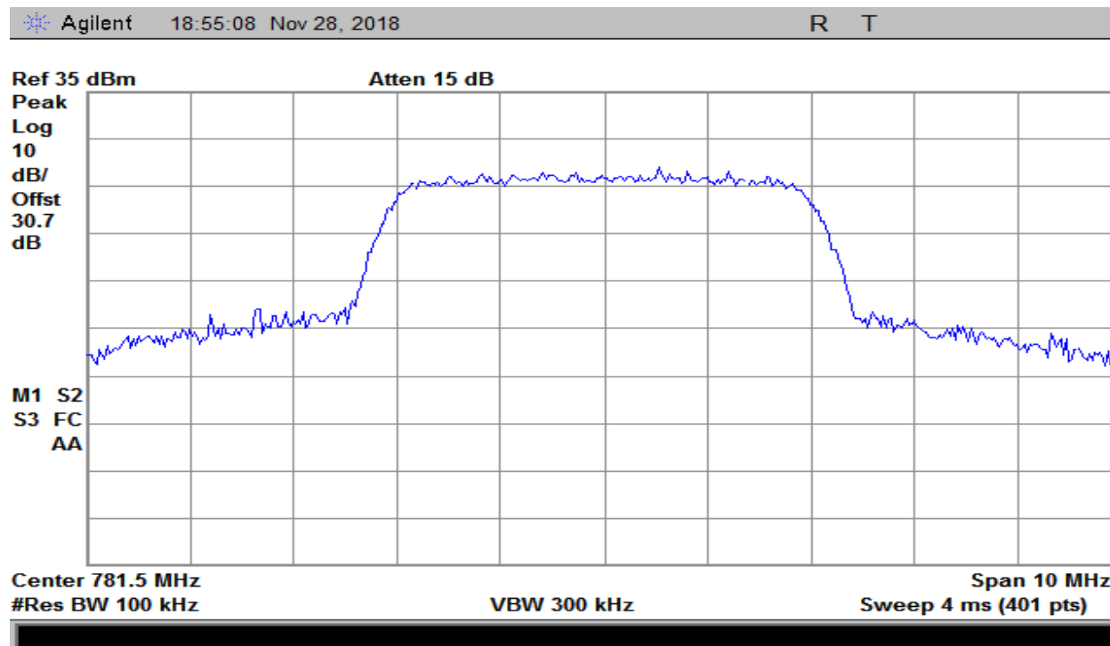
Plot 184 – 776-787MHz Band – Uplink Output – LTE
