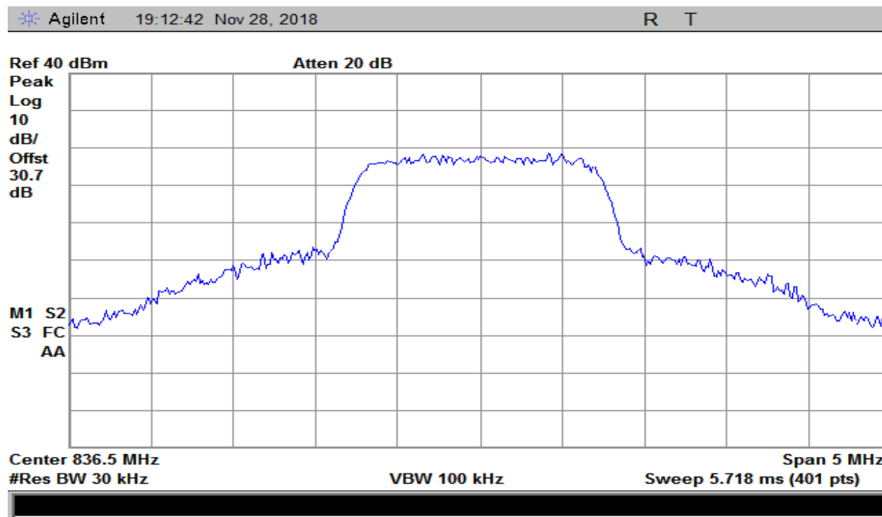
Plot 166 – 824-849MHz Band – Uplink Output – CDMA
