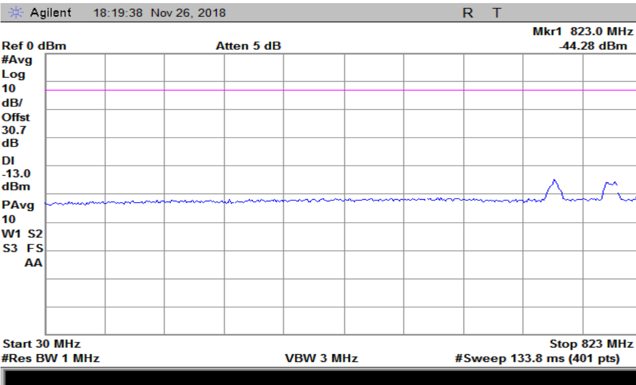
Plot 86 – 824-849MHz Band – Uplink
