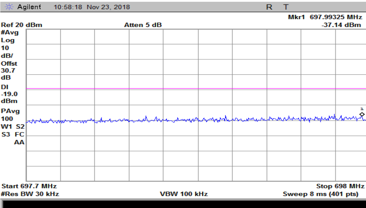
Plot 40 – 698-716MHz Band – LTE Uplink Lower Band Edge
