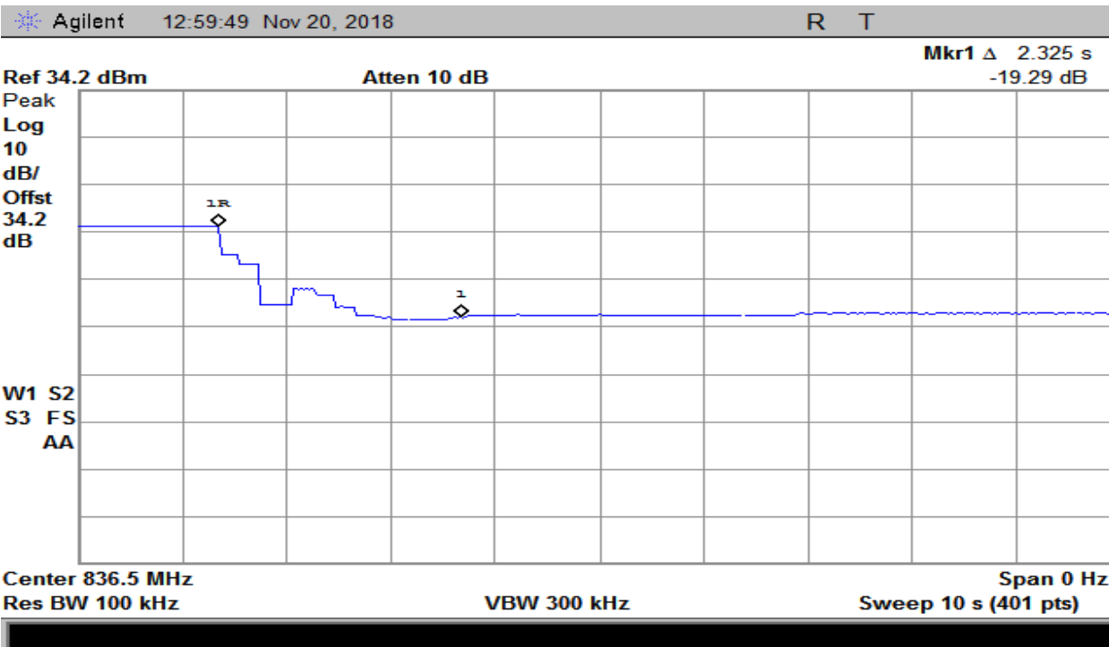
Plot 138 – 824-849MHz Band – Uplink Gain Timing
