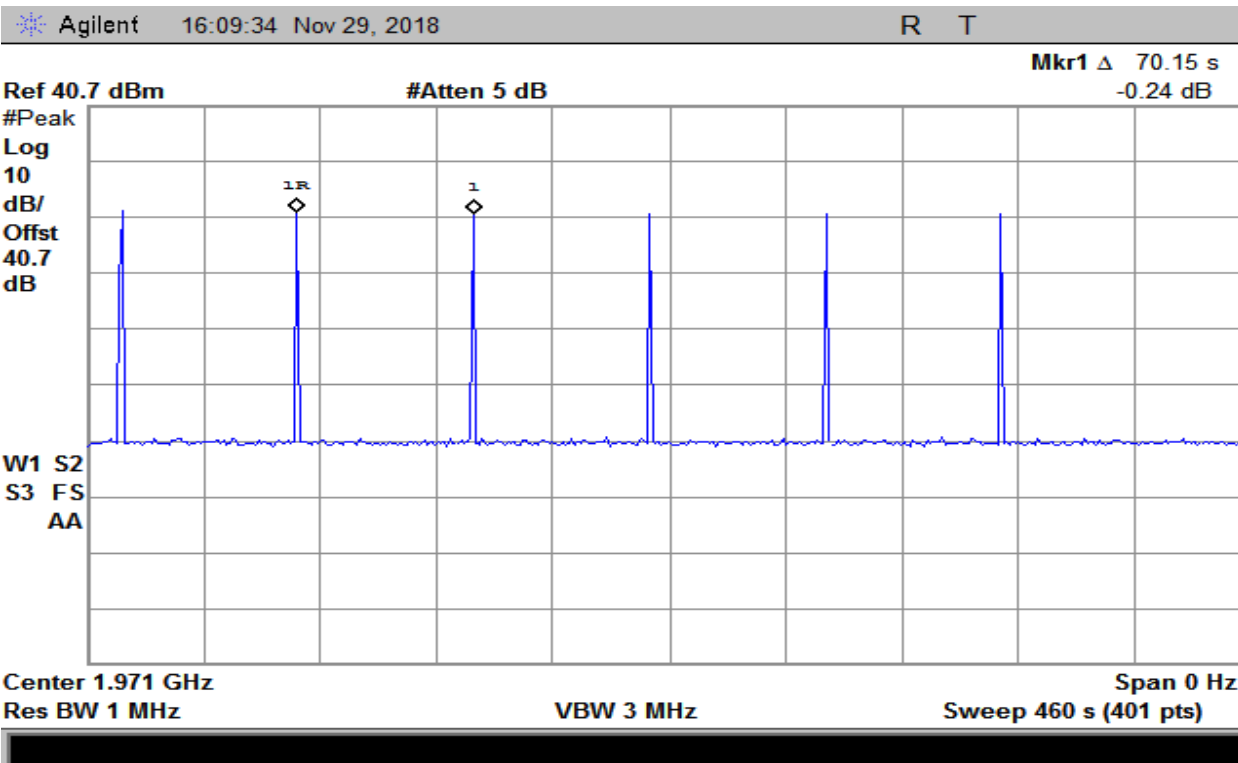
Plot 239 – 1930-1995MHz Band – Downlink # of Restart Time
