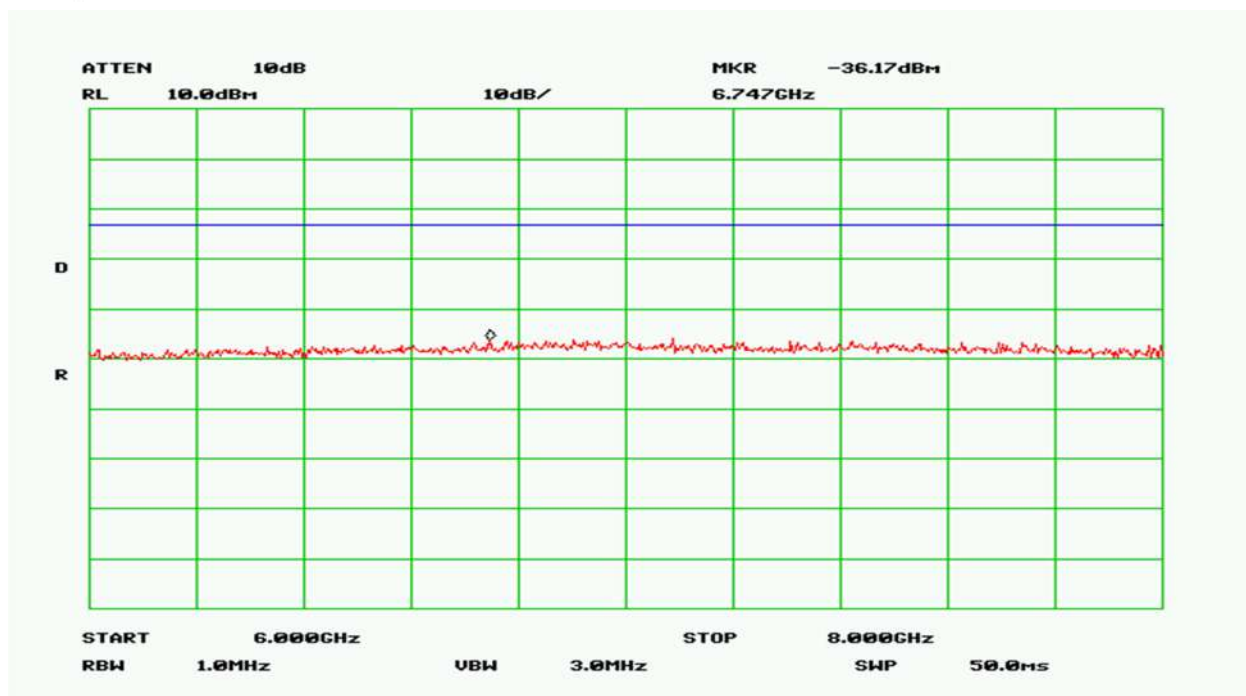
Plot 102 – 746-757MHz Band – Downlink
