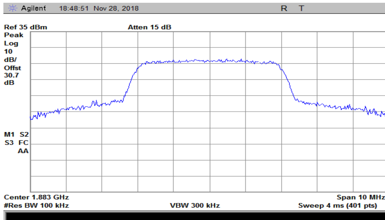
Plot 190 – 1850-1915MHz Band – Uplink Output – LTE
