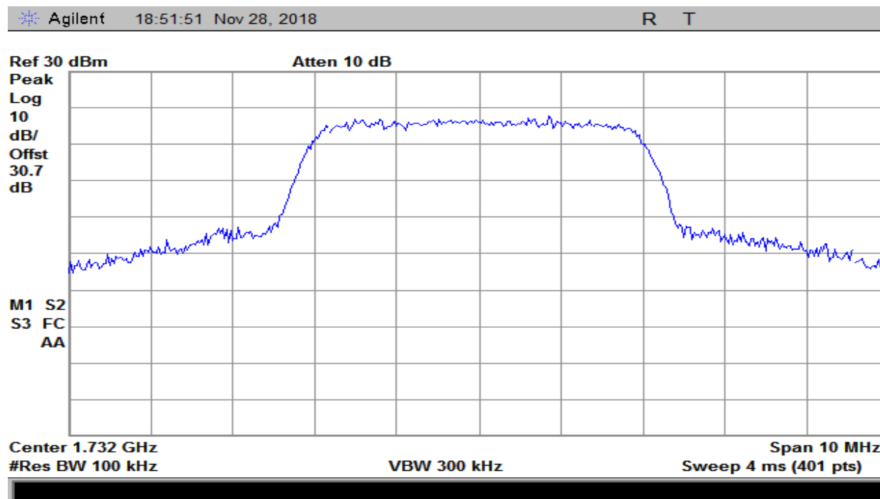
Plot 188 – 1710-1755MHz Band – Uplink Output – LTE
