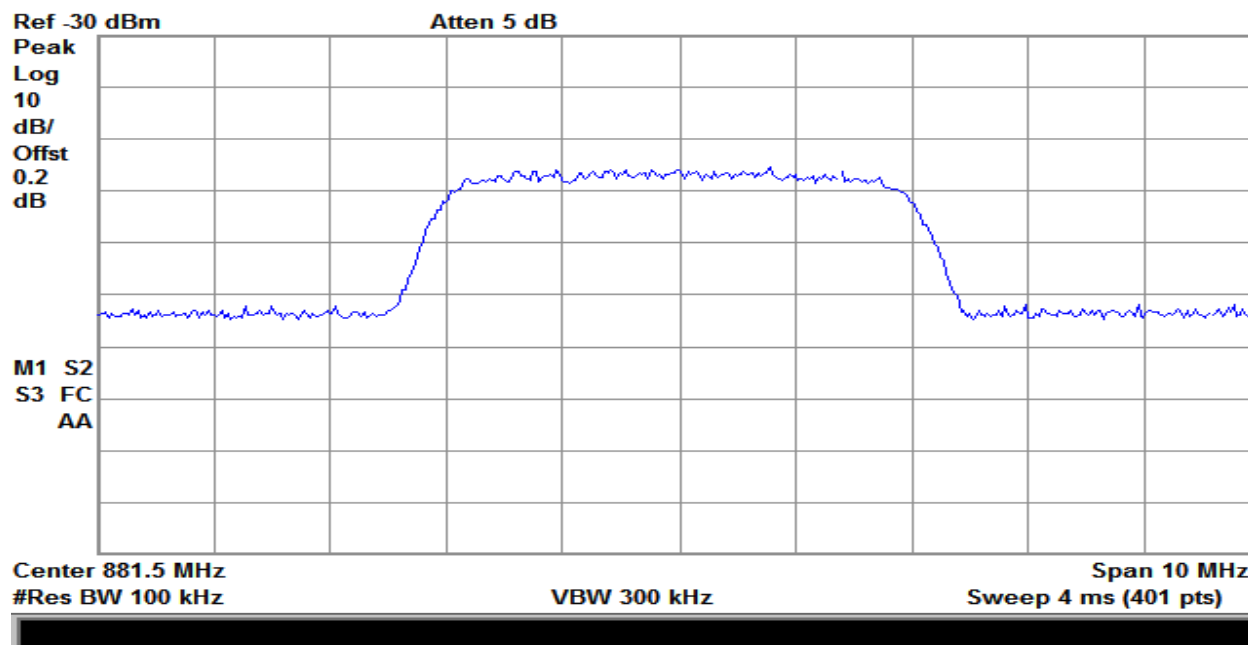
Plot 195 – 869-894MHz Band – Downlink Input – LTE
