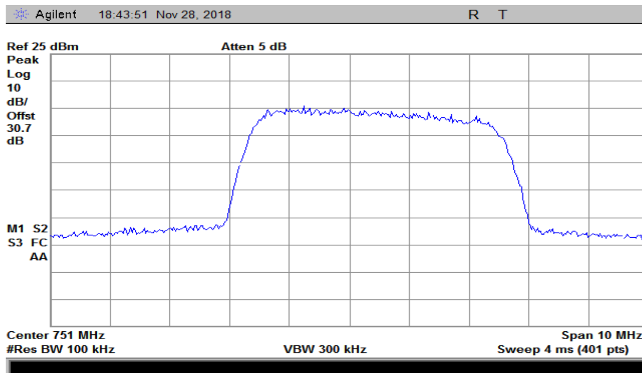
Plot 194 – 746-757MHz Band – Downlink Output – LTE
