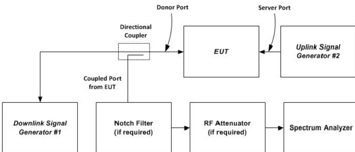
Figure 4 – Variable Gain
