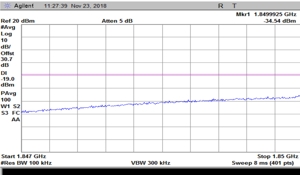
Plot 48 – 1850-1915MHz Band – LTE Uplink Lower Band Edge
