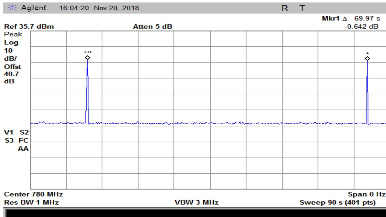
Plot 222 – 776-787MHz Band –Uplink Restart Time
