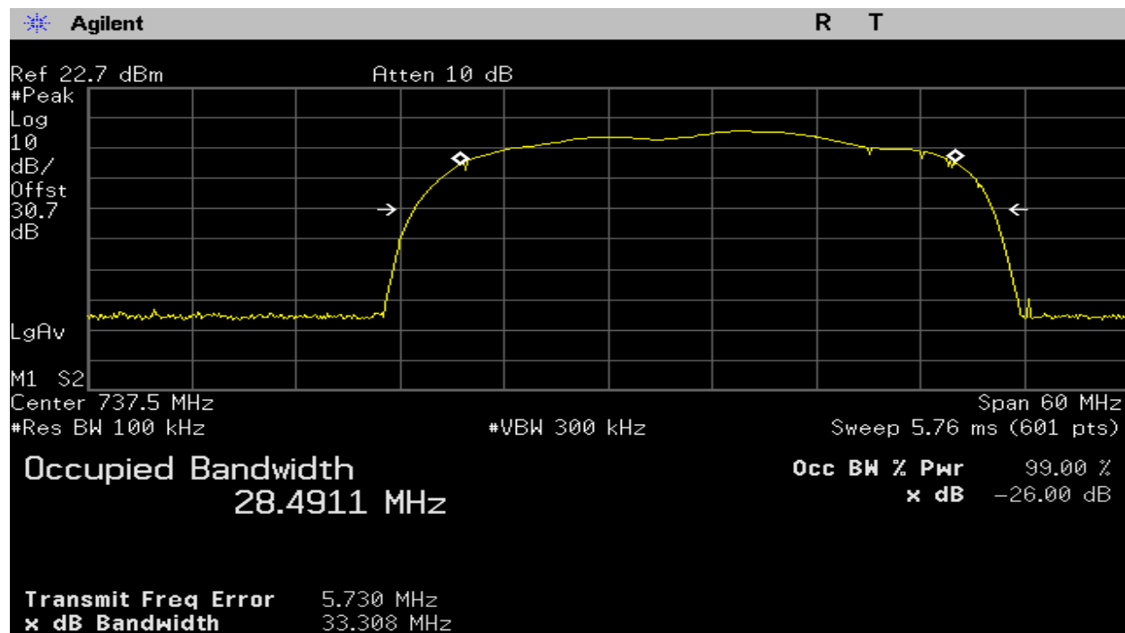
Plot 206 – 728-746MHz Band – Downlink – 99% BW for ISED (Canada)
