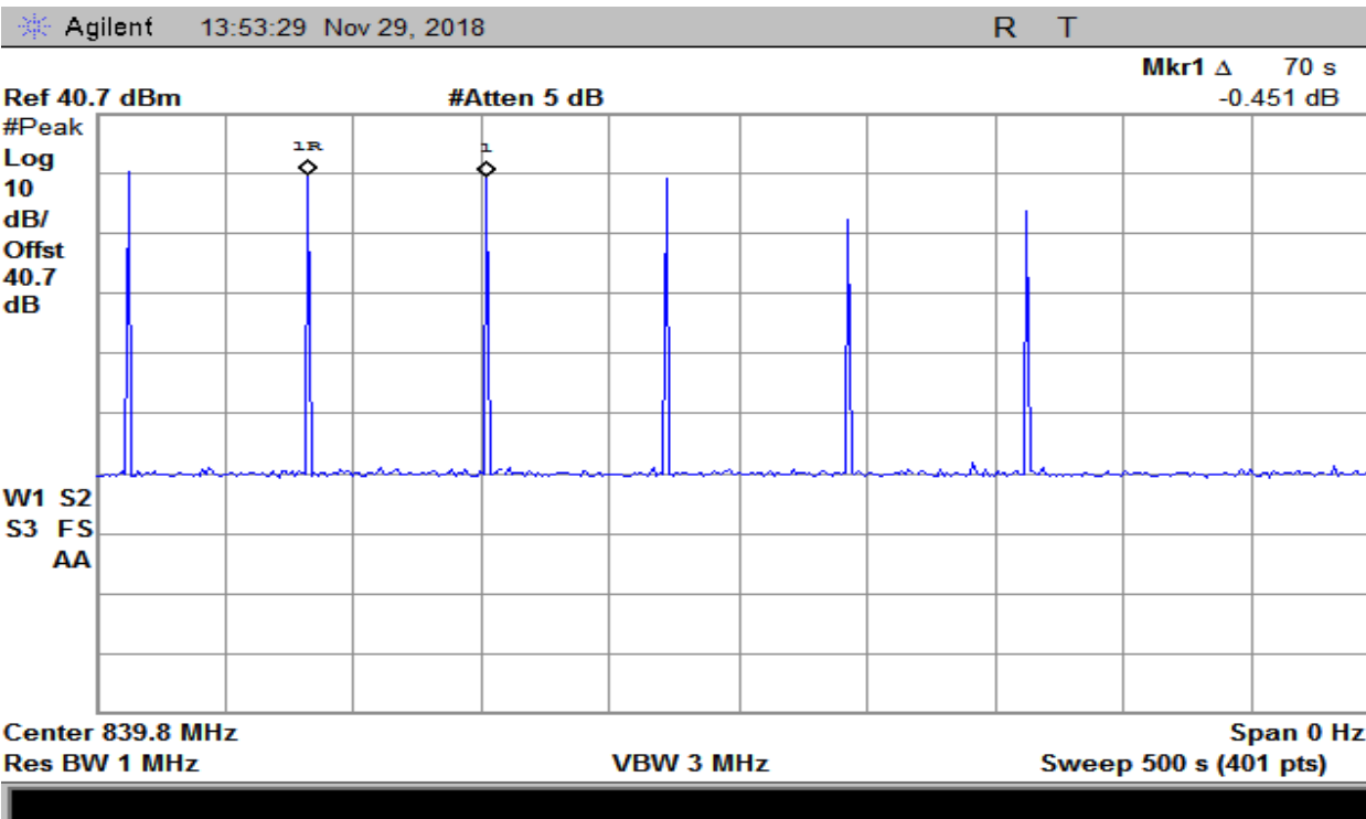
Plot 233 – 824-849MHz Band – Uplink # of Restart Time
