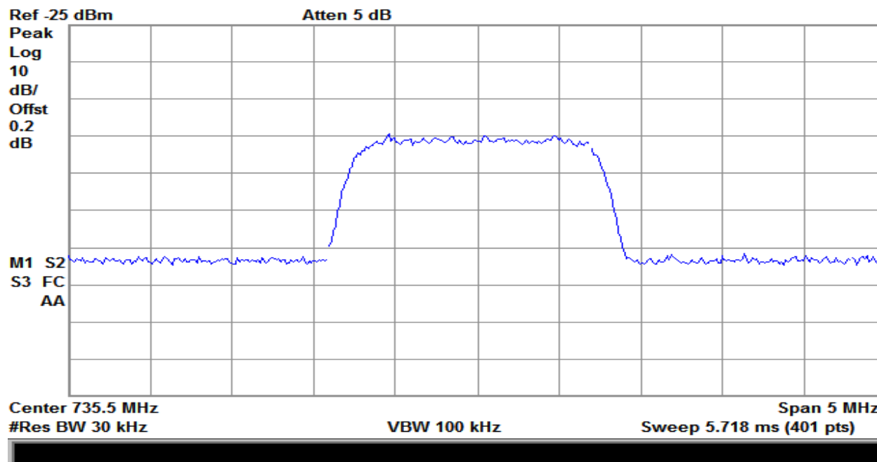
Plot 171 – 728-746MHz Band – Downlink Input – CDMA
