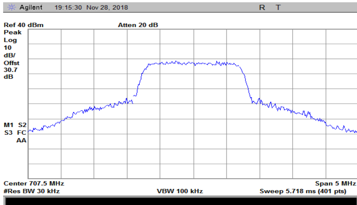
Plot 162 – 698-716MHz Band – Uplink Output – CDMA
