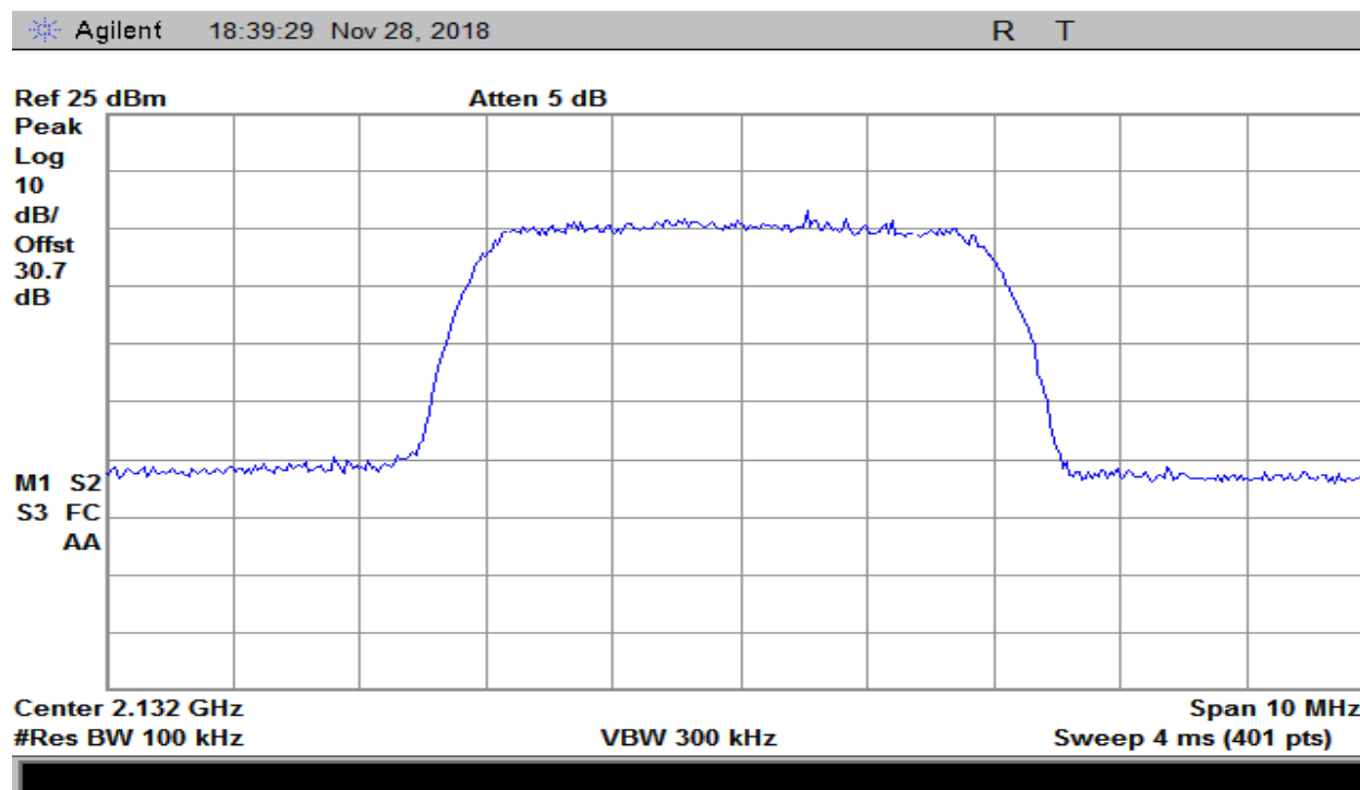
Plot 200 – 2110-2155MHz Band – Downlink Output – LTE
