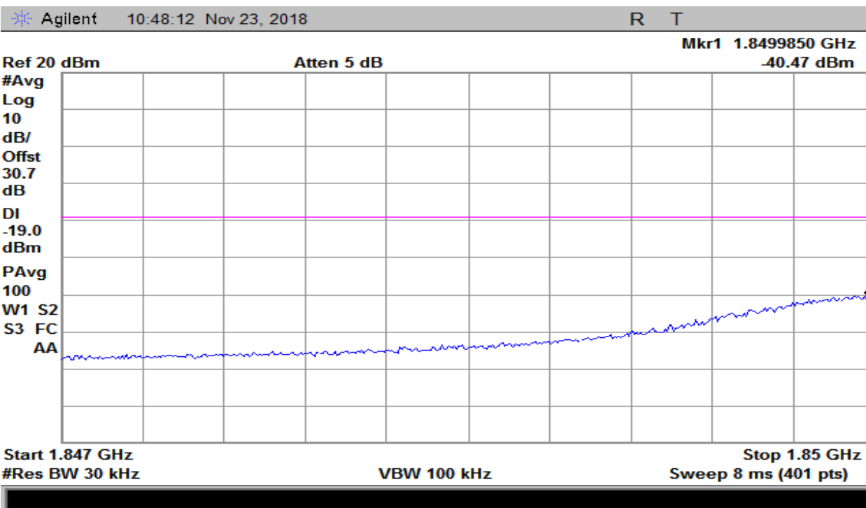
Plot 38 – 1850-1915MHz Band – CDMA Uplink Lower Band Edge
