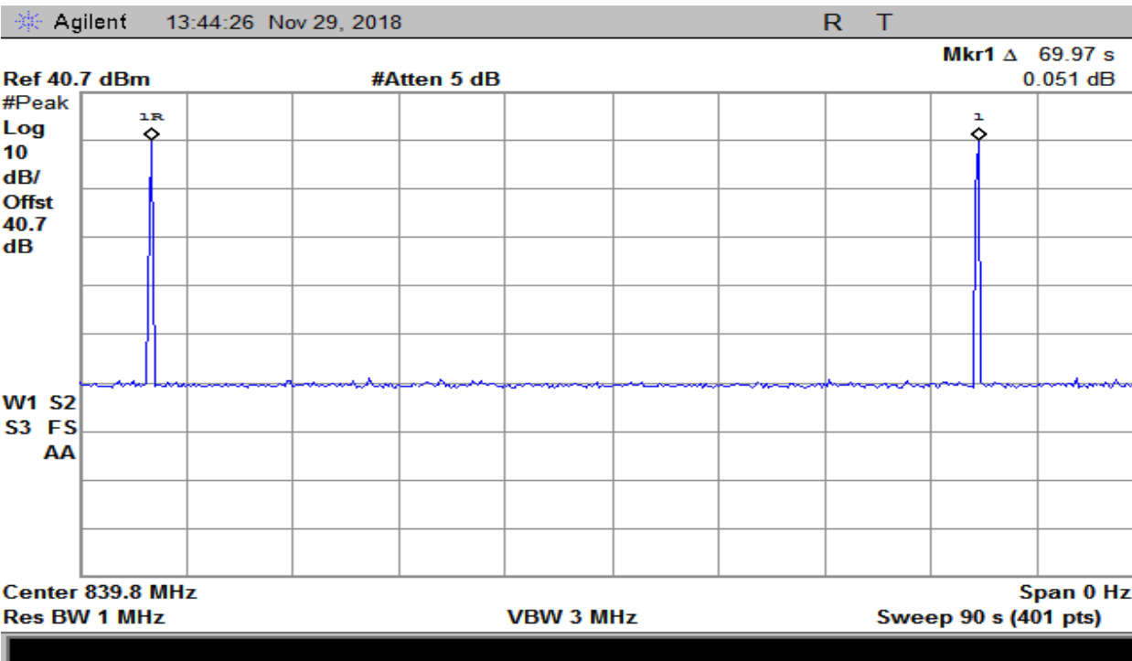
Plot 223 – 824-849MHz Band –Uplink Restart Time
