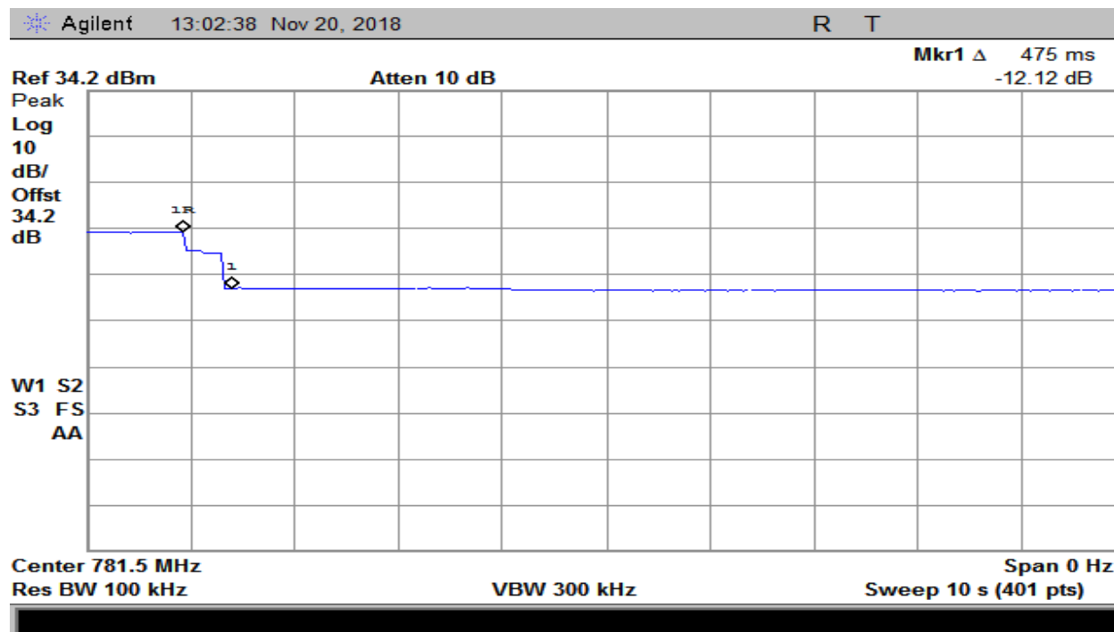
Plot 137 – 776-787MHz Band – Uplink Gain Timing
