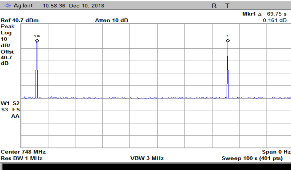
Plot 227 – 746-757MHz Band –Downlink Restart Time
