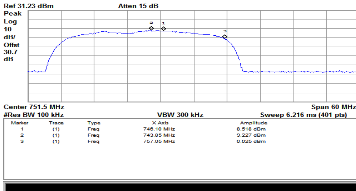
Plot 7 – 746-757MHz Band – Downlink
