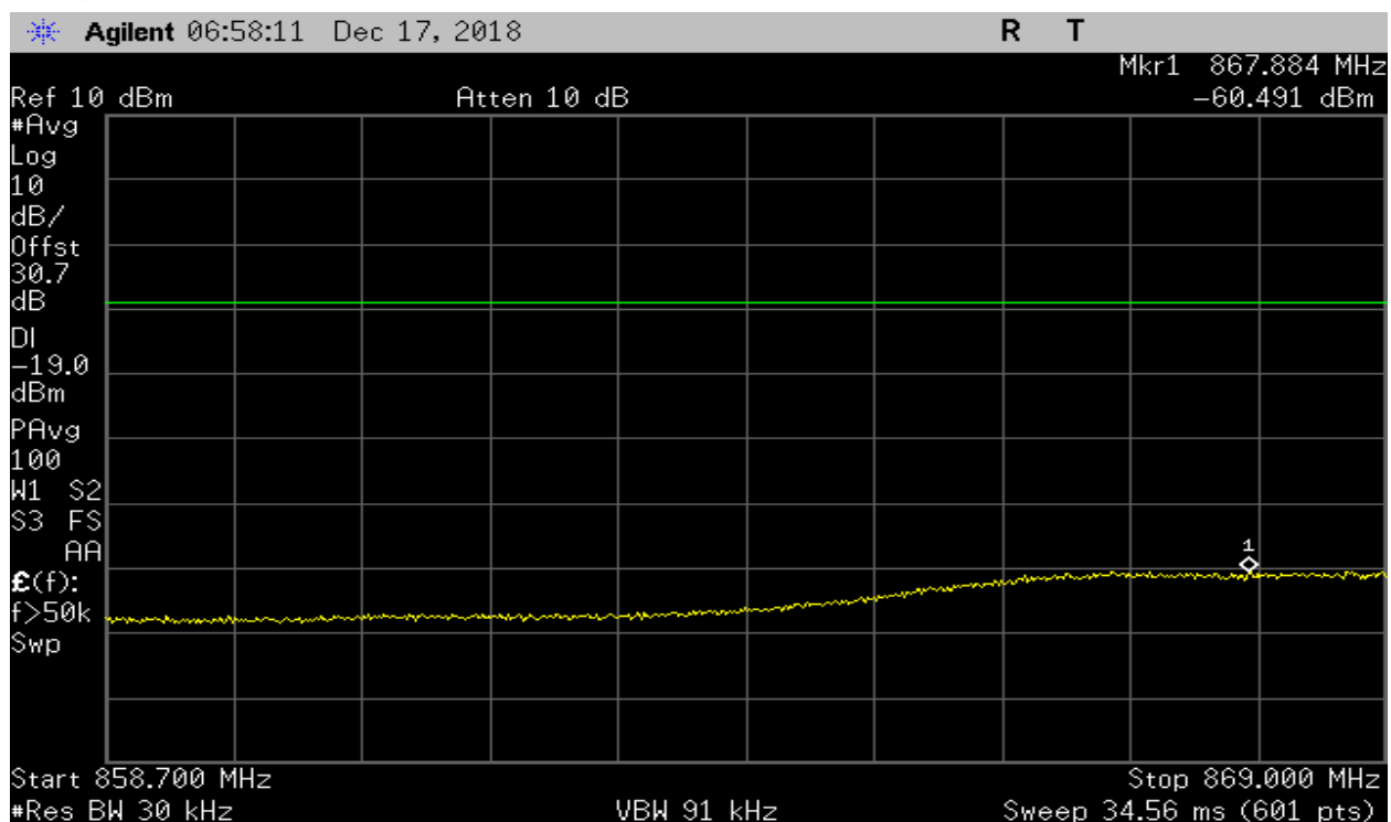
Plot 54 – 869-894MHz Band – GSM Downlink Lower Band Edge
