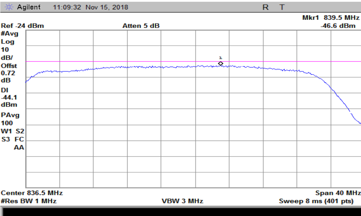
Plot 123 – 824-849MHz Band – Maximum Uplink Noise
