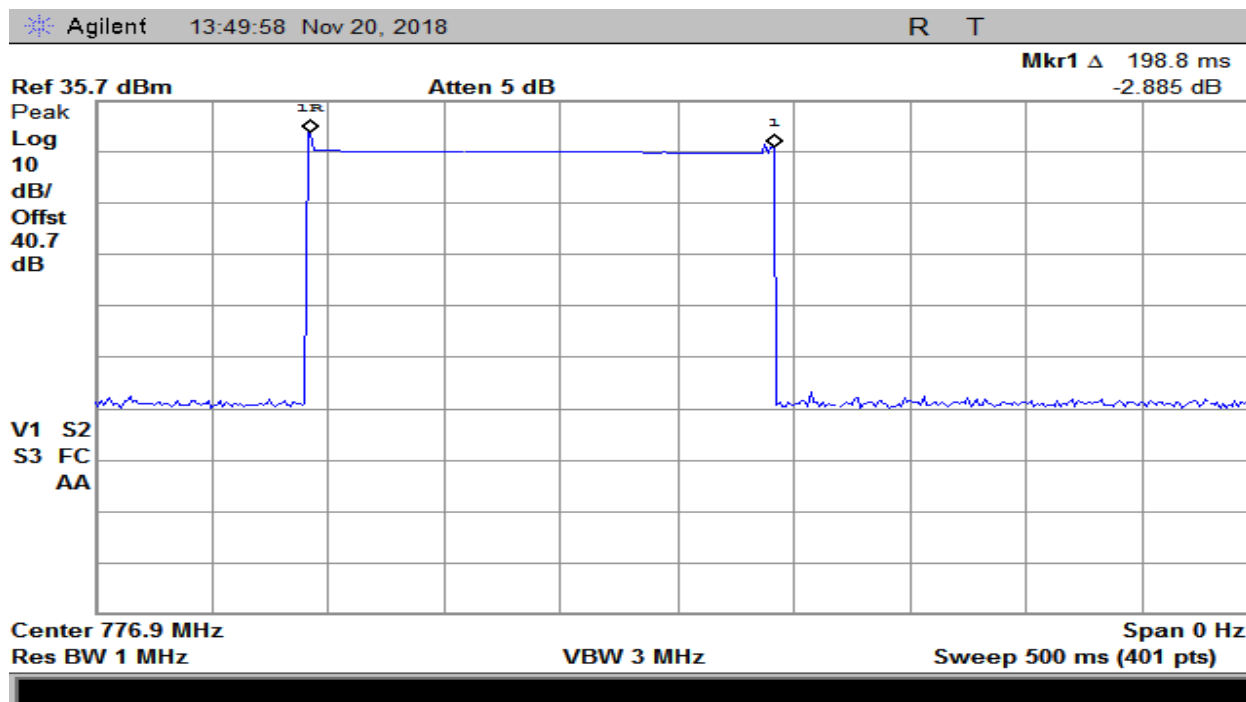
Plot 212 – 776-787MHz Band – Uplink Oscillation Detection Time
