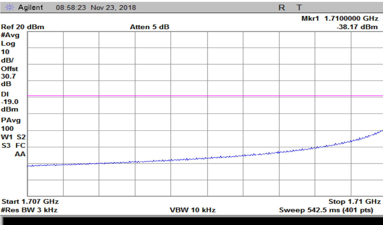
Plot 26 – 1710-1755MHz Band – GSM Uplink Lower Band Edge
