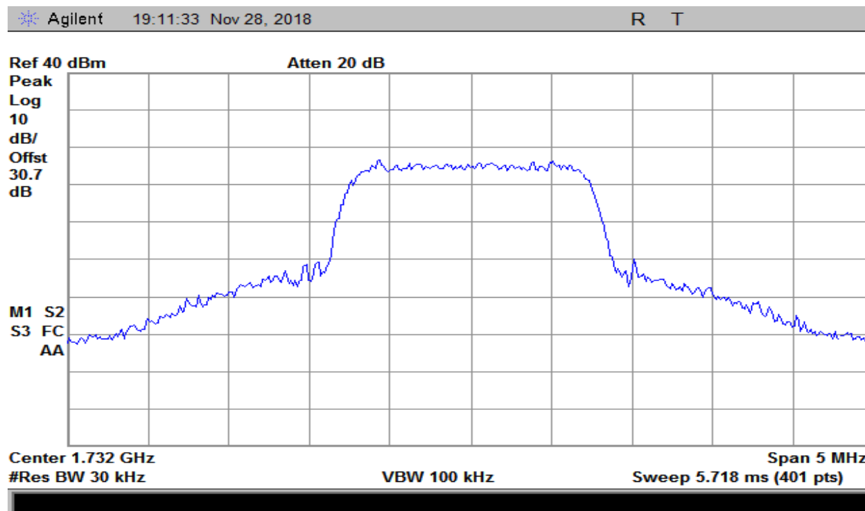
Plot 168 – 1710-1755MHz Band – Uplink Output – CDMA
