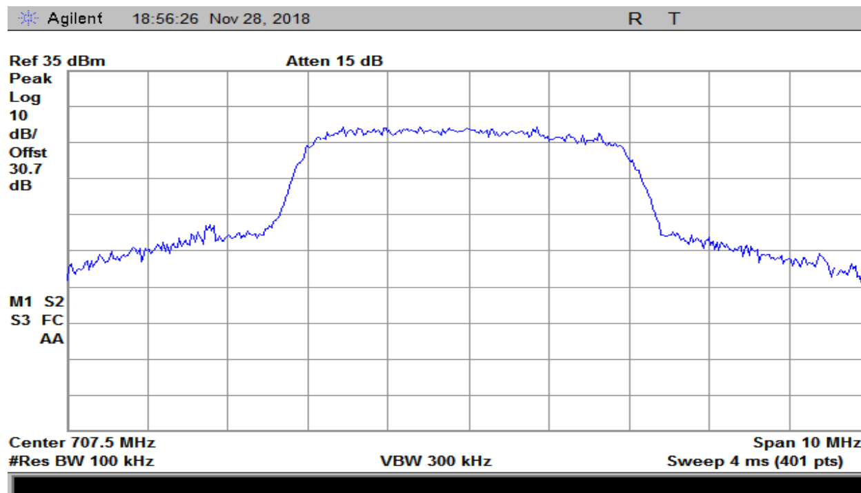
Plot 182 – 698-716MHz Band – Uplink Output – LTE
