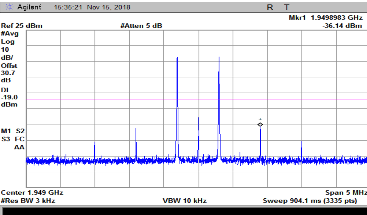
Plot 19 – 1930-1995MHz Band – Downlink
