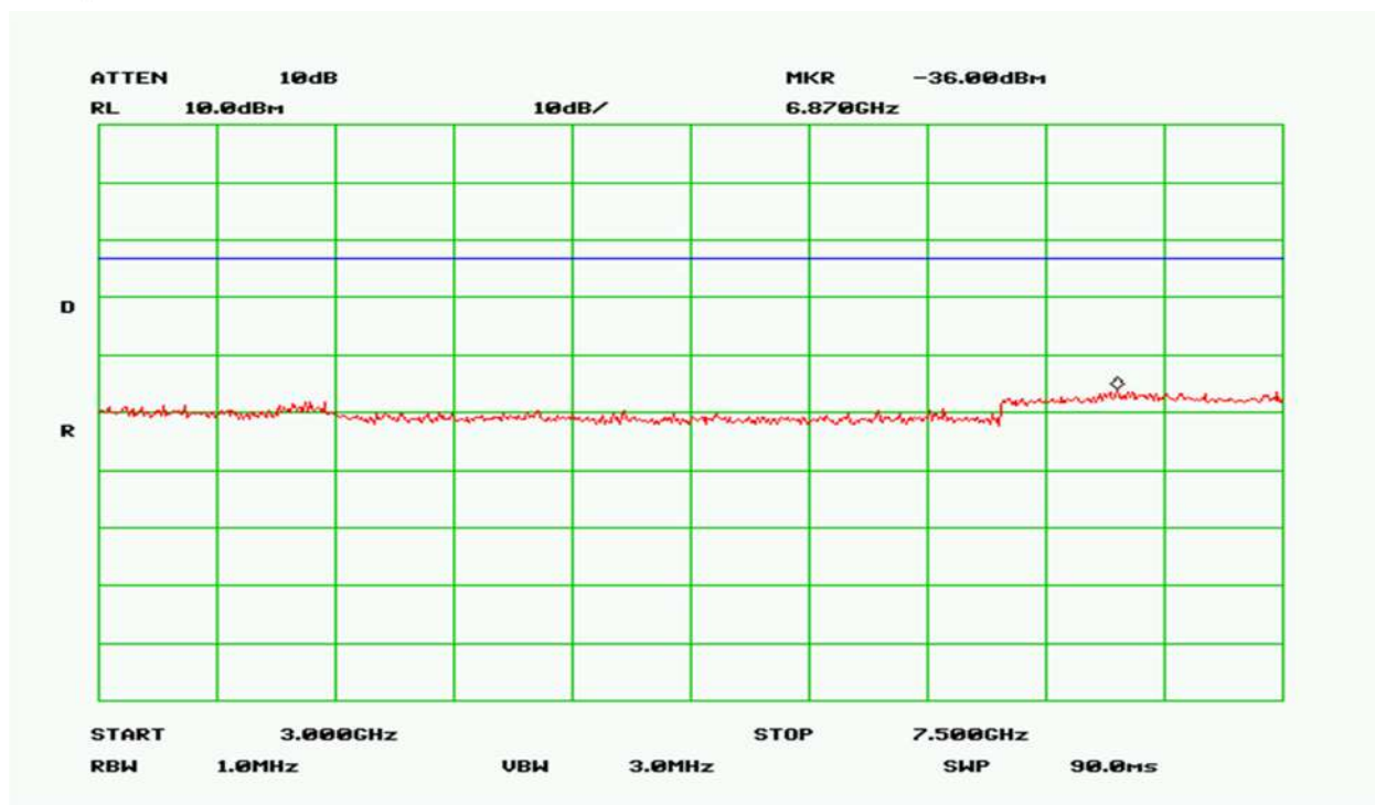
Plot 82 – 698-716MHz Band – Uplink
