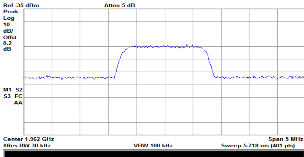
Plot 177 – 1930-1995MHz Band – Downlink Input – CDMA
