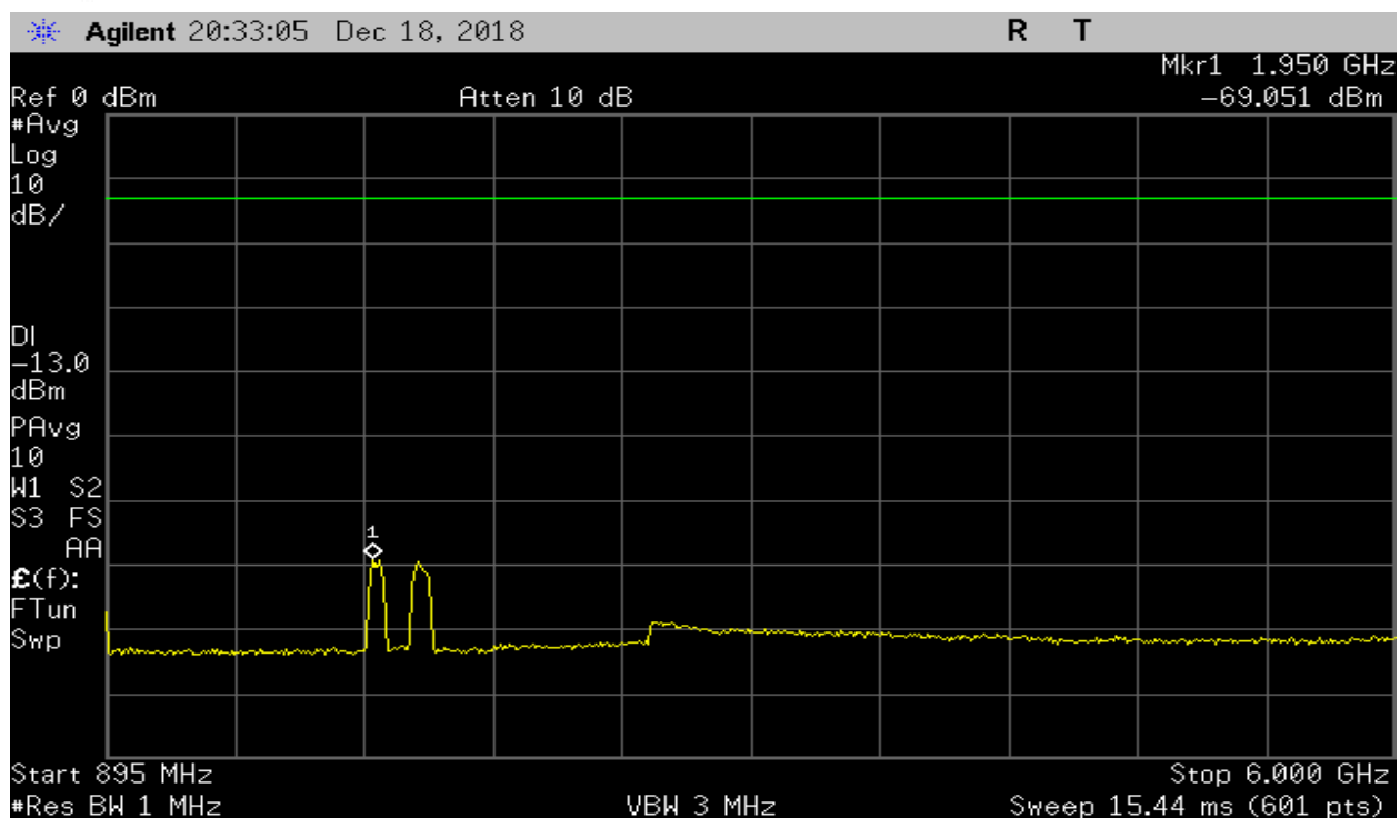
Plot 104 – 869-894MHz Band – Downlink
