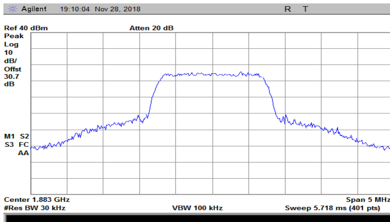
Plot 170 – 1850-1915MHz Band – Uplink Output – CDMA
