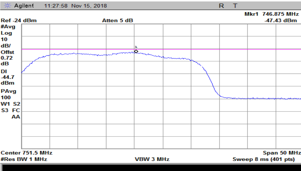
Plot 127 – 746-757MHz Band – Maximum Downlink Noise
