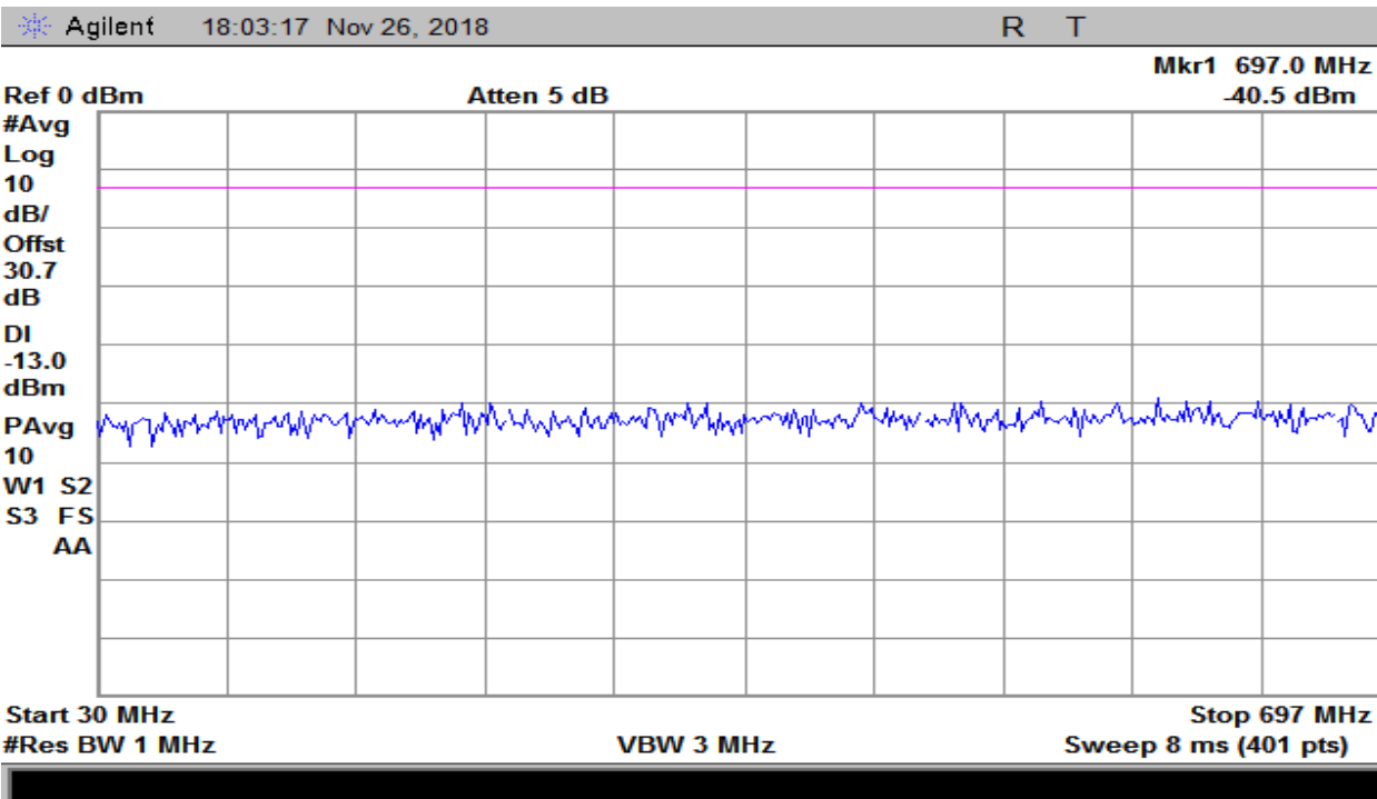
Plot 80 – 698-716MHz Band – Uplink
