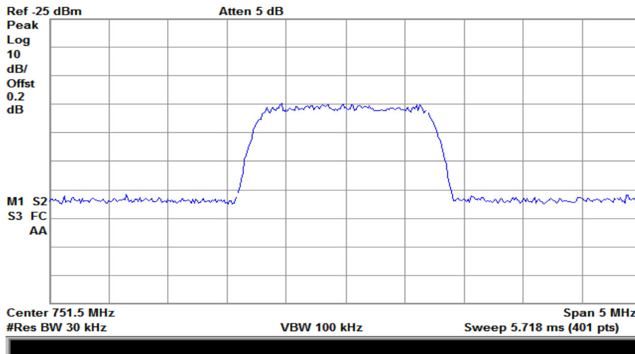
Plot 173 – 746-757MHz Band – Downlink Input – CDMA
