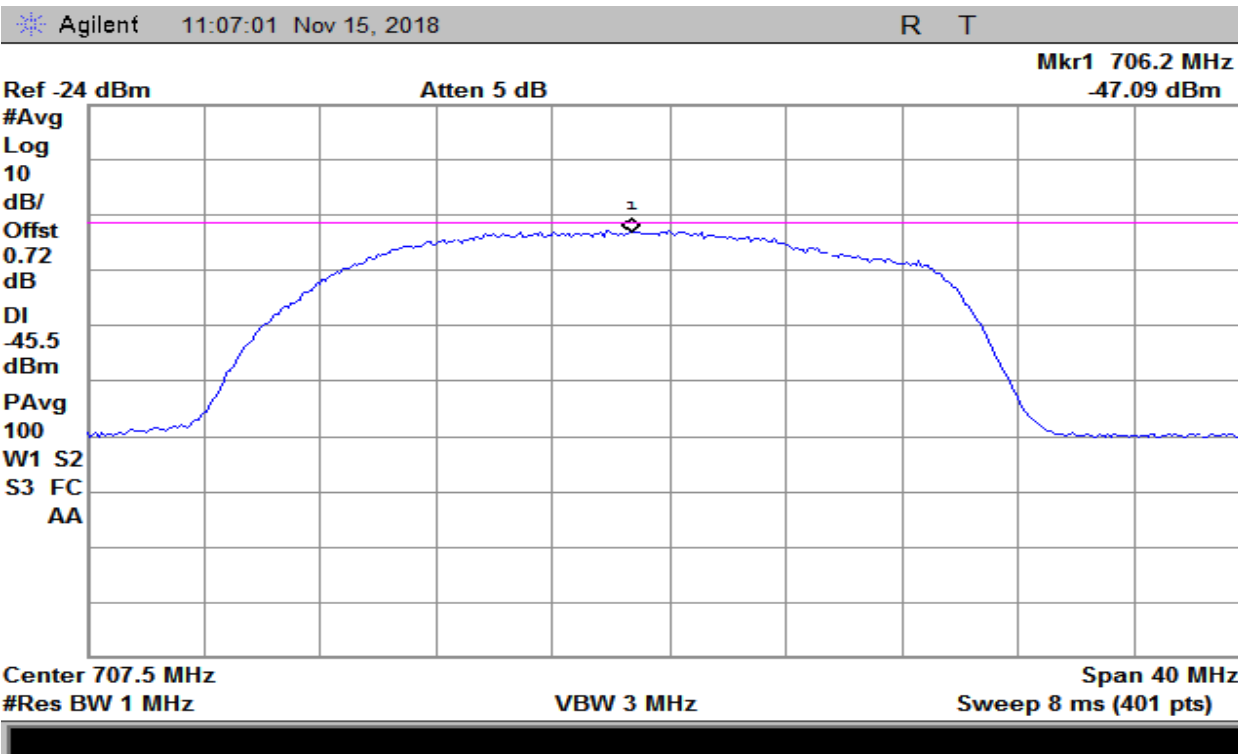
Plot 121 – 698-716MHz Band – Maximum Uplink Noise
