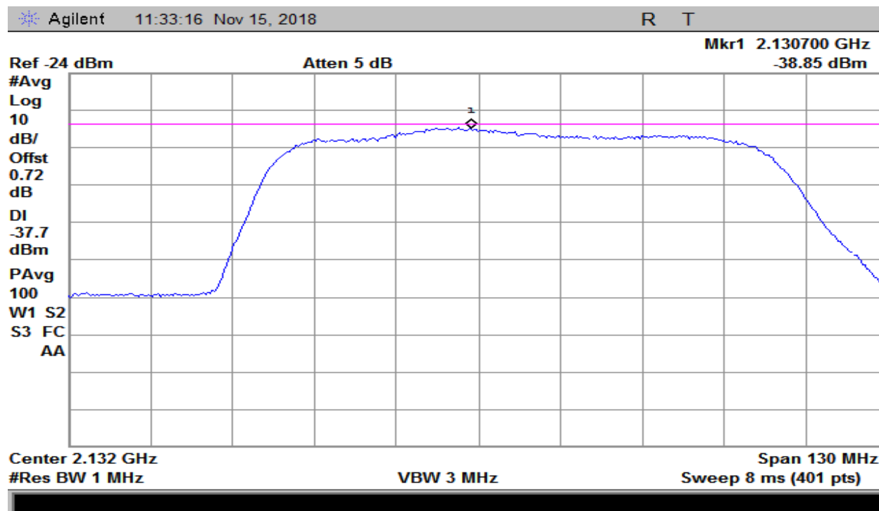
Plot 130 – 2110-2155MHz Band – Maximum Downlink Noise
