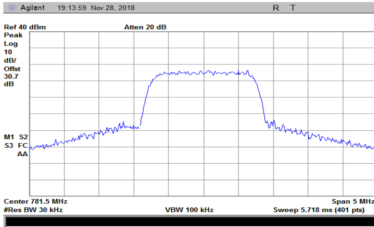
Plot 164 – 776-787MHz Band – Uplink Output – CDMA
