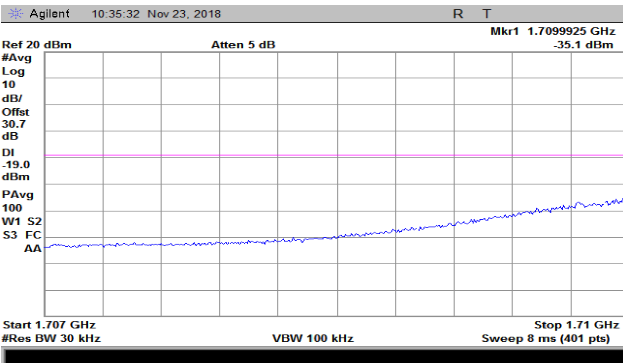
Plot 36 – 1710-1755MHz Band – CDMA Uplink Lower Band Edge
