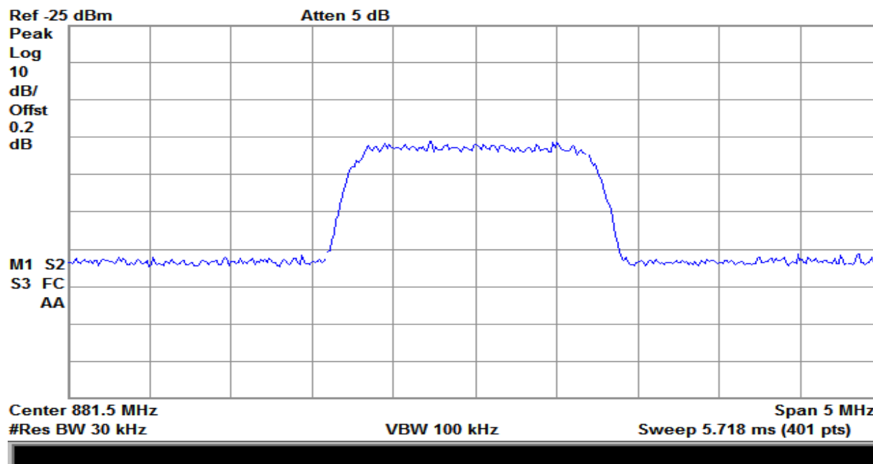
Plot 175 – 869-894MHz Band – Downlink Input – CDMA
