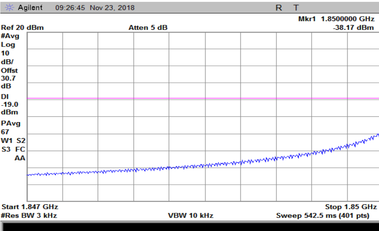
Plot 28 – 1850-1915MHz Band – GSM Uplink Lower Band Edge
