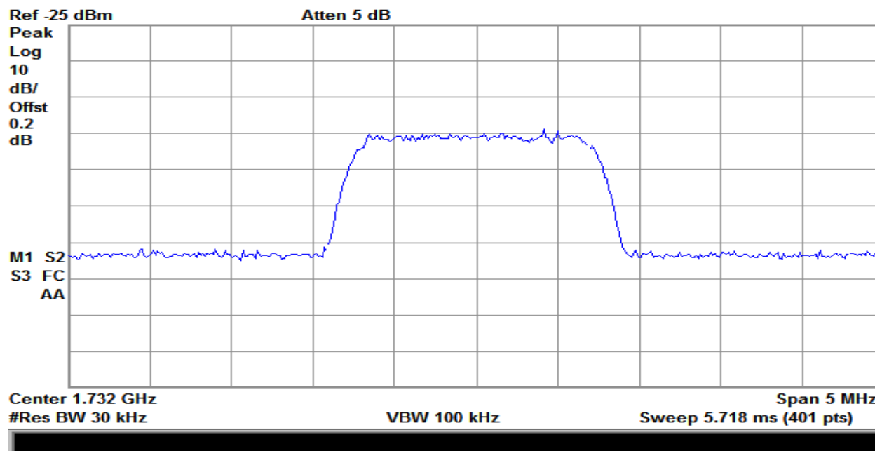
Plot 167 – 1710-1755MHz Band – Uplink Input – CDMA
