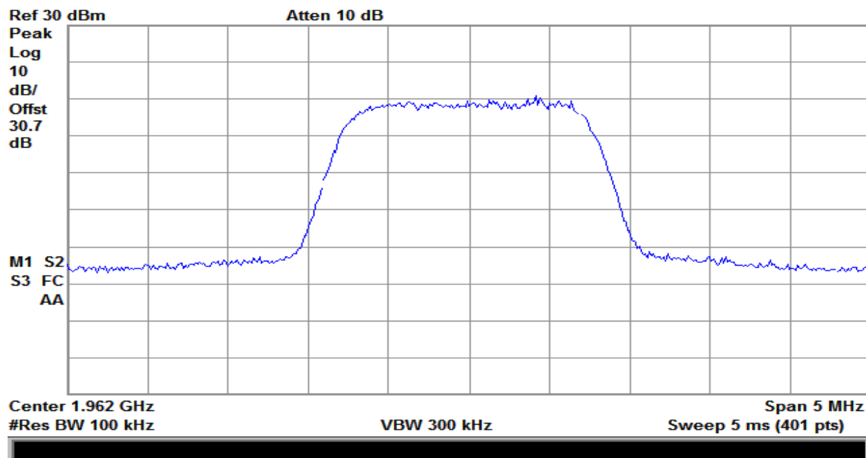
Plot 178 – 1930-1995MHz Band – Downlink Output – CDMA
