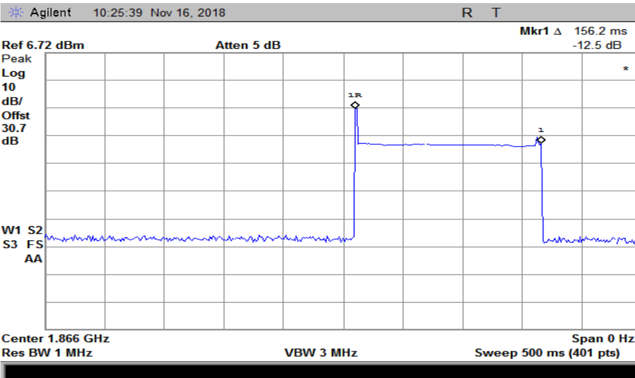
Plot 215 – 1850-1915MHz Band – Uplink Oscillation Detection Time
