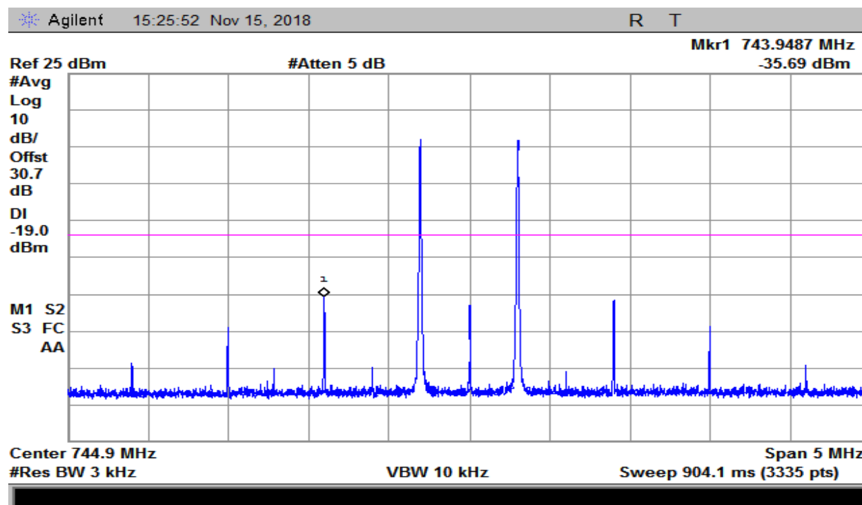
Plot 16 – 728-746MHz Band – Downlink
