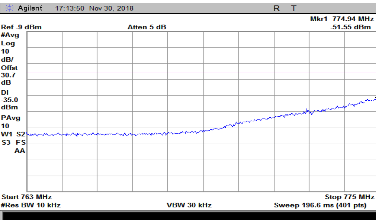
Plot 114 -27.53c4 – Uplink
