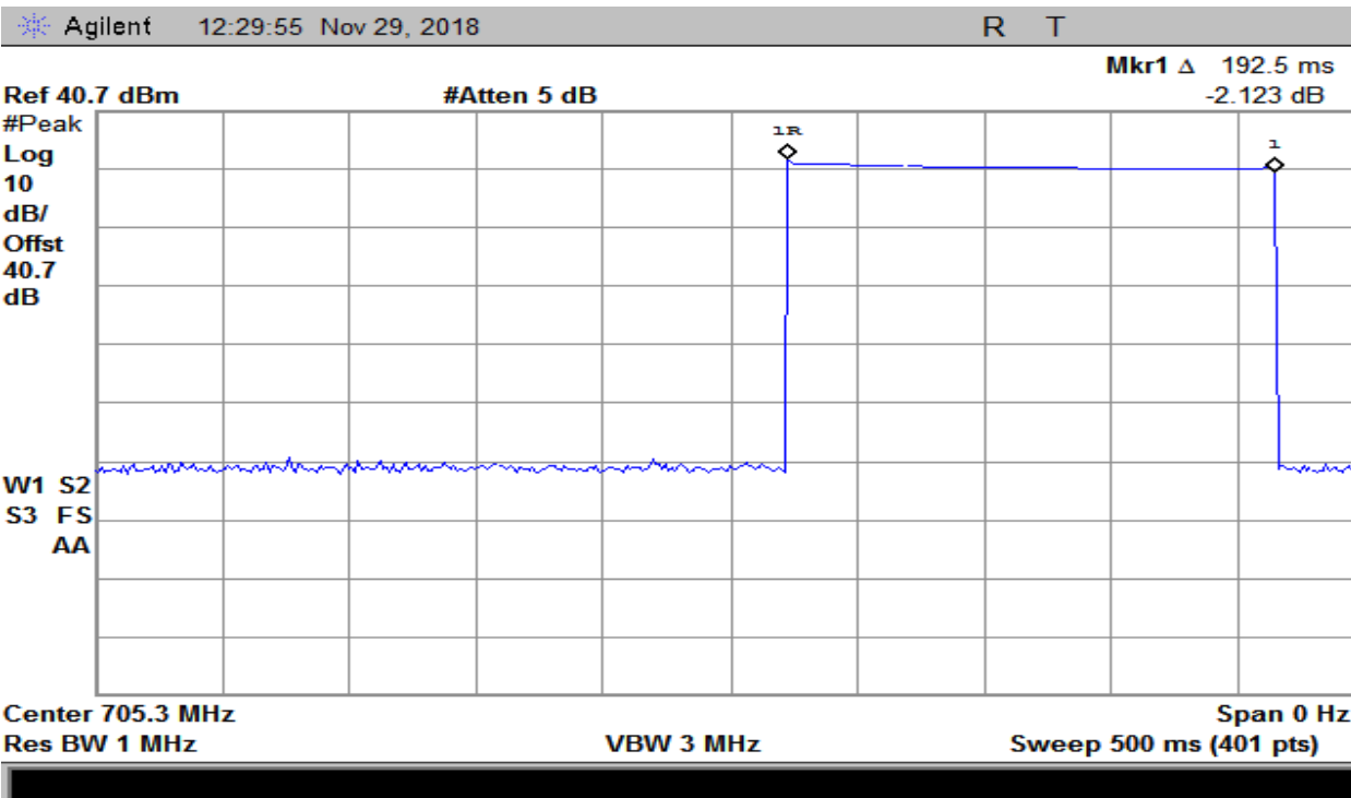
Plot 211 – 698-716MHz Band – Uplink Oscillation Detection Time
