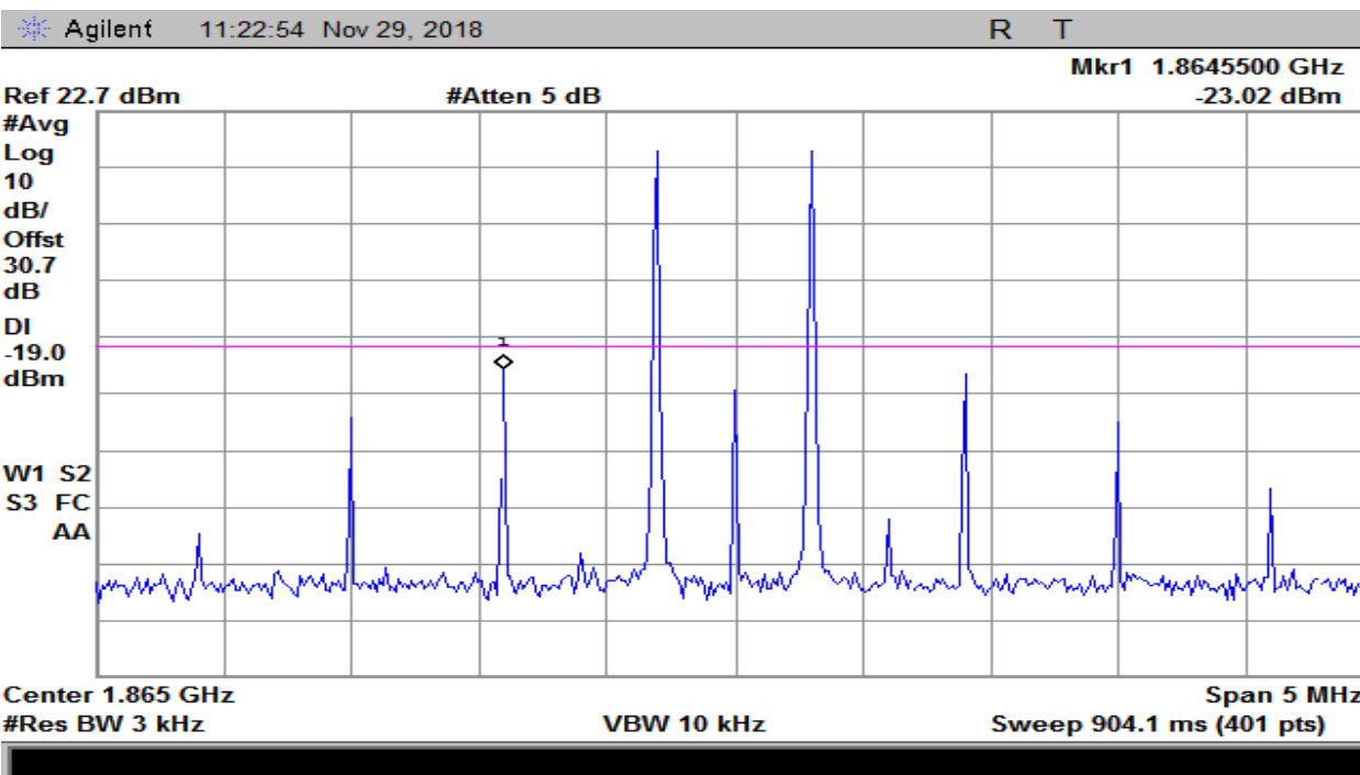
Plot 15 – 1850-1915MHz Band – Uplink
