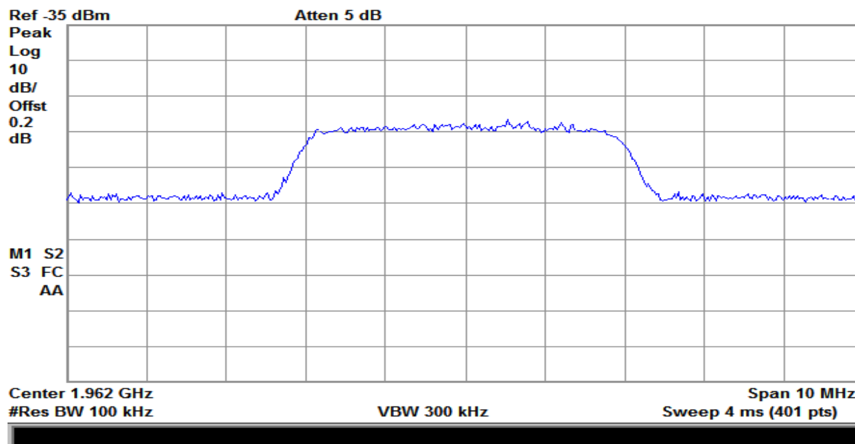
Plot 197 – 1930-1995MHz Band – Downlink Input – LTE
