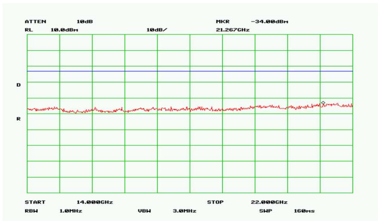
Plot 113 –2110-2155MHz Band – Downlink
