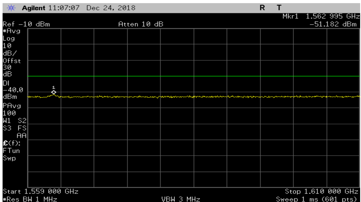
Plot 117 –27.53f – Uplink Wideband
