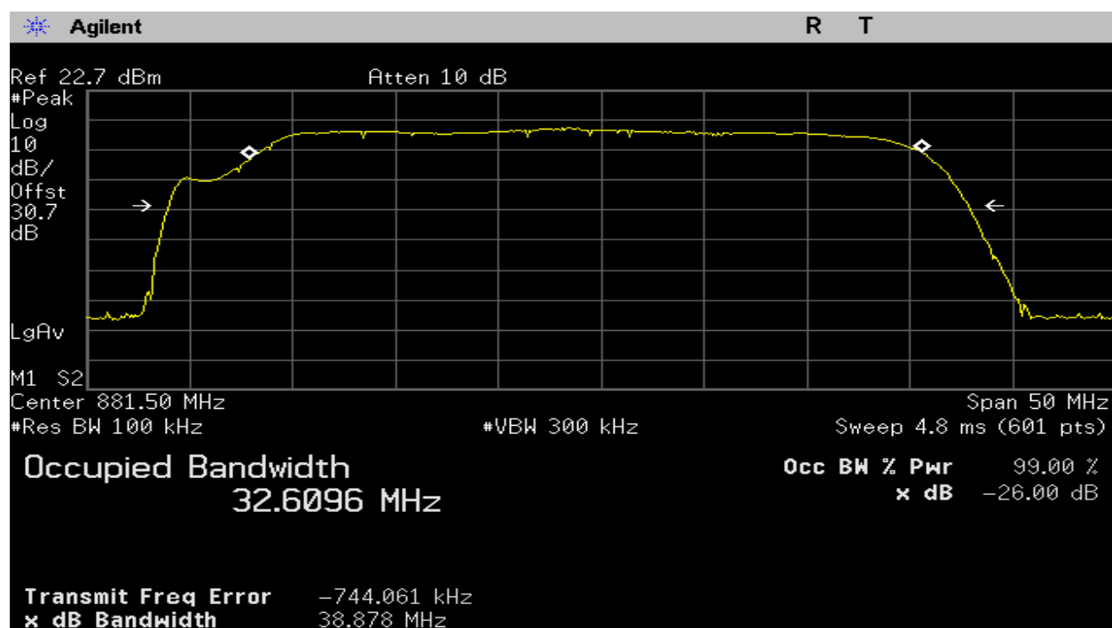
Plot 208 – 869-894MHz Band – Downlink – 99% BW for ISED (Canada)
