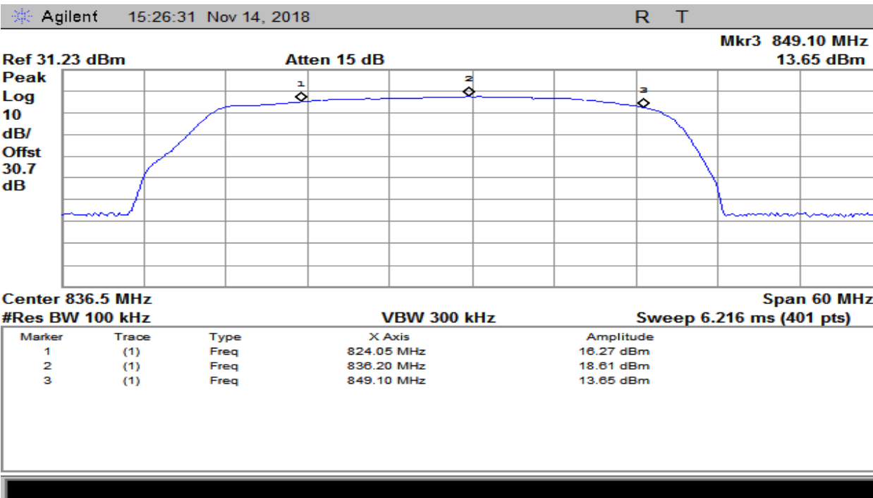
Plot 3 – 824-849MHz Band – Uplink
