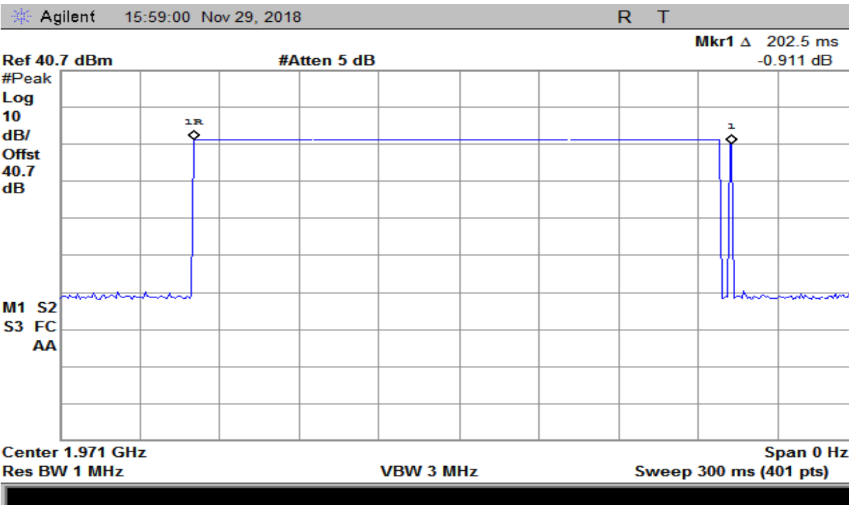
Plot 219 – 1930-1995MHz Band – Downlink Oscillation Detection Time
