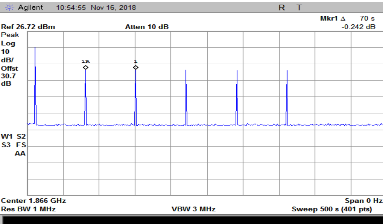
Plot 235 – 1850-1915MHz Band – Uplink # of Restart Time
