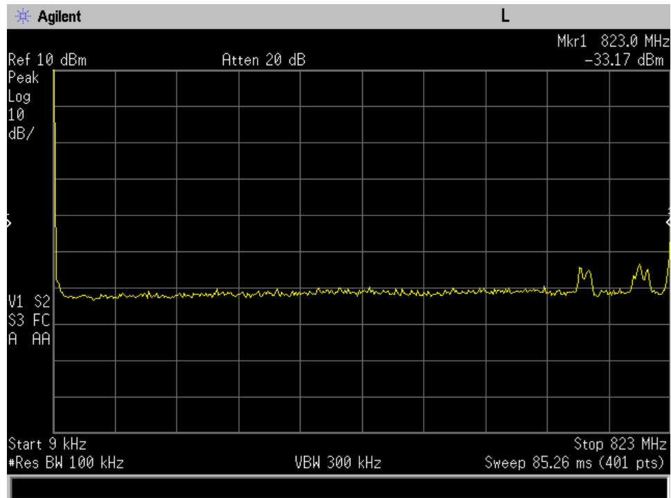
Uplink_824 - 849 MHz_plot 1
