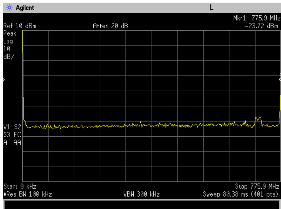
Uplink_776 - 787 MHz_plot 1
