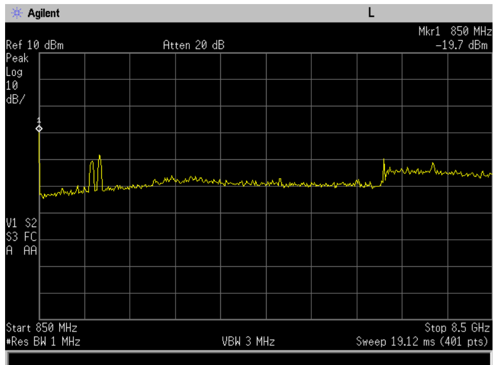
Uplink_824 - 849 MHz_plot 2
