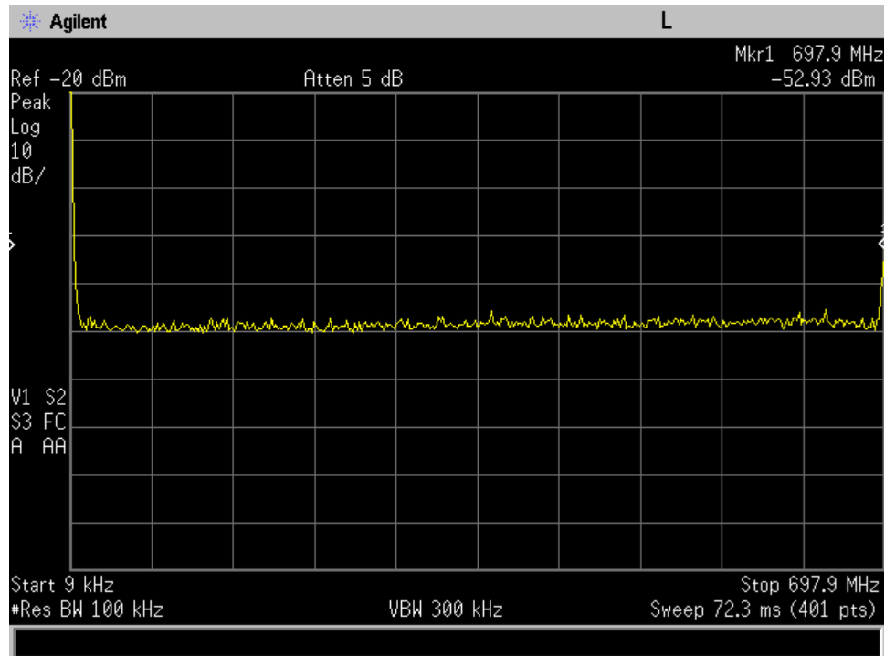
Uplink_698 - 716 MHz_plot 1
