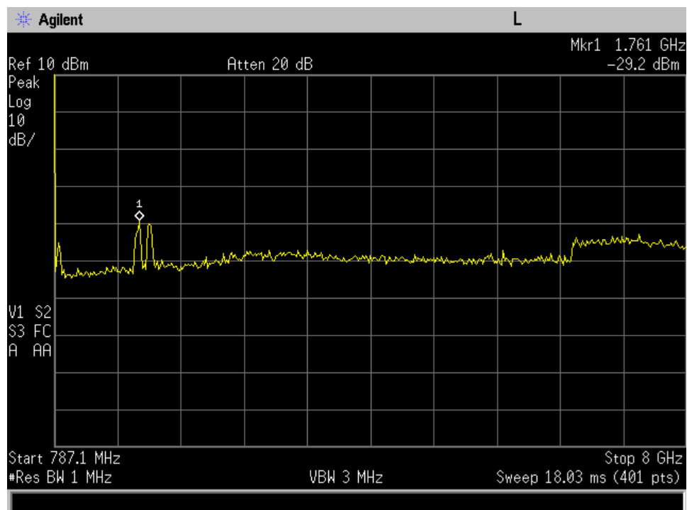
Uplink_776 - 787 MHz_plot 2
