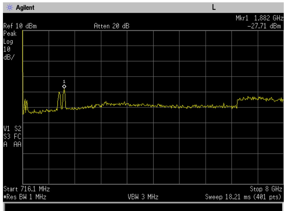
Uplink_698 - 716 MHz_plot 2
