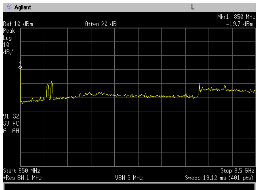
Uplink_824 - 849 MHz_plot 2
