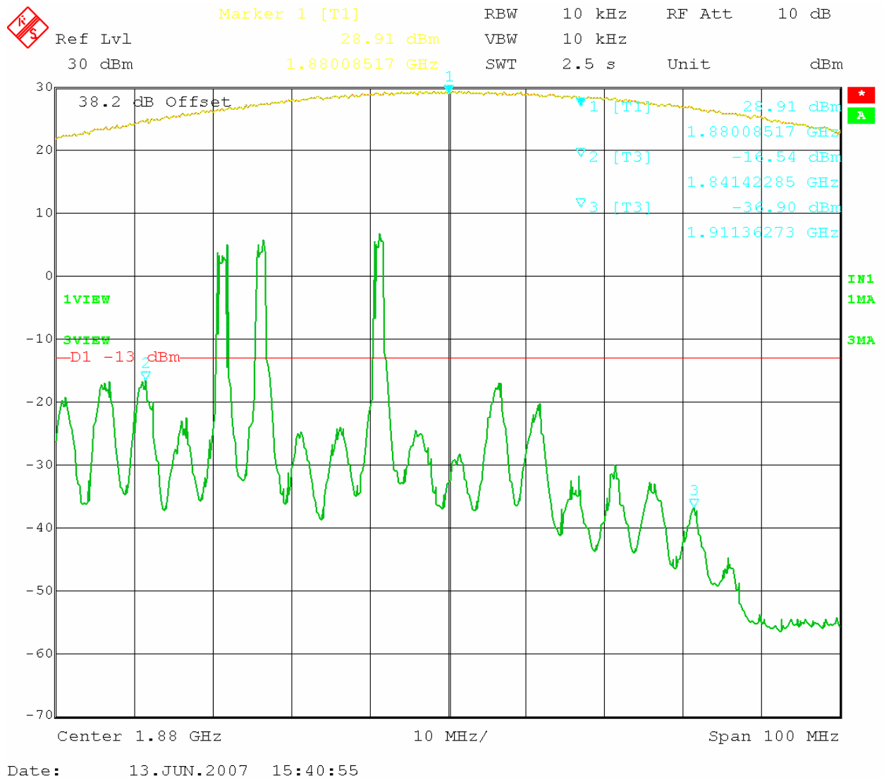
Figure 29: CDMA 3 tones intermodulation - (1850 – 1910) MHz.
