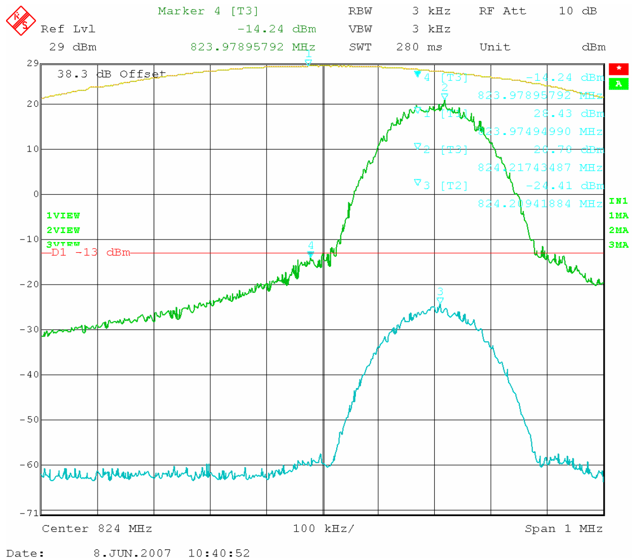
Figure 21: GSM – In vs. Out 824.2 MHz
