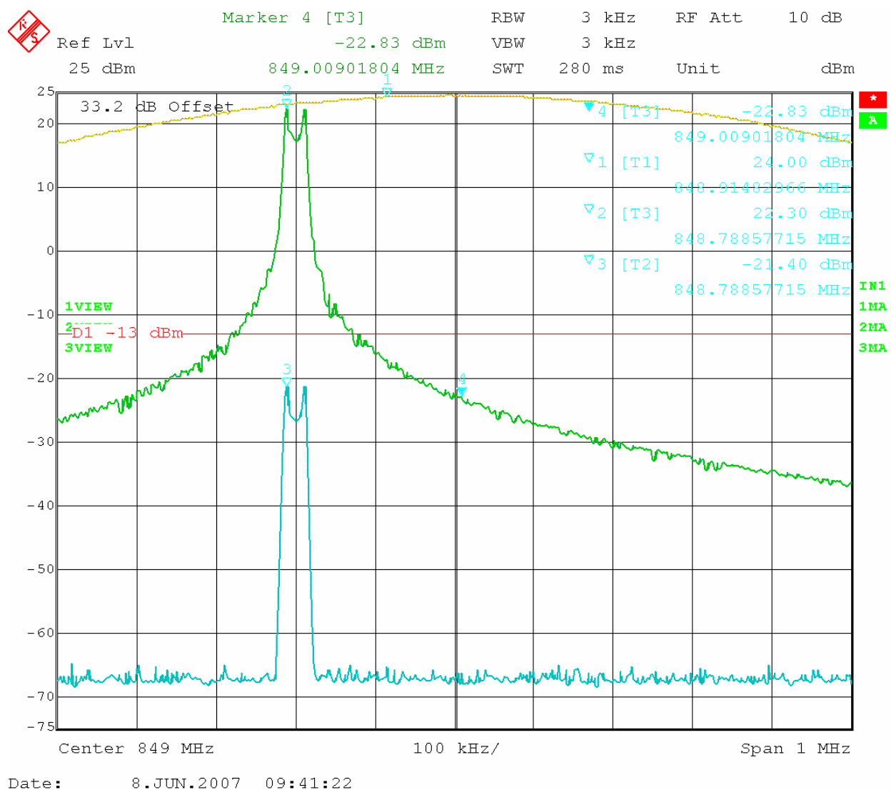
Figure 26: AMPS – In vs. Out 848.80 MHz
