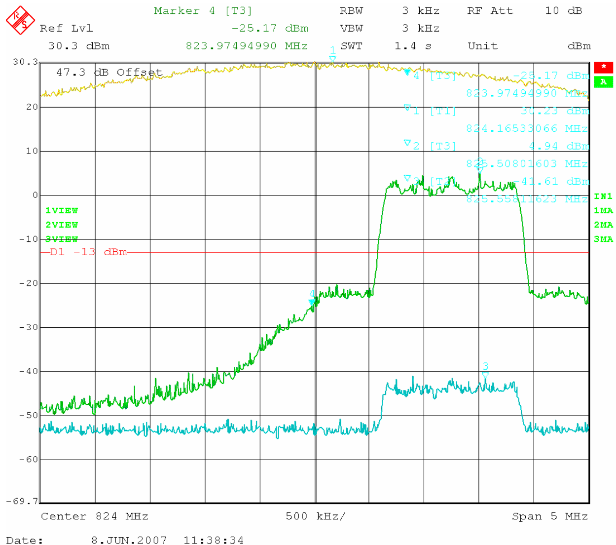
Figure 13: CDMA – In vs. Out 825.25MHz
