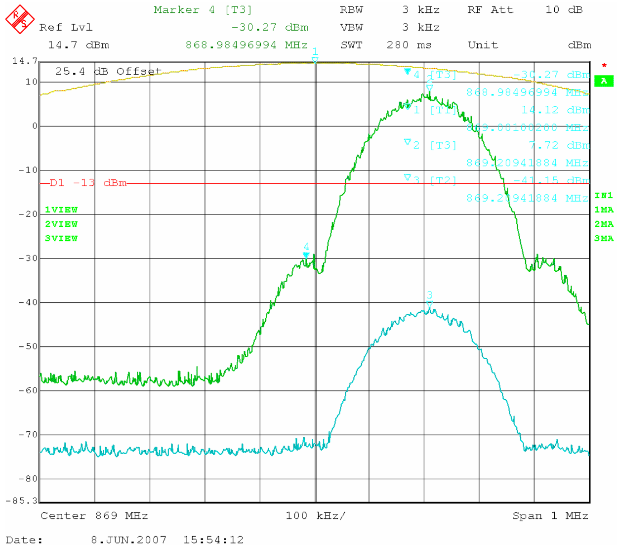
Figure 23: GSM – In vs. Out 869.2MHz
