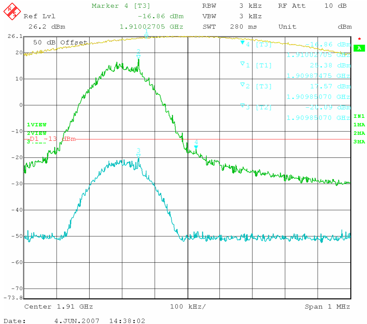
Figure 6: EDGE – In vs. Out 1909.80MHz
