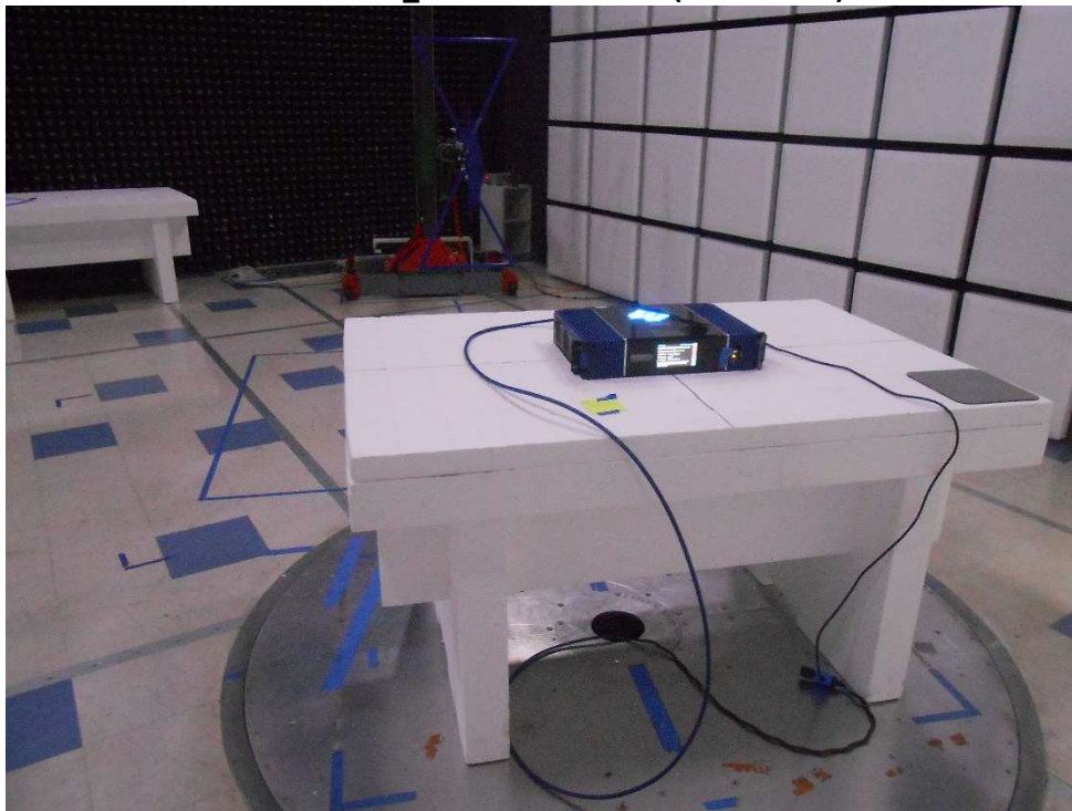
RF Radiated_ 30 – 1000 MHz #1 (rack mount)
