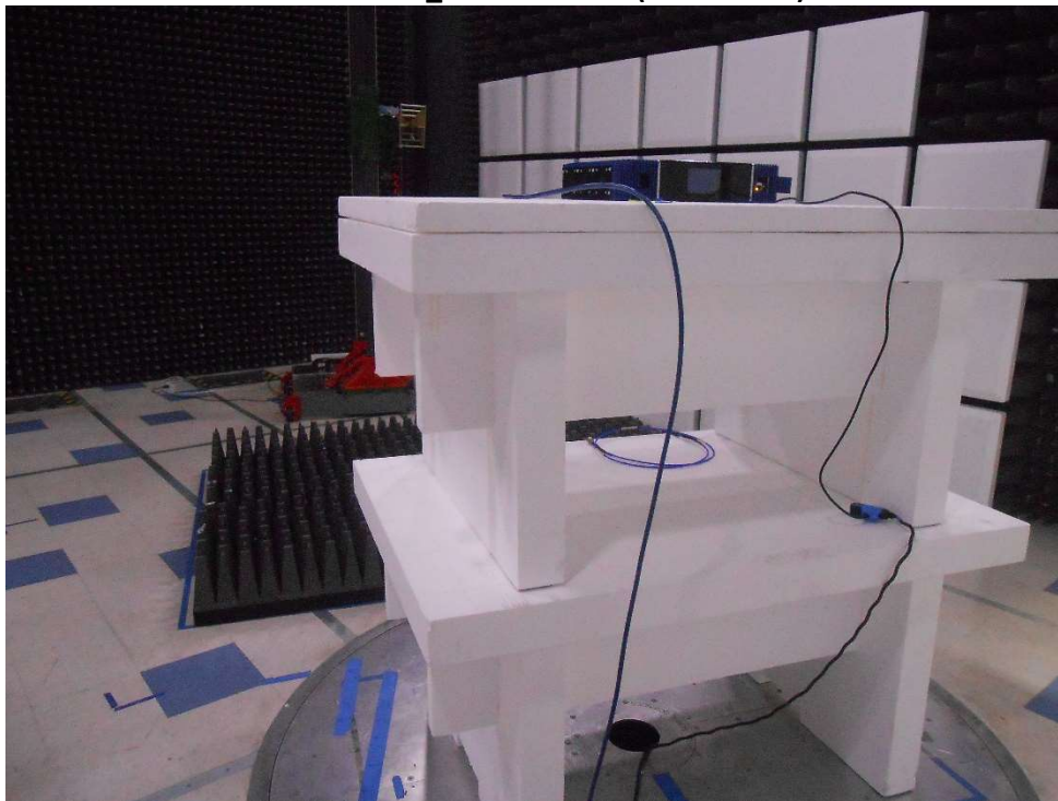
RF Radiated_1 – 18 GHz #1 (wall mount)
