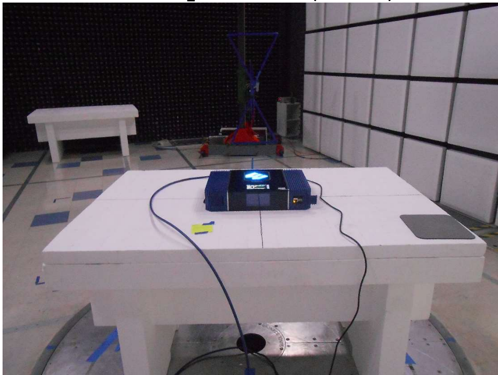
RF Radiated_ 30 – 1000 MHz #1 (wall mount)
