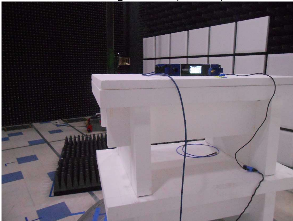
RF Radiated_ 1 – 18 GHz #1 (rack mount)
