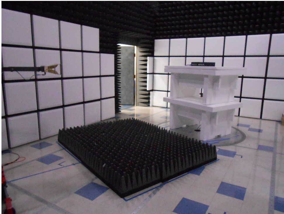
Radiated Emissions_ above 1 GHz_ wall mount
