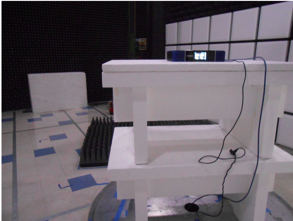
Radiated Emissions_ above 1 GHz_ rack mount
