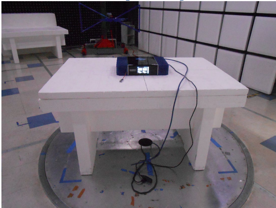
Radiated Emissions_ below 1 GHz_ rack mount
