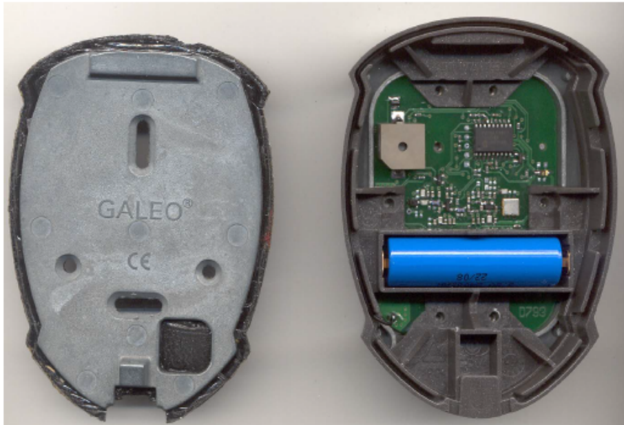
11.6 Galeo - rear view with battery and cover
