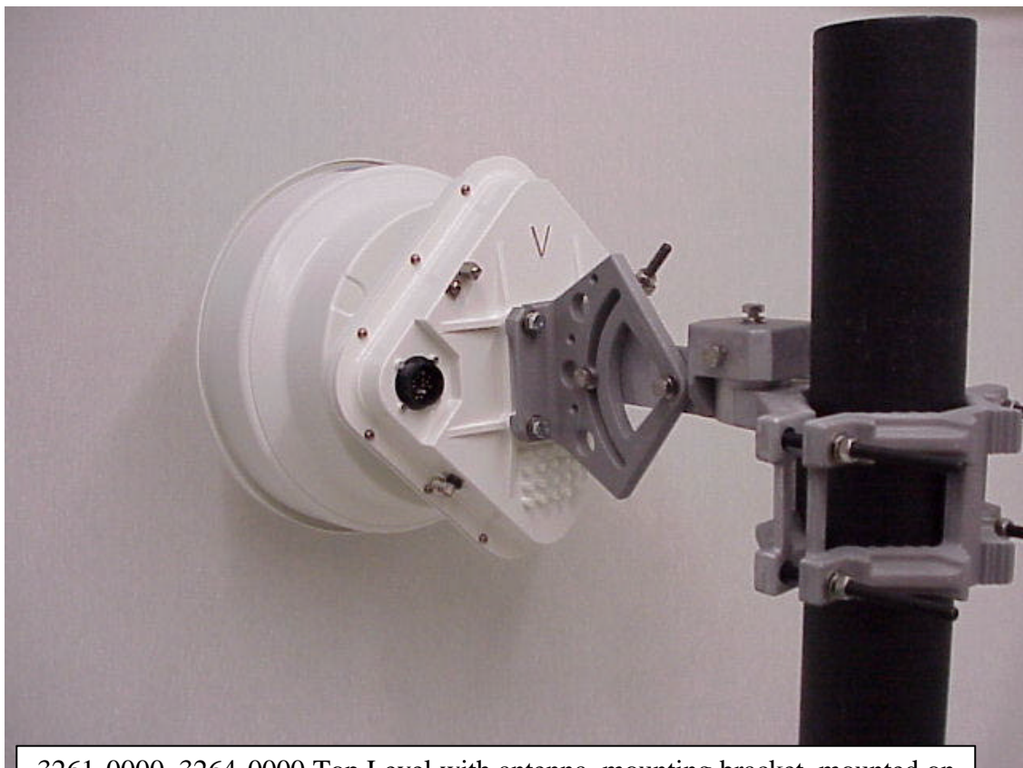
3261-0000, 3264-0000 Top Level with antenna, mounting bracket, mounted on pole.
