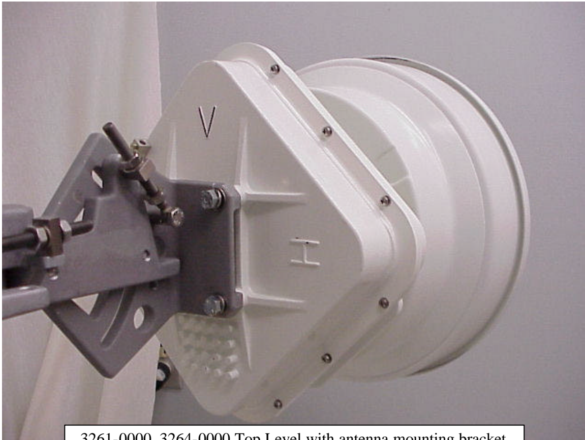
3261-0000, 3264-0000 Top Level with antenna mounting bracket, mounted on pole. Back view, Right
