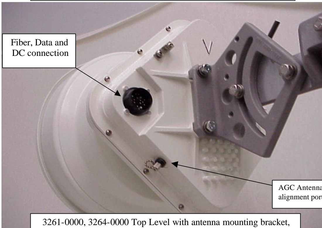
3261-0000, 3264-0000 Top Level with antenna mounting bracket, mounted on pole. Back view, Right
