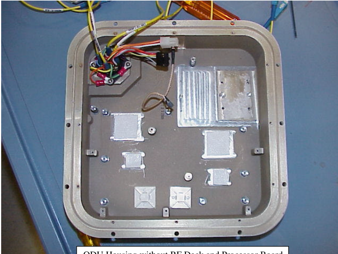
ODU Housing without RF Deck and Processor Board and SONET Interface board
