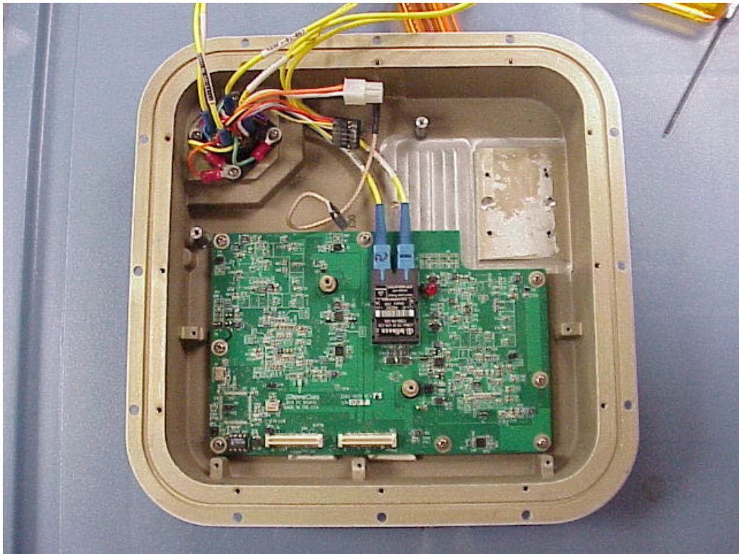
ODU Housing without RF Deck and Processor Board
