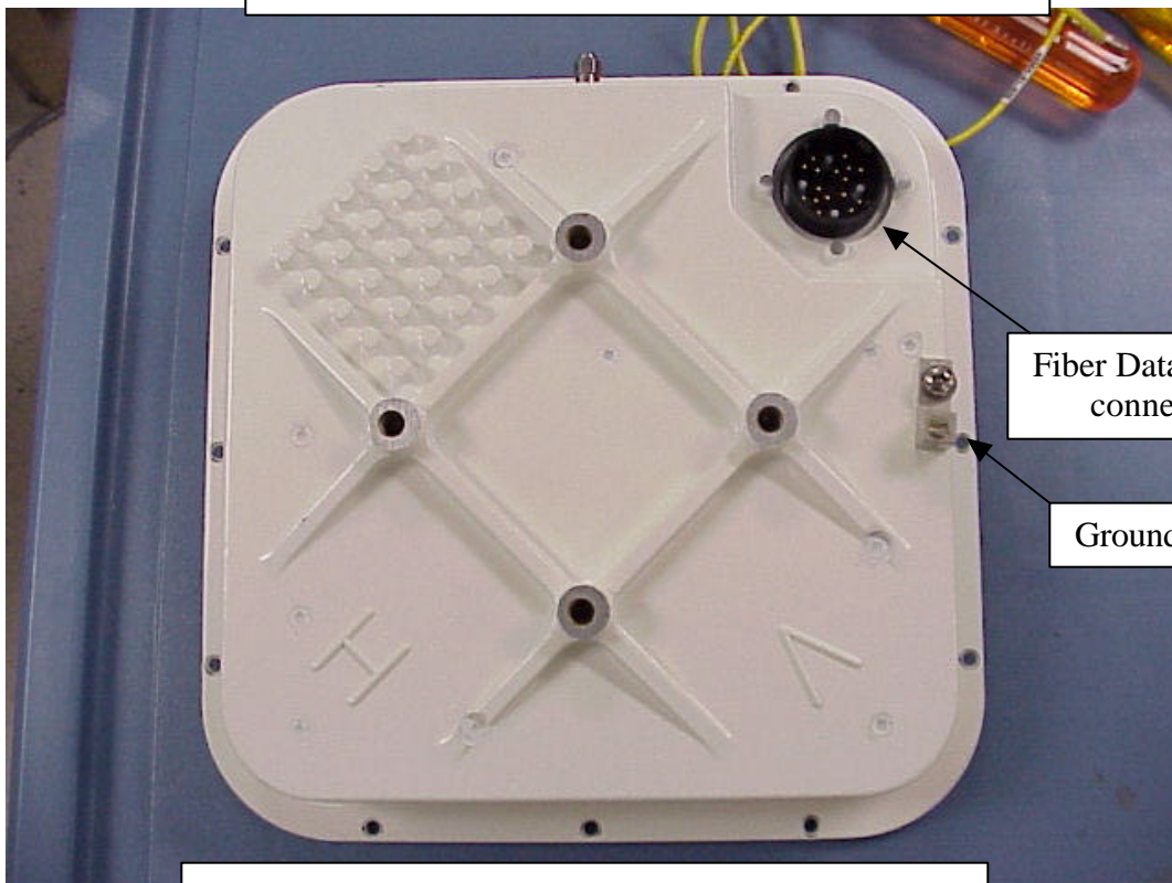
ODU Housing Back
