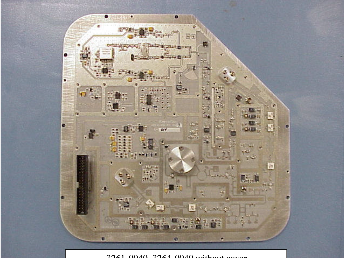
3261-0040, 3264-0040 without cover
