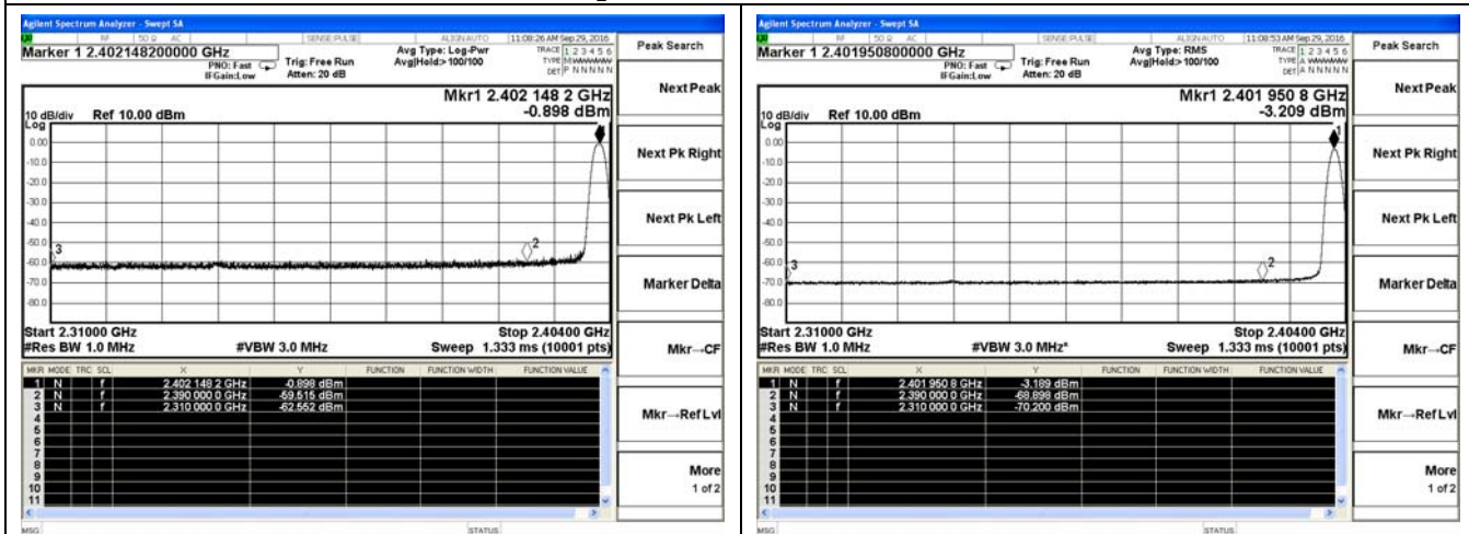
BLE-Low channel(Peak)
