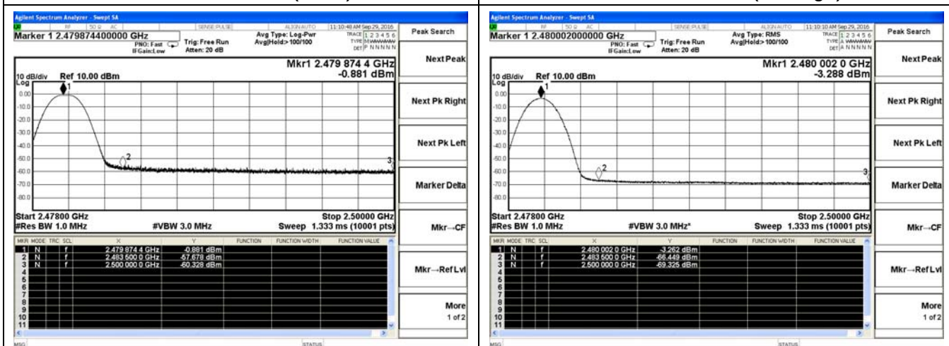
BLE-High channel(Peak)
