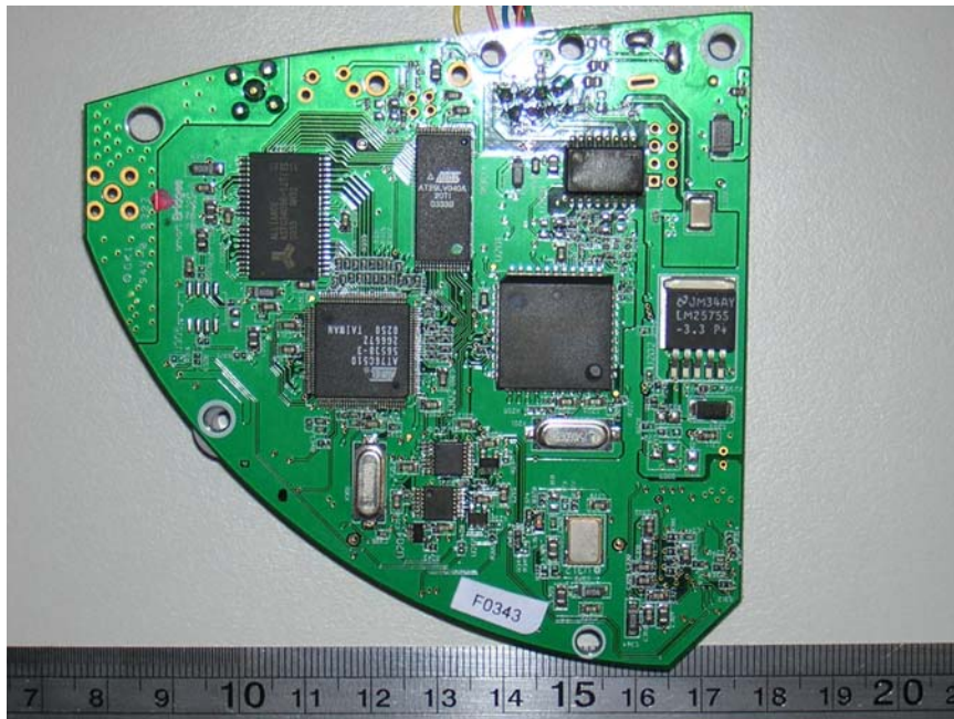
Radio B – Bottom View
