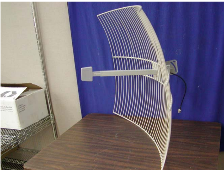
Antenna 3: WISP 24024 PTNF 24dBi parabolic Grid Rear View
