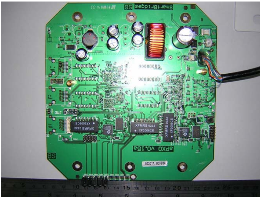
EUT (airPoint XO) – Main Board Component View
