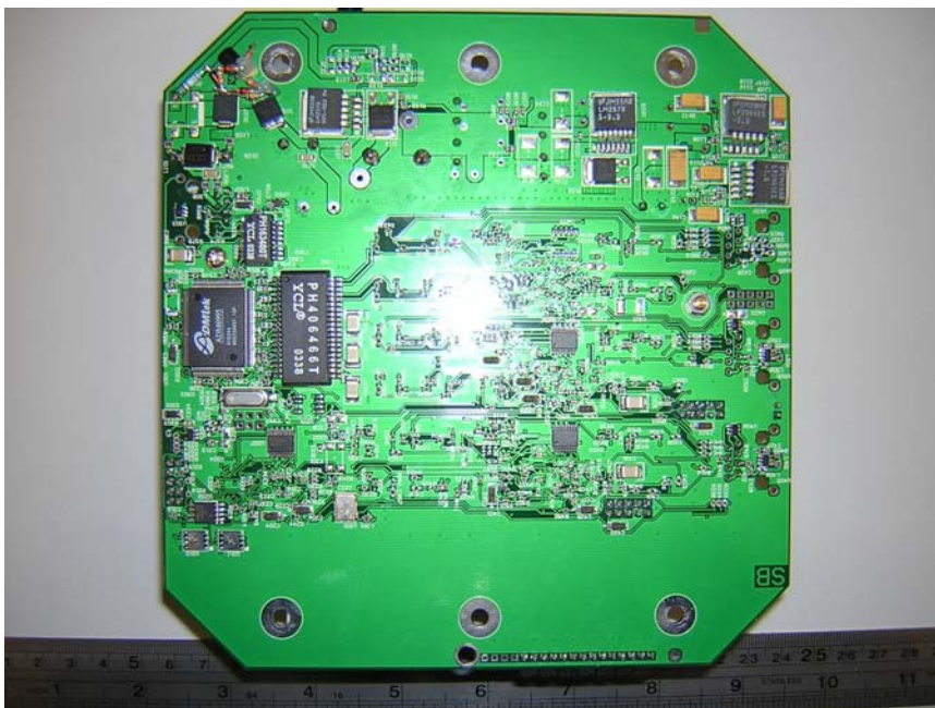
EUT (airPoint XO) – Main Board Solder View
