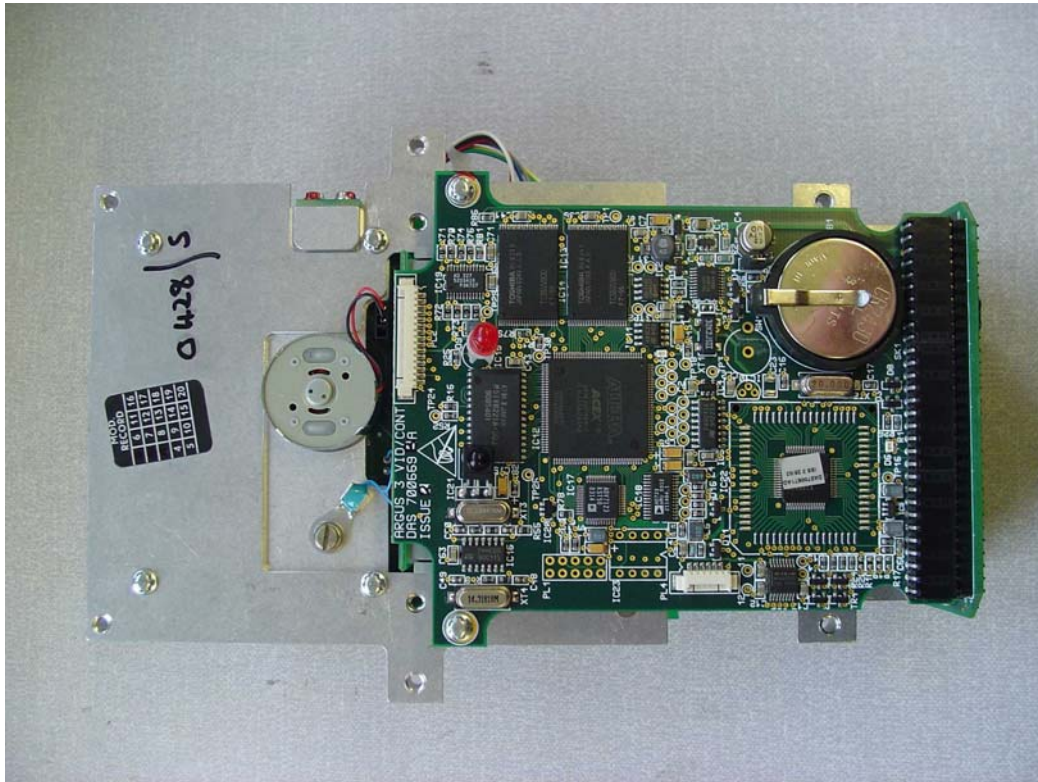
BST Chassis – Rear view showing Mabuchi shutter mortor
