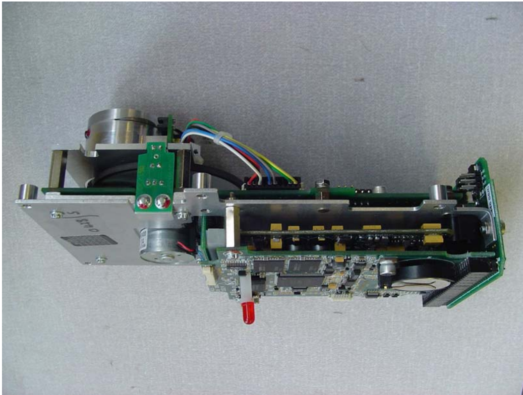
BST Chassis – Side View
