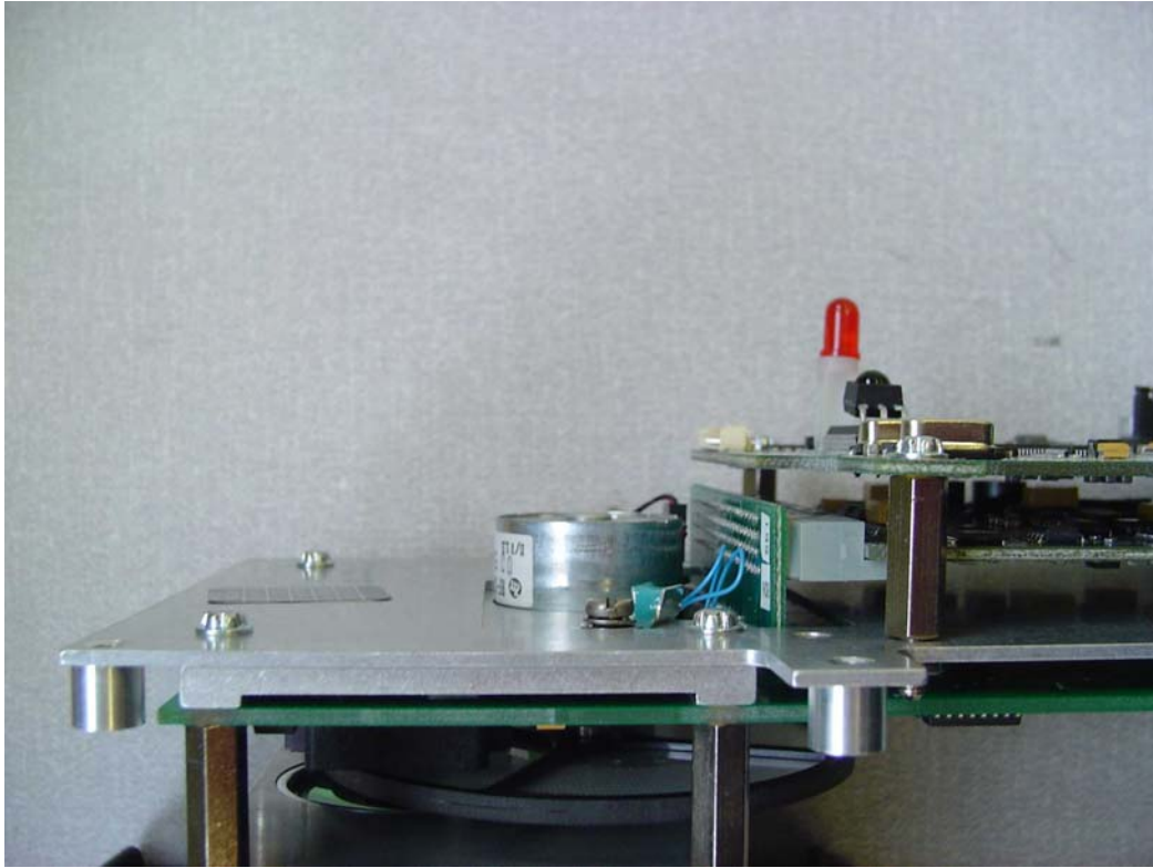
BST Chassis – Close-up of Mabuchi shutter motor
