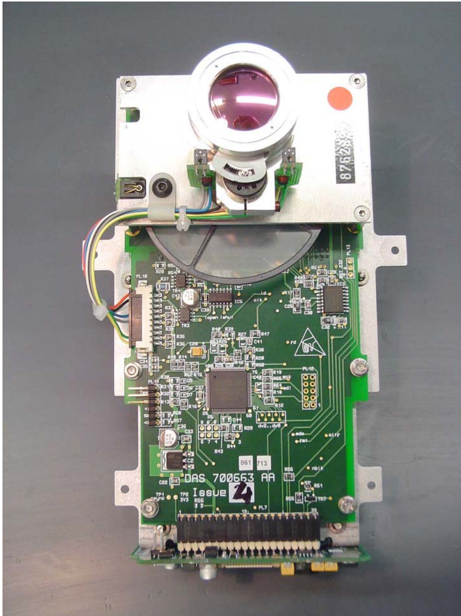
BST Chassis - Front View
