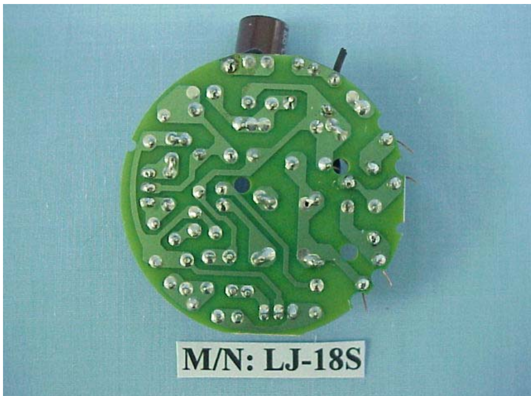
FIGURE 9 ENERGY SAVING LAMP (M/N: LJ-18S) MAIN BOARD (SOLDERED SIDE)
