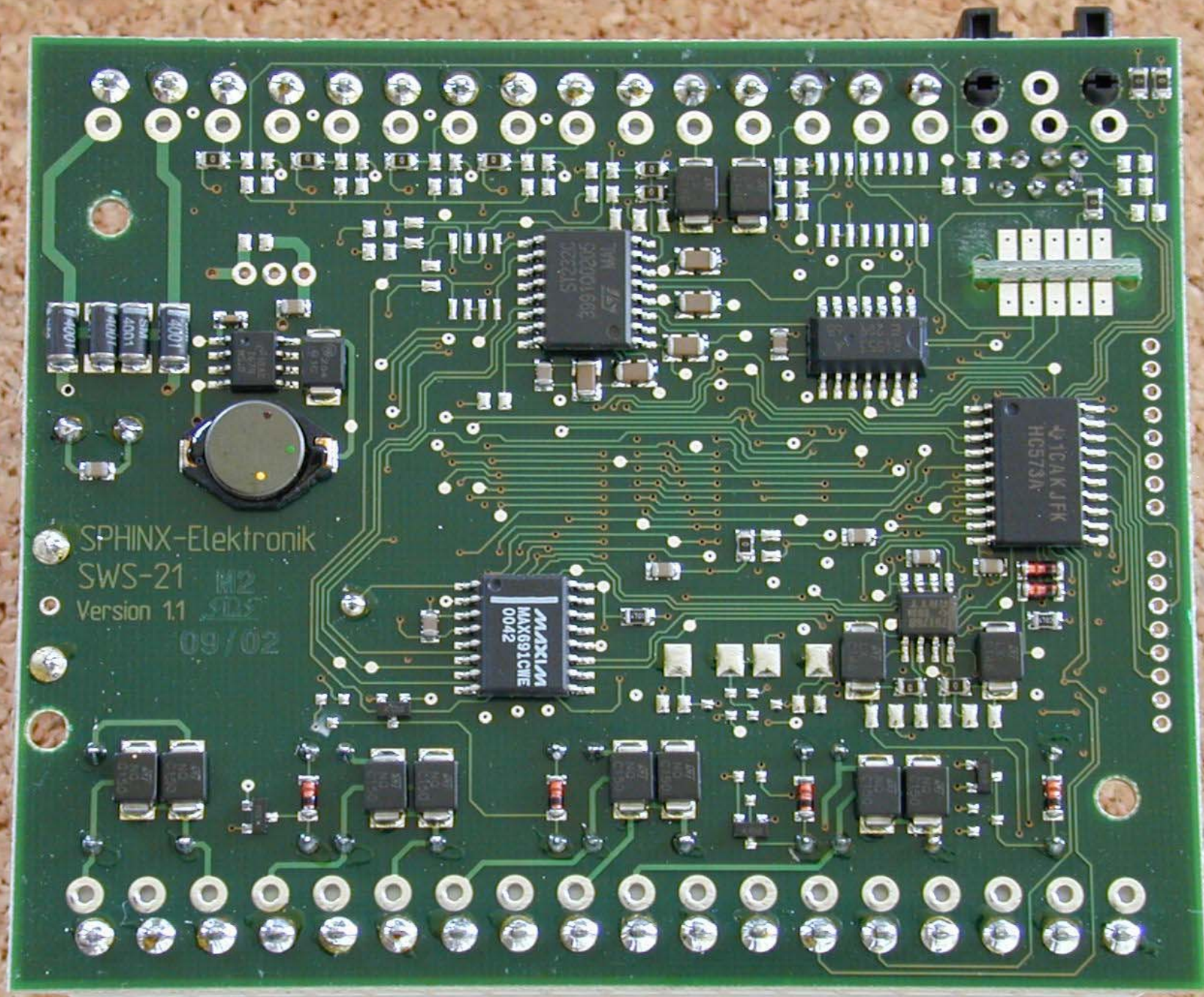
WT2000L Contol Box PCB (bottom)
