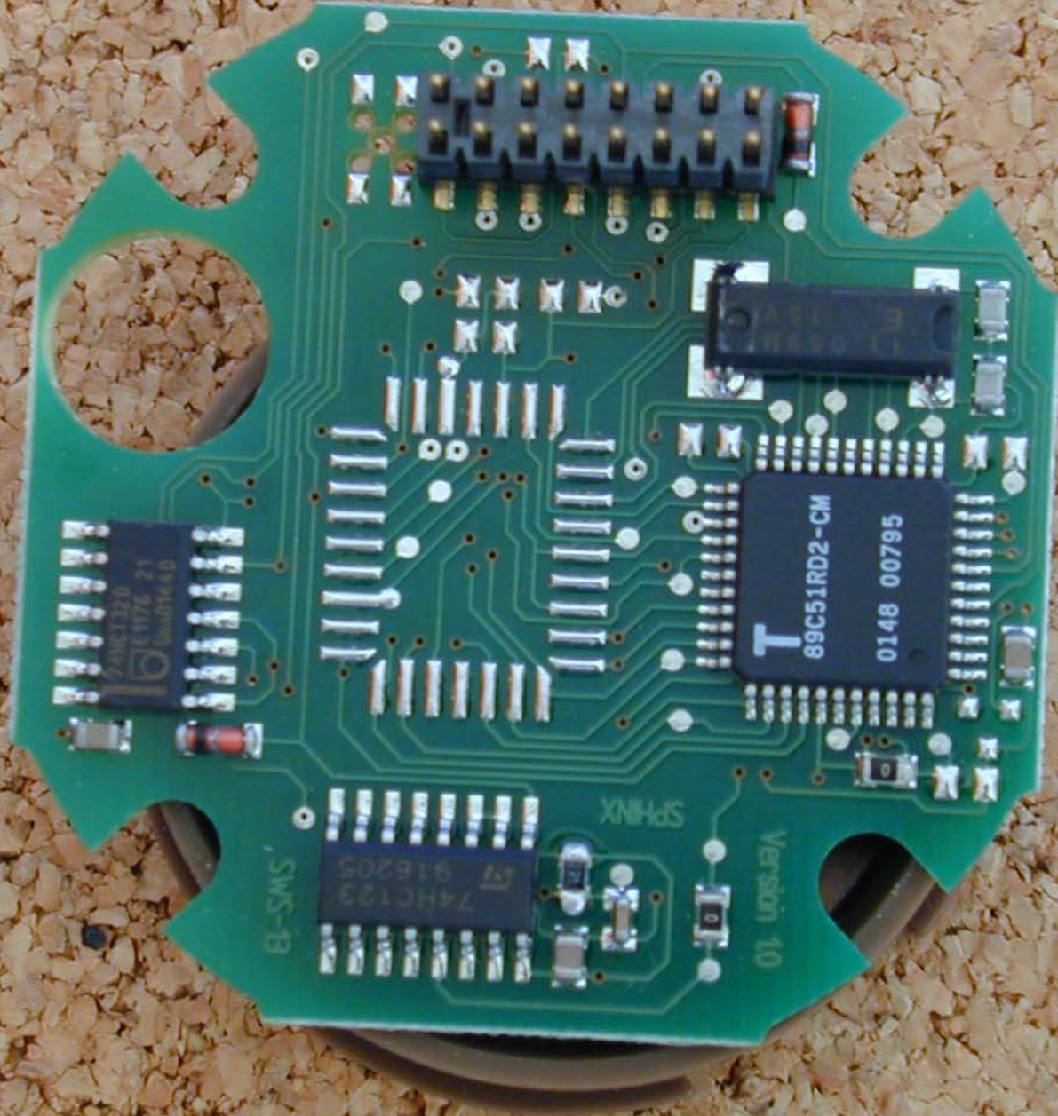
WT2000L PCB3 (top)
