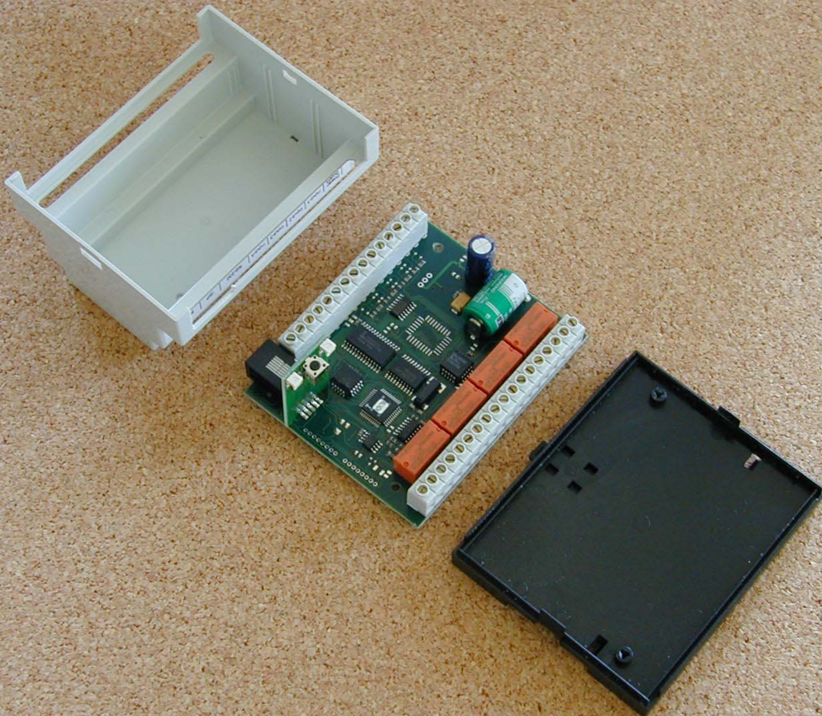
WT2000L Control Box apart (bottom)
