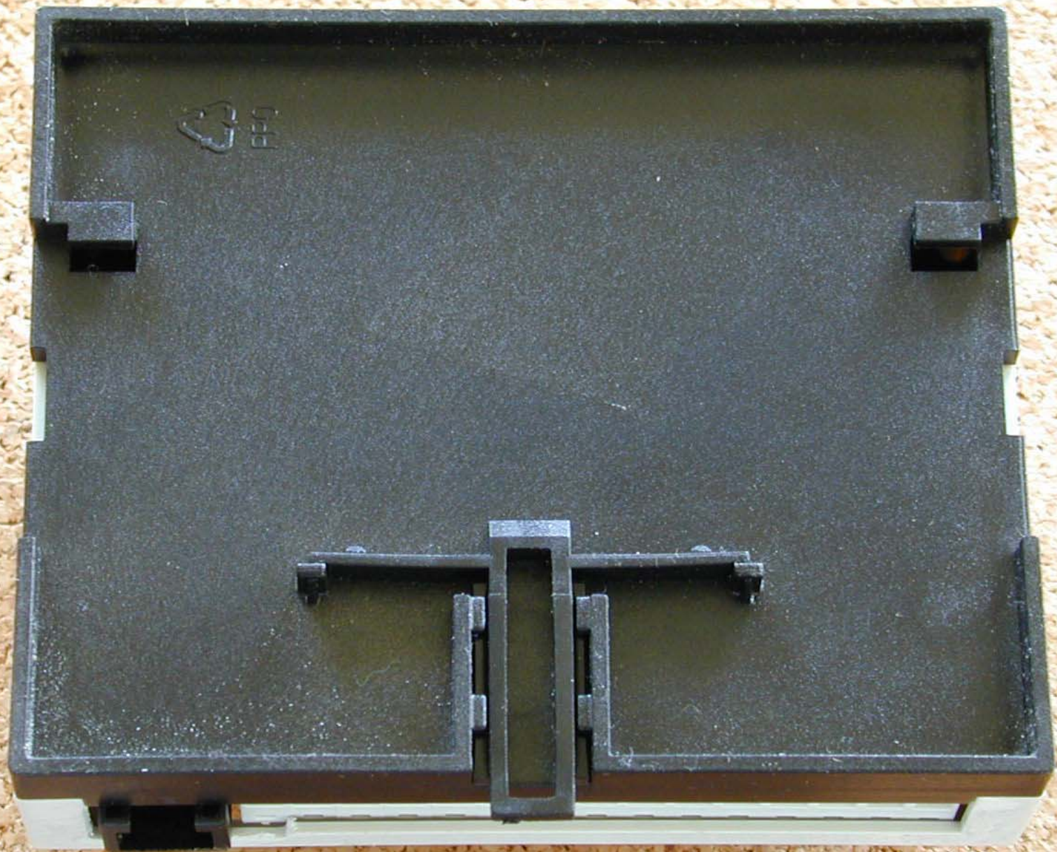
WT2000L Control Box (bottom)
