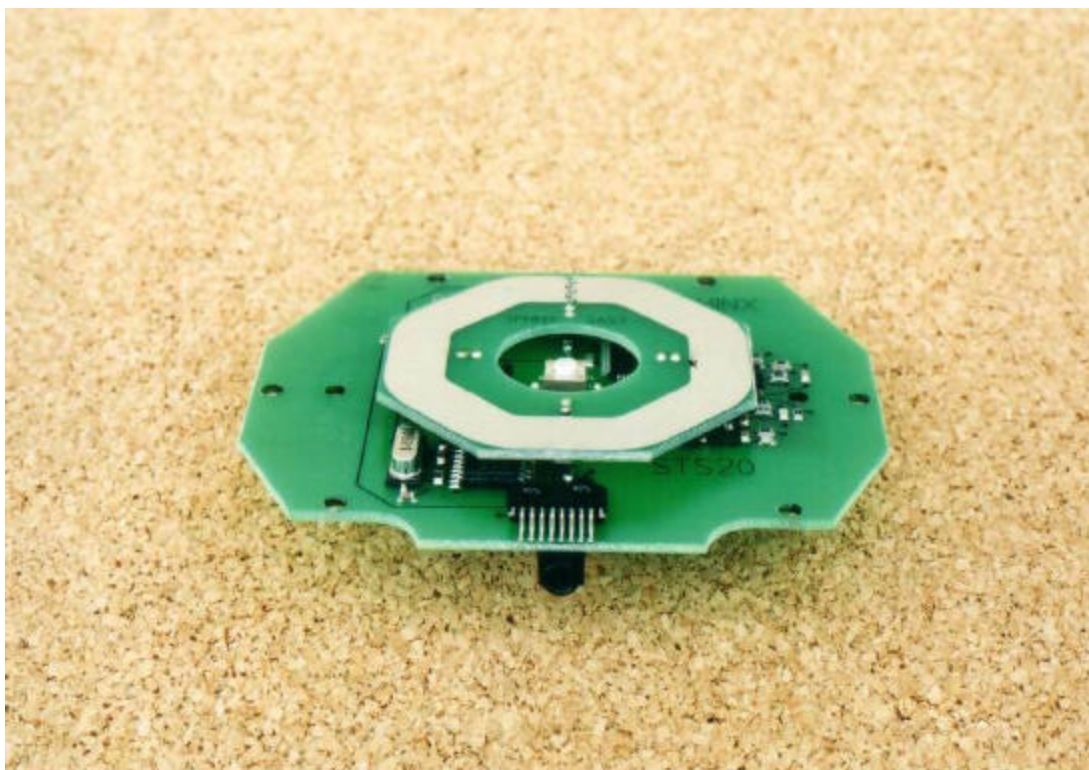
DMT 32 (LEGIC) PCB Front with Coil
