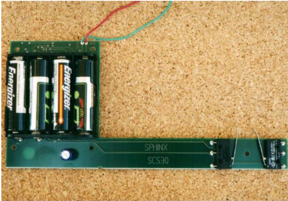
DMT 32 (TIRIS) – Internal PCB Back
