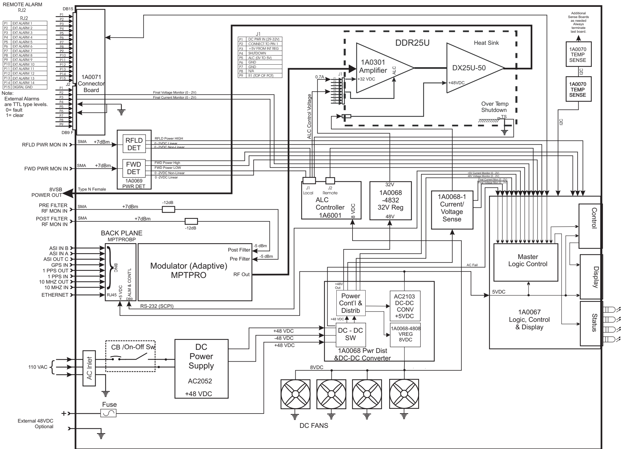
DXDPRO-10U DIGITAL MODULATOR (Used in DTXPRO-10U and DTXPRO-400U AND HIGHER TRANSMITTERS)
