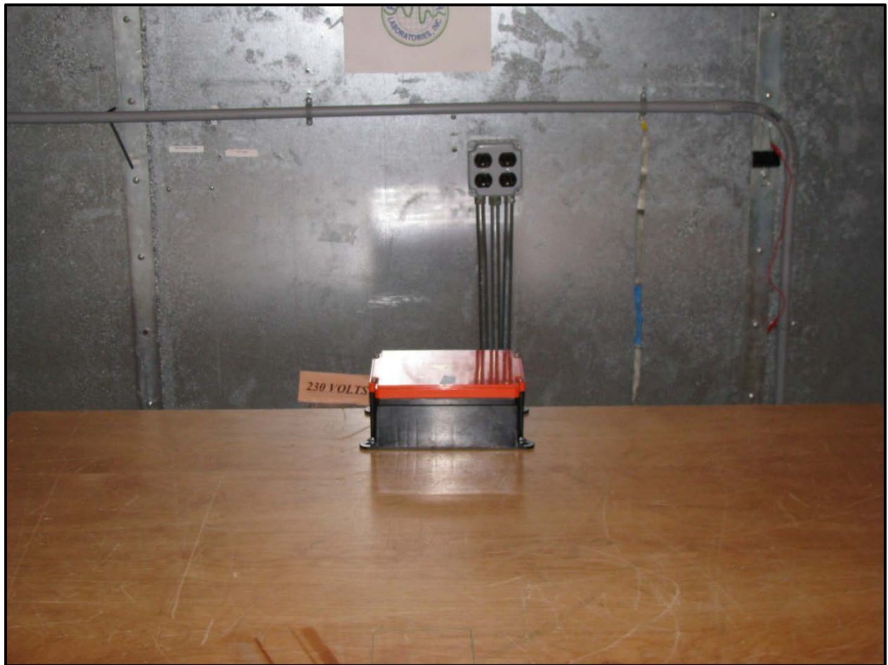
Photograph 3: Conducted AC Emissions - Front View - Module Tested in "Typical Host"
