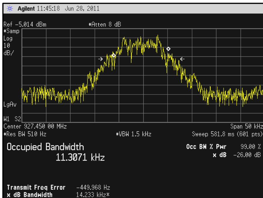
Plot 7-3: Occupied Bandwidth - High Channel
