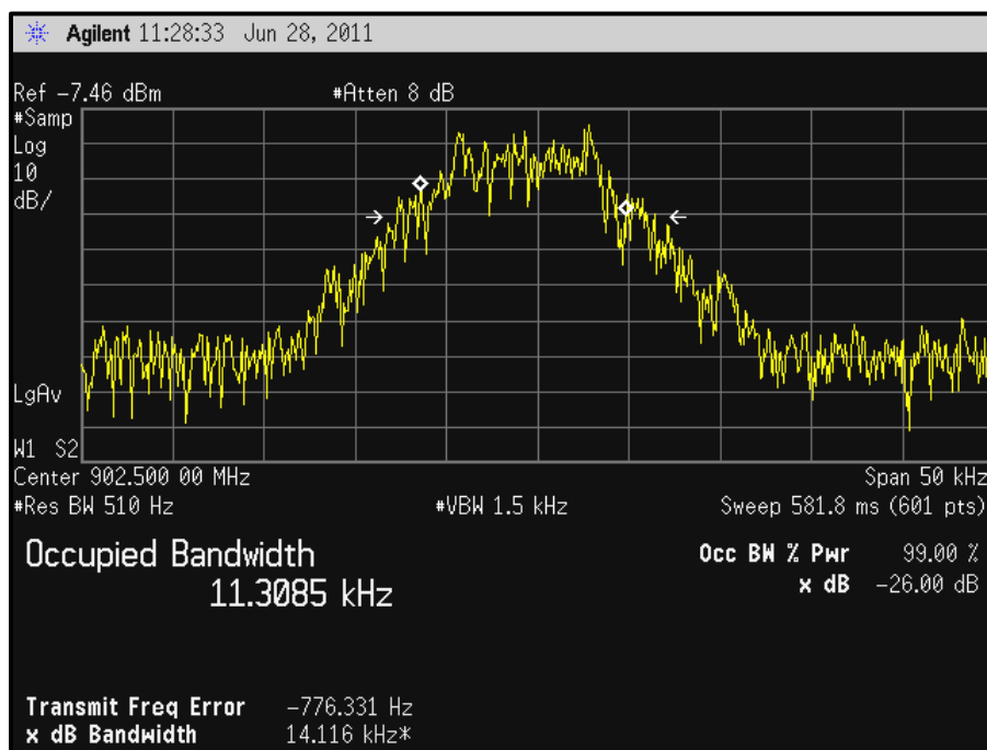
Plot 7-1: Occupied Bandwidth - Low Channel
