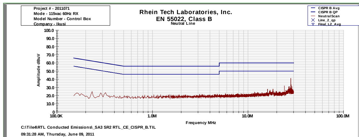
Plot 3-1: Conducted AC Emissions; Neutral (Line 1); Receive Mode
