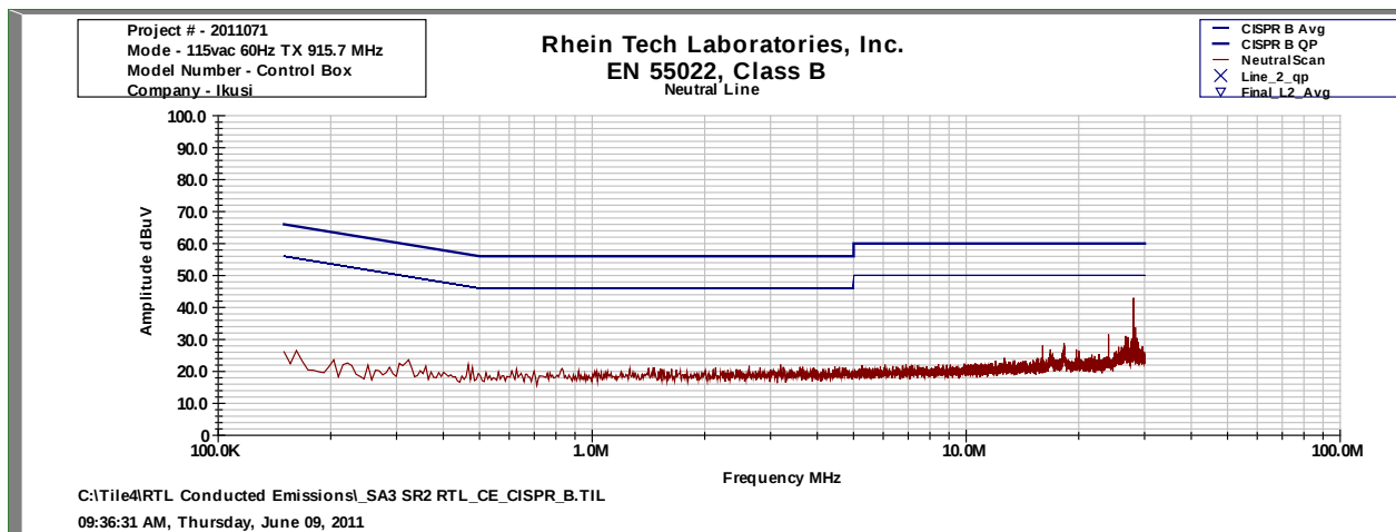
Plot 3-3: Conducted AC Emissions; Neutral (Line 1); Transmit Mode
