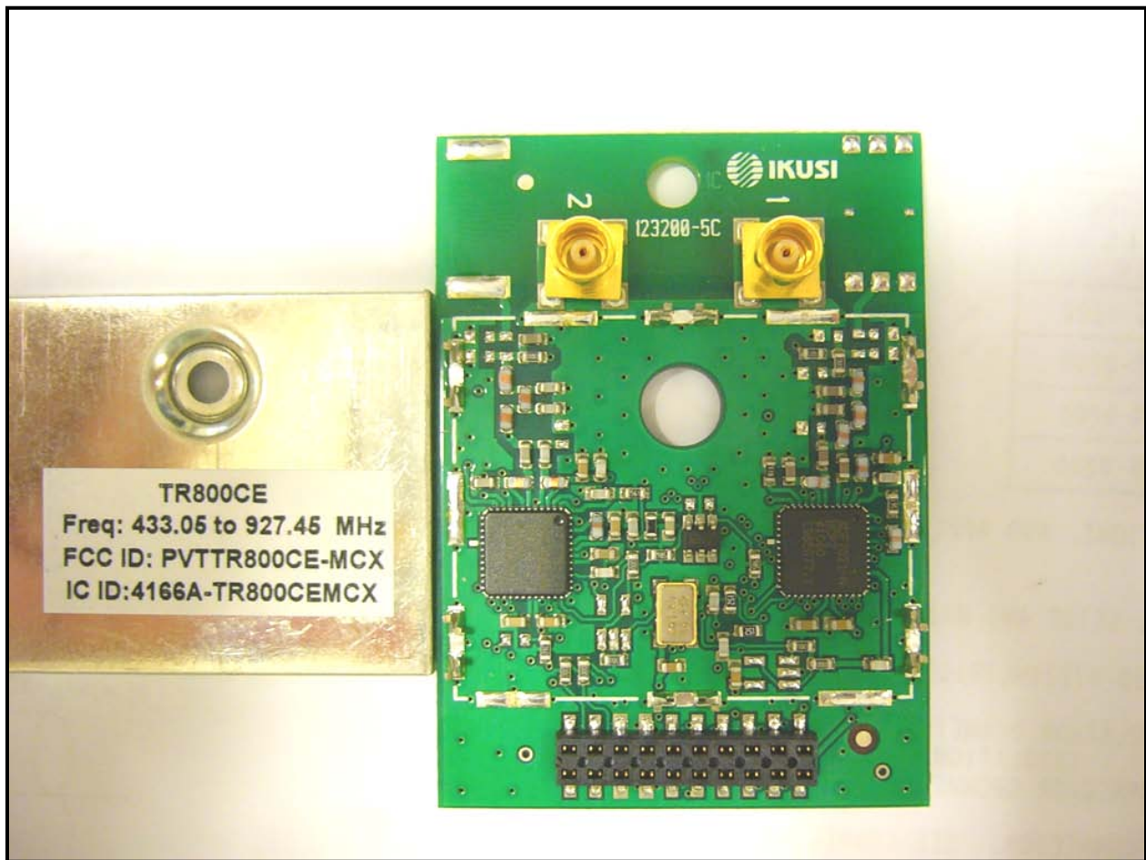
Photograph 8: EUT Top View without Shield
