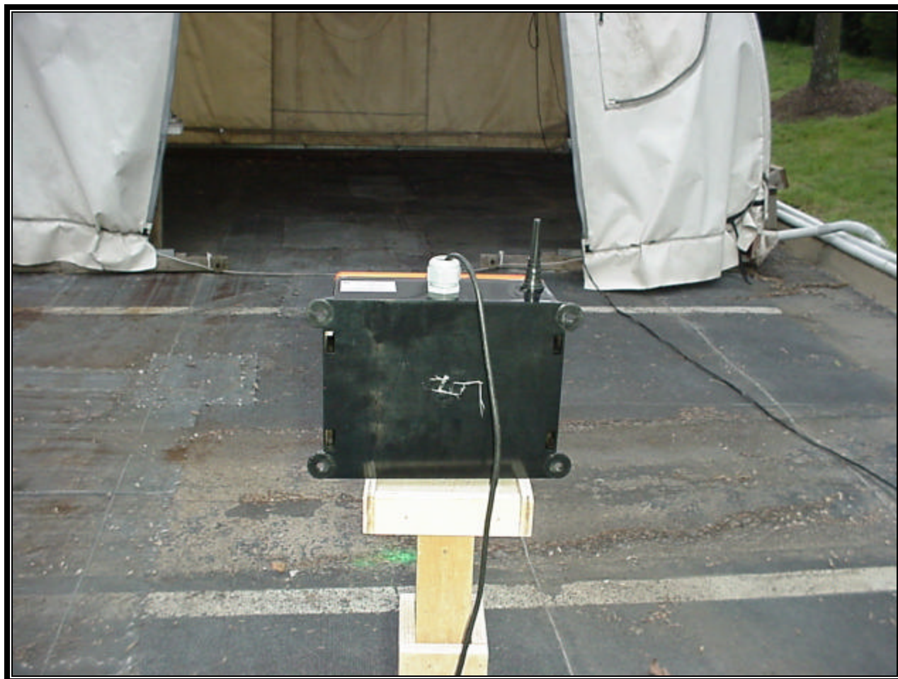
Photograph 2: Radiated Emission Rear View – Attached Antenna Configuration
