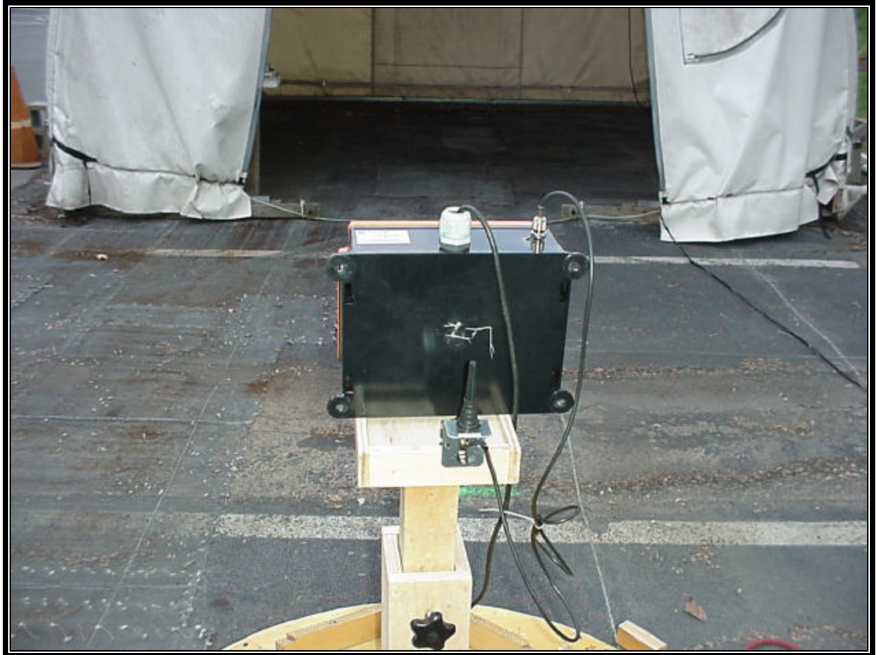
Photograph 4: Radiated Emission Rear View – Unattached Antenna Configuration
