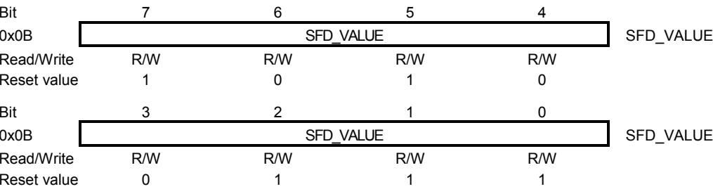
Figure 11-28. Register SFD_VALUE.
