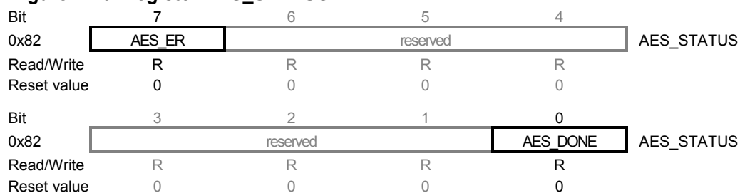
Figure 11-6. Register AES_STATUS.
