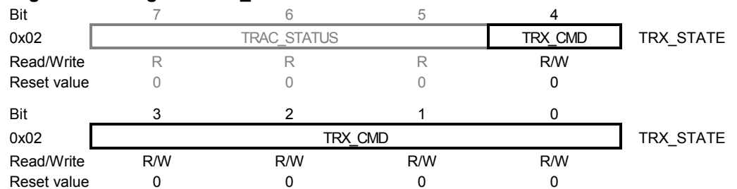
Figure 7-10. Register TRX_STATE.
