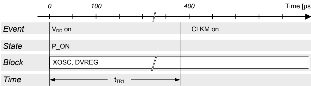
Figure 7-3. Power-on Procedure to P_ON State.
