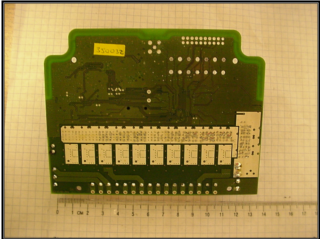
Photograph 7: PCB Bottom
