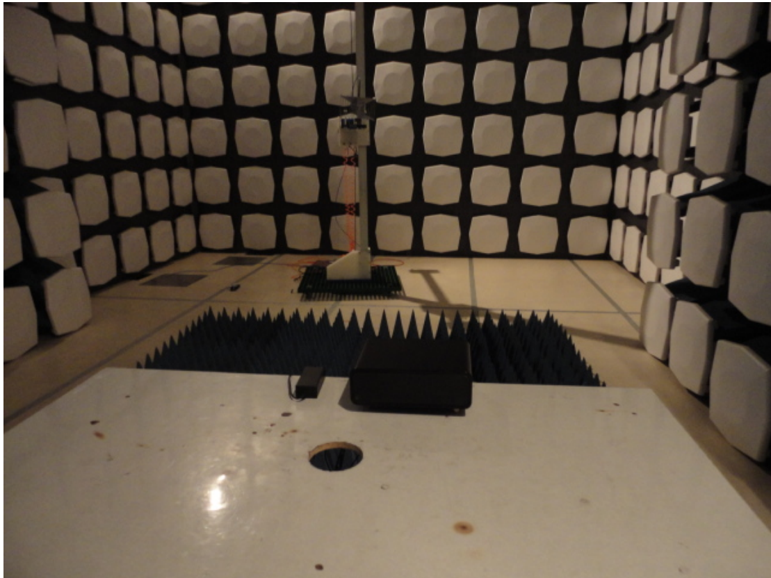
3: Radiated emission (>1000MHz)
