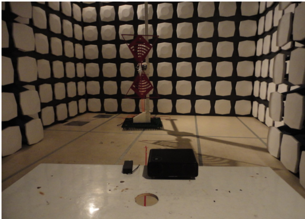
2: Radiated emission (30-1000MHz)
