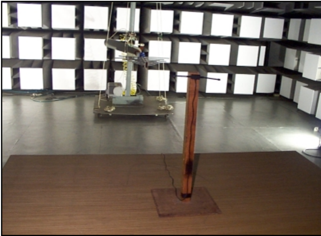
Photograph of the test configuration
