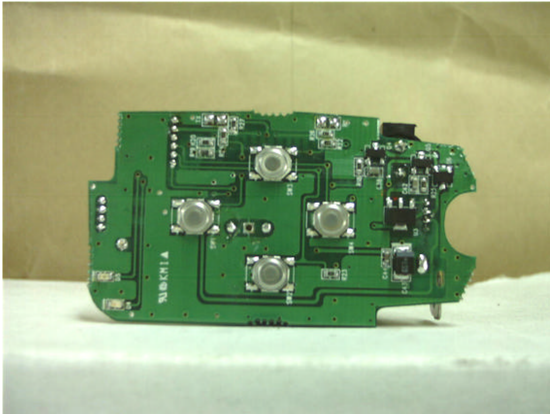
GTL-3001R PHOTO (CPU PCB TOP SIDE)
