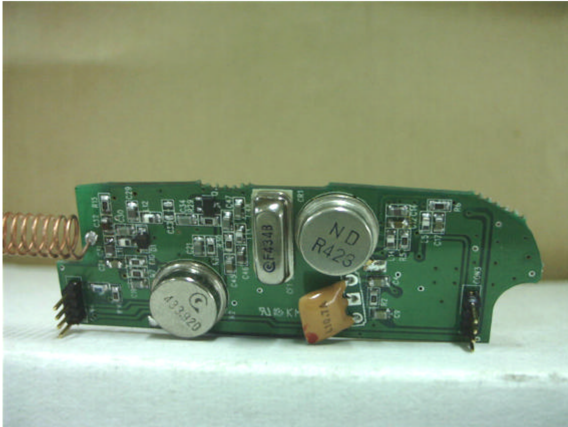
GTL-3001R PHOTO (RF PCB TOP SIDE)
