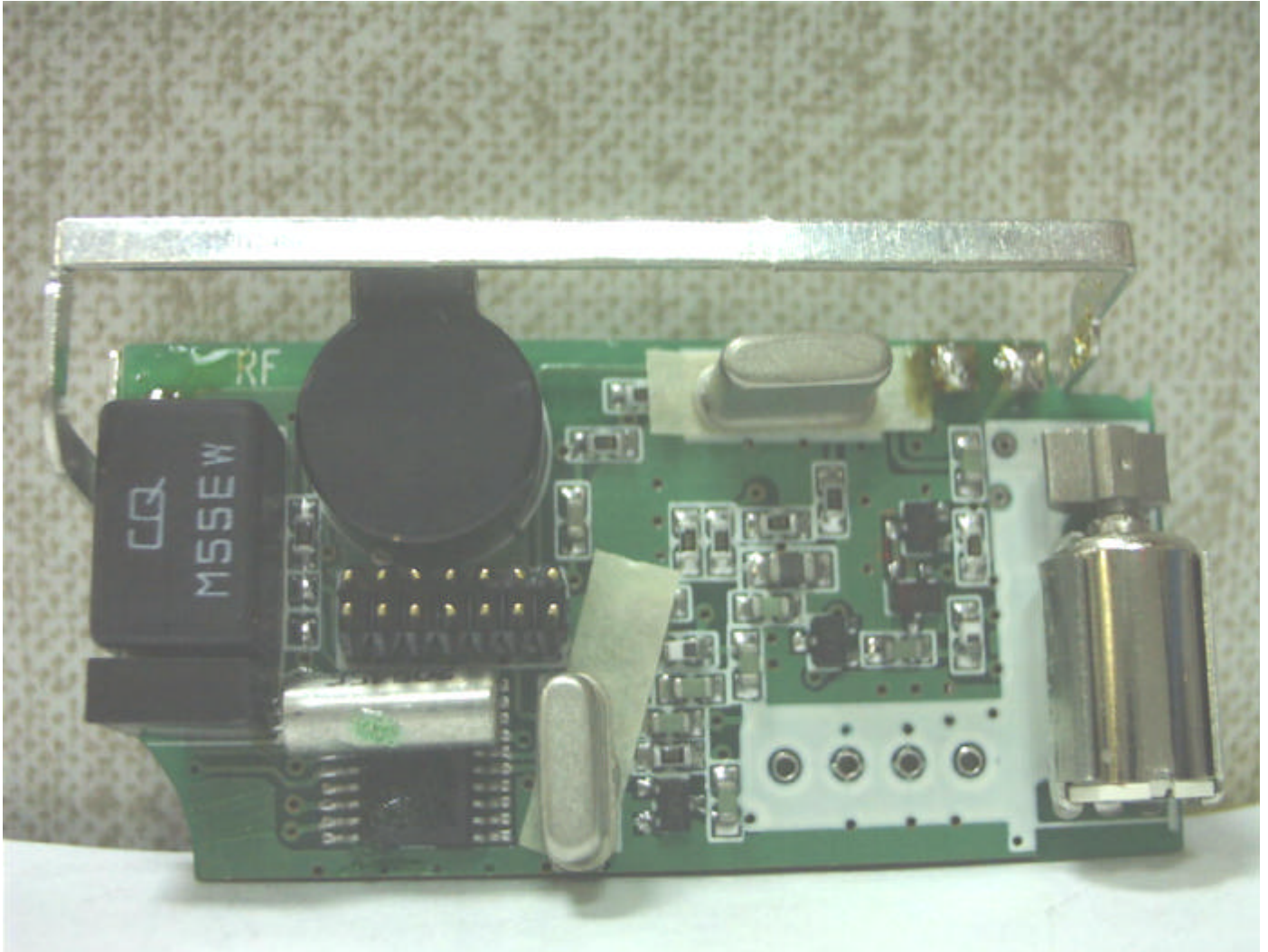
SP-1001R PHOTO (PCB TOP SIDE)
