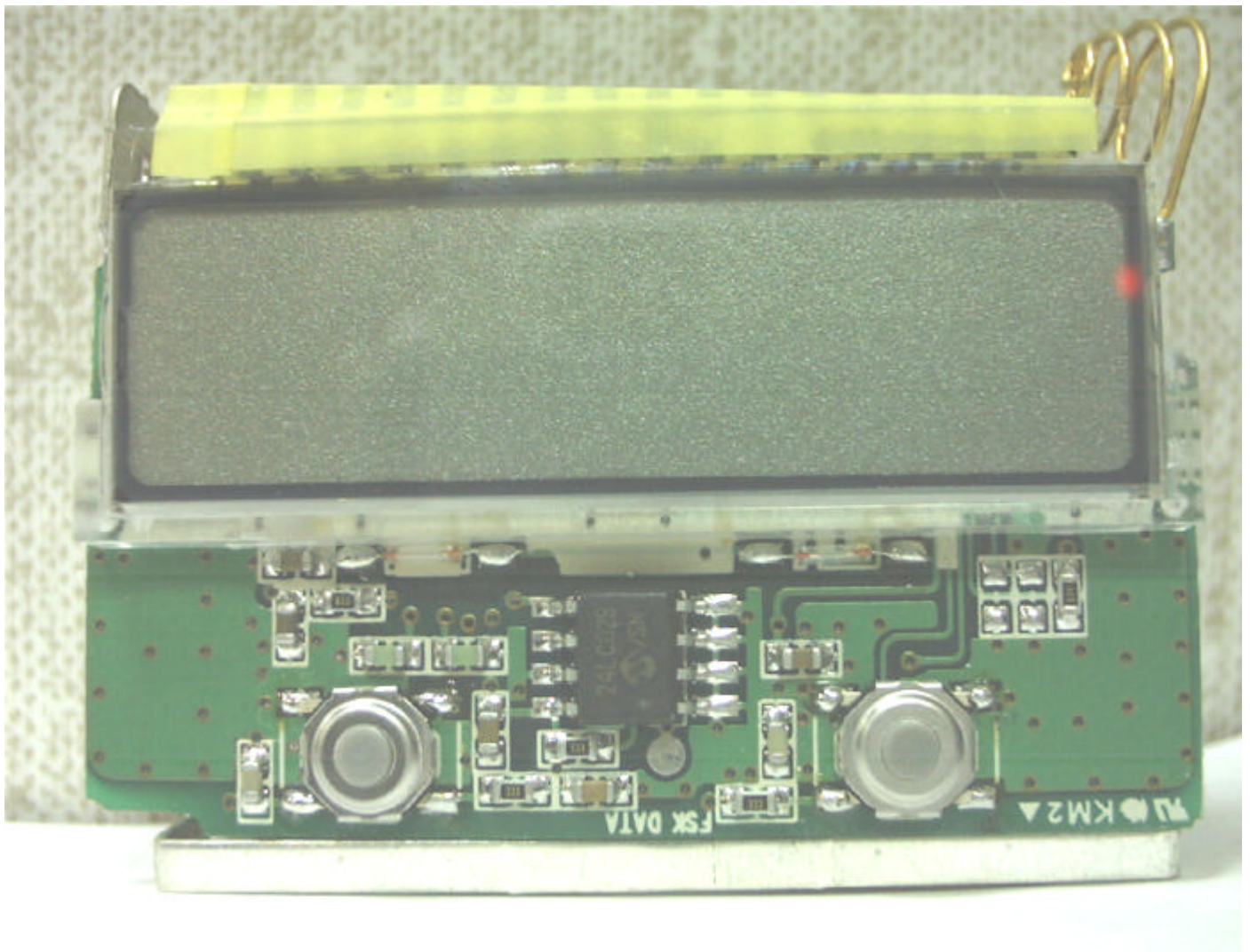
SP-1001R PHOTO ( CPU PCB TOP SIDE)
