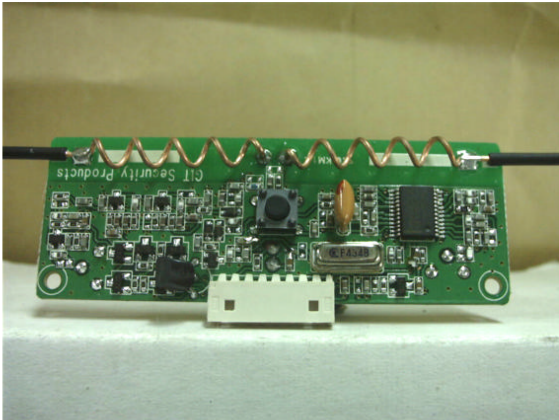
GTL-3001B PHOTO (PCB TOP SIDE)
