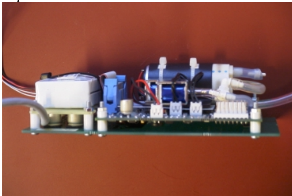
Pump PCB side
