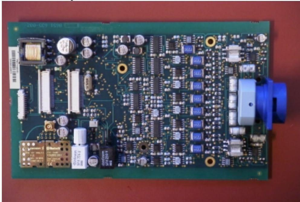
Transmitter PCB top
