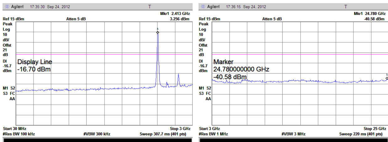
(Plot G.1: Channel = 1, 30MHz to 3GHz)
