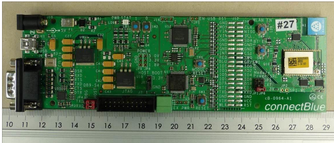
145298_05.jpg: Carrier Board wit EUT – Top View
