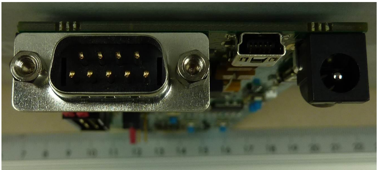
145298_07.JPG: Carrier Board – Connectors
