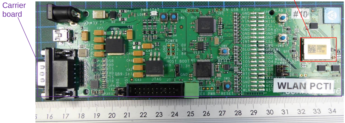
160912_2.jpg: EUT + test PCB – top view
