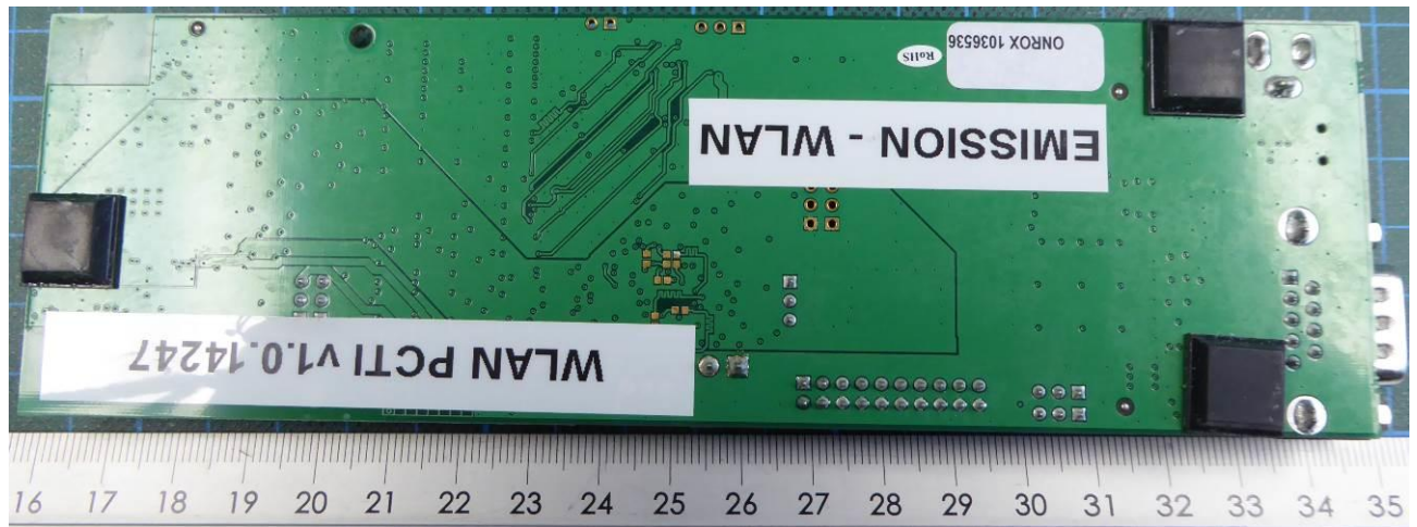
160912_3.jpg: EUT + test PCB – bottom view
