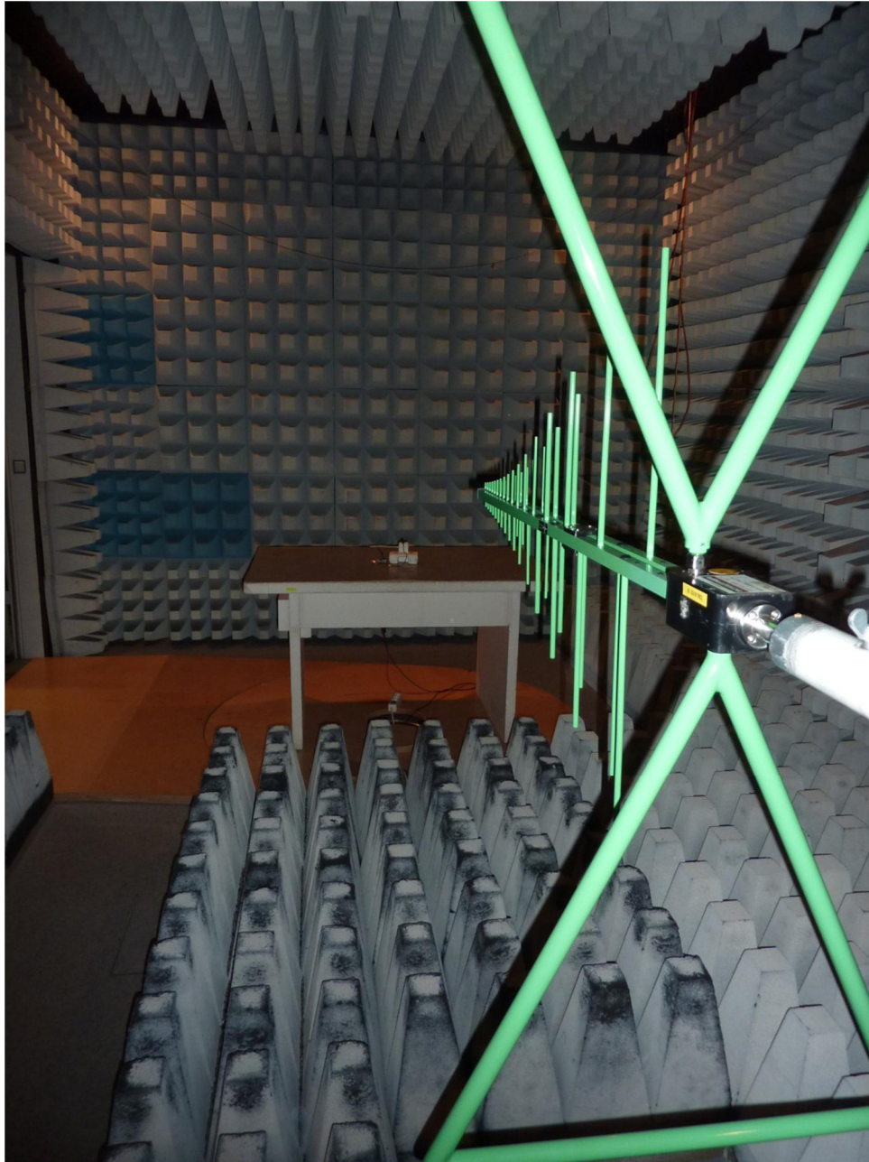
124266_1.JPG: Test setup fully anechoic chamber
