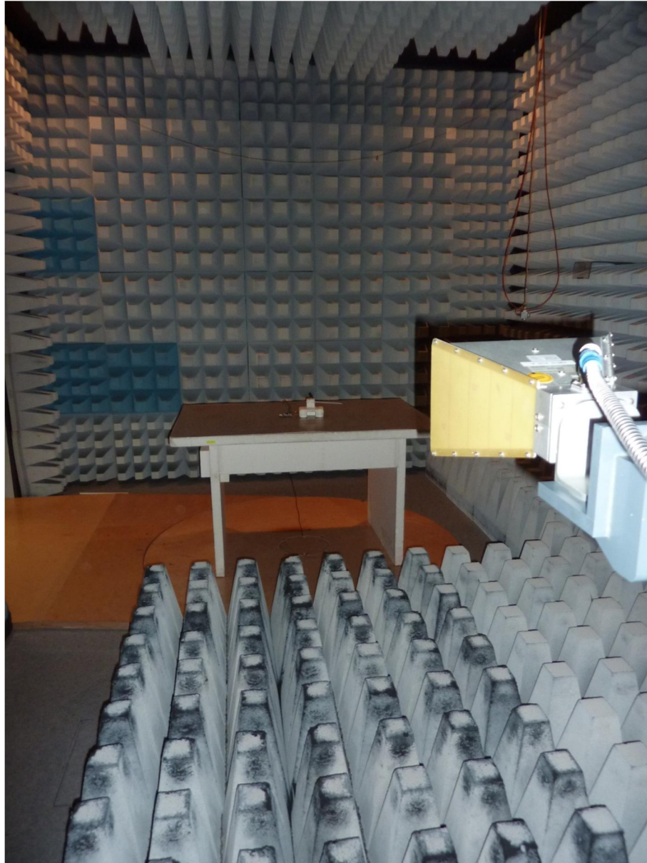
124266_2.JPG: Test setup fully anechoic chamber
