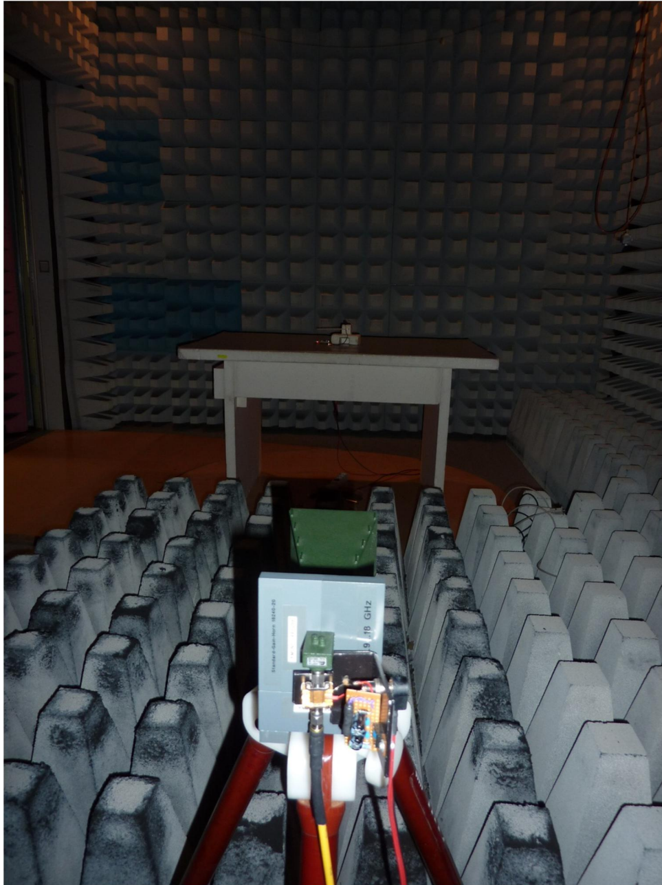
124266_3.JPG: Test setup fully anechoic chamber
