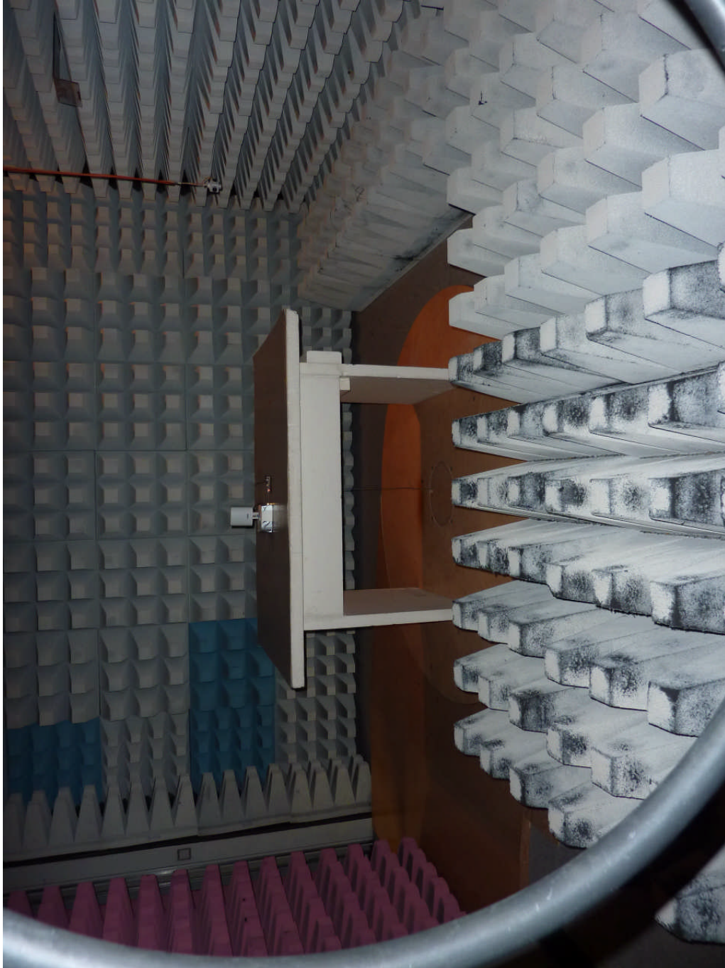
111592_16.JPG: cB-0946 with external patch antenna, test setup fully anechoic chamber
