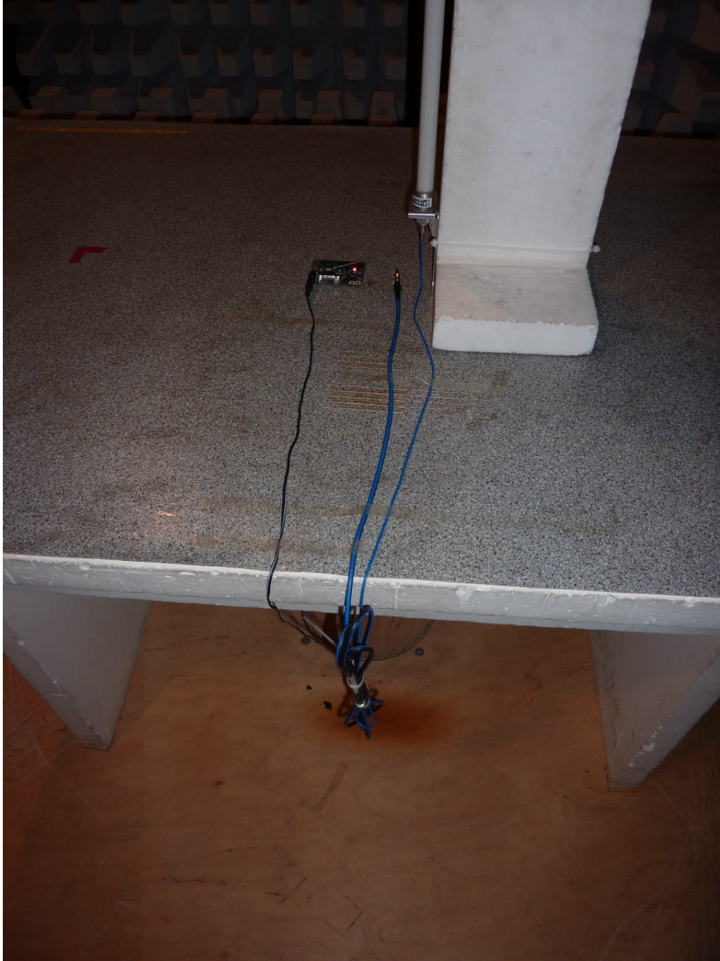
111592_9.JPG: cB-0946 with external monopole antenna, test setup fully anechoic chamber (pos. 1)
