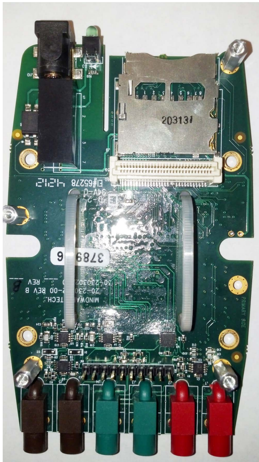
MindWare Mobile Impedance Board Top
