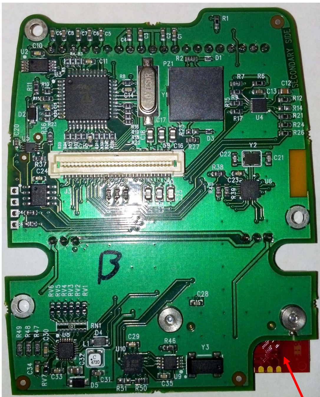
MindWare Mobile CPU Board Bottom
