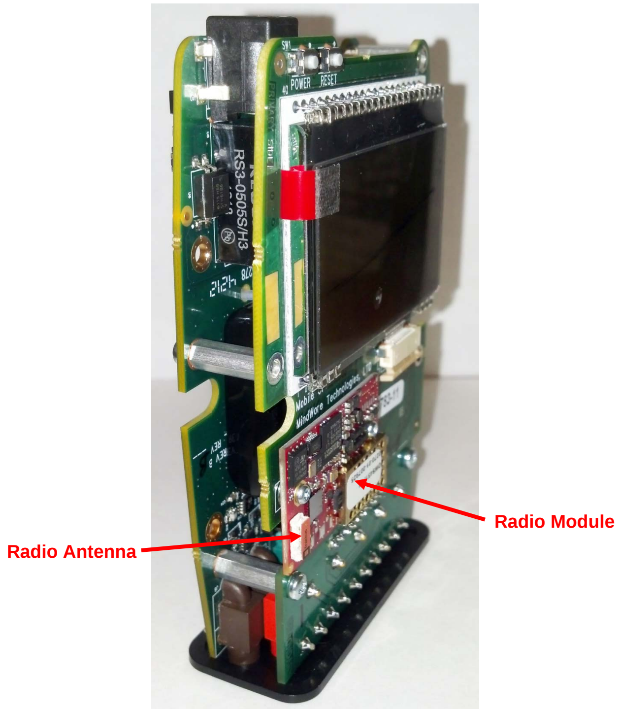
MindWare Mobile Front and Left Side
