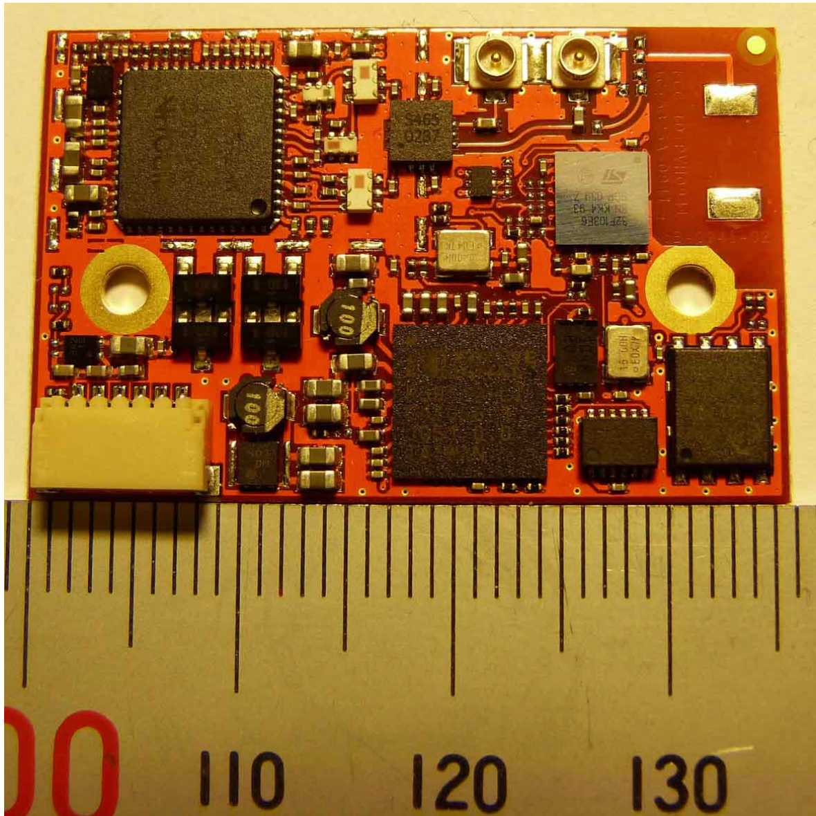
Photo 6 cB-0941-02 External antenna with CPU and JST connector (OWS451x-06)
