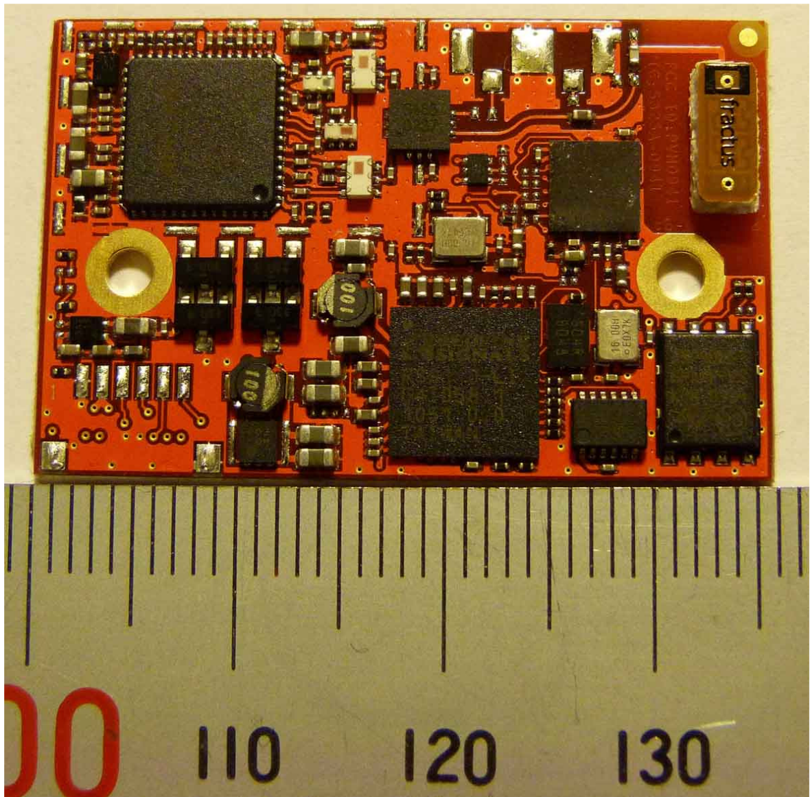
Photo 3 cB-0941-02 Internal antenna with CPU without JST connector (OWS451i-04)
