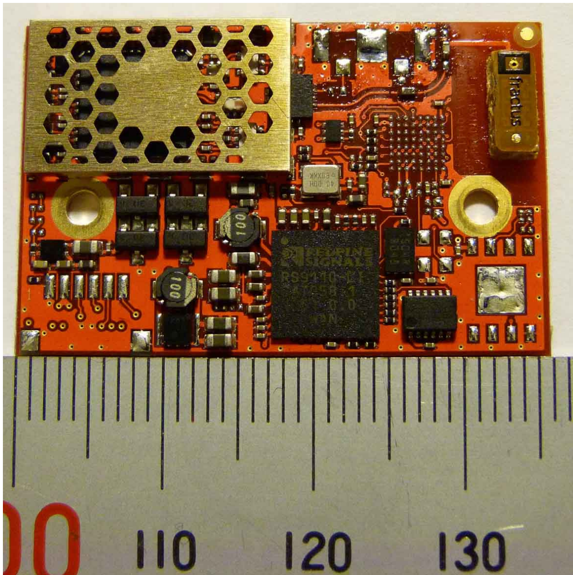
Photo 1 cB-0941-02 Internal antenna without CPU and JST connector (OWL253i-04)
