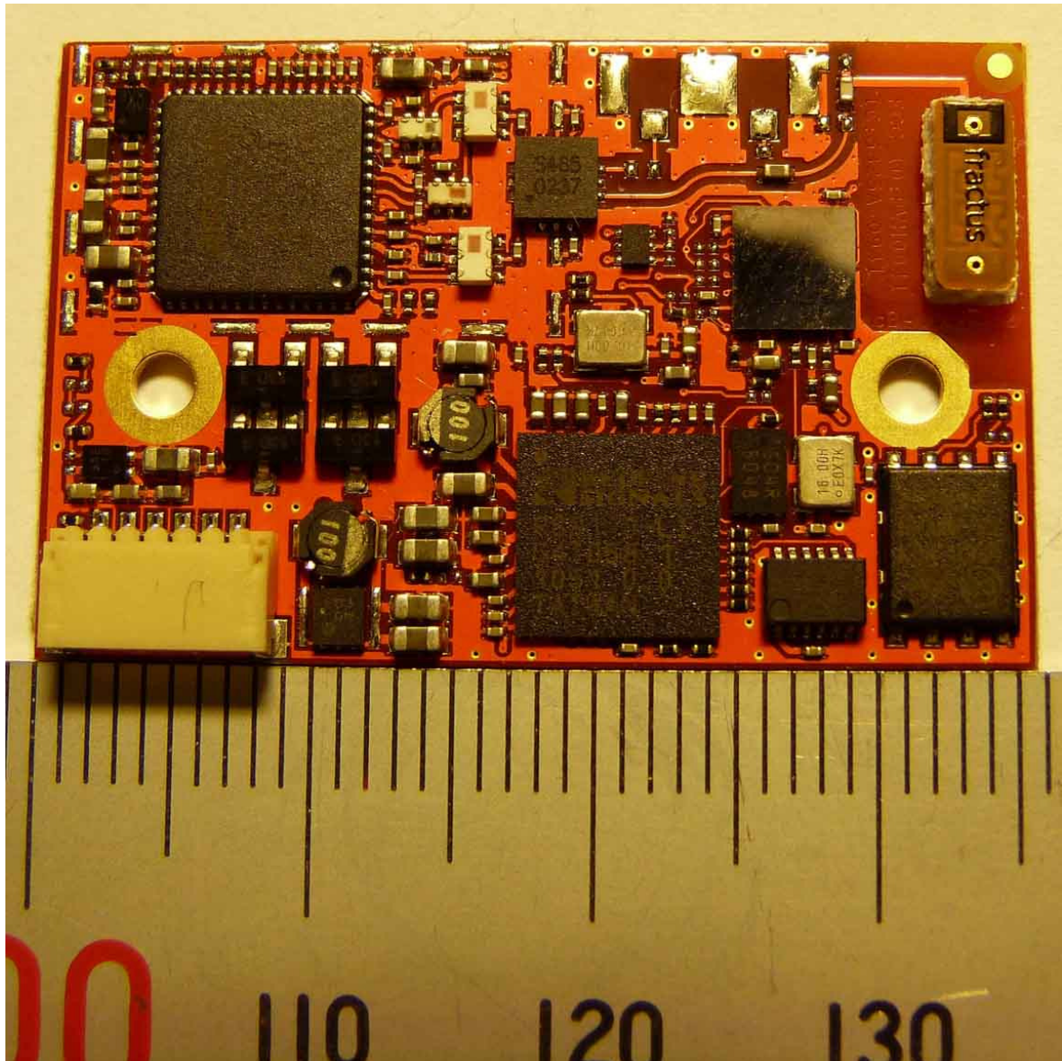
Photo 5 cB-0941-02 Internal antenna with CPU and JST connector (OWS451i-06)
