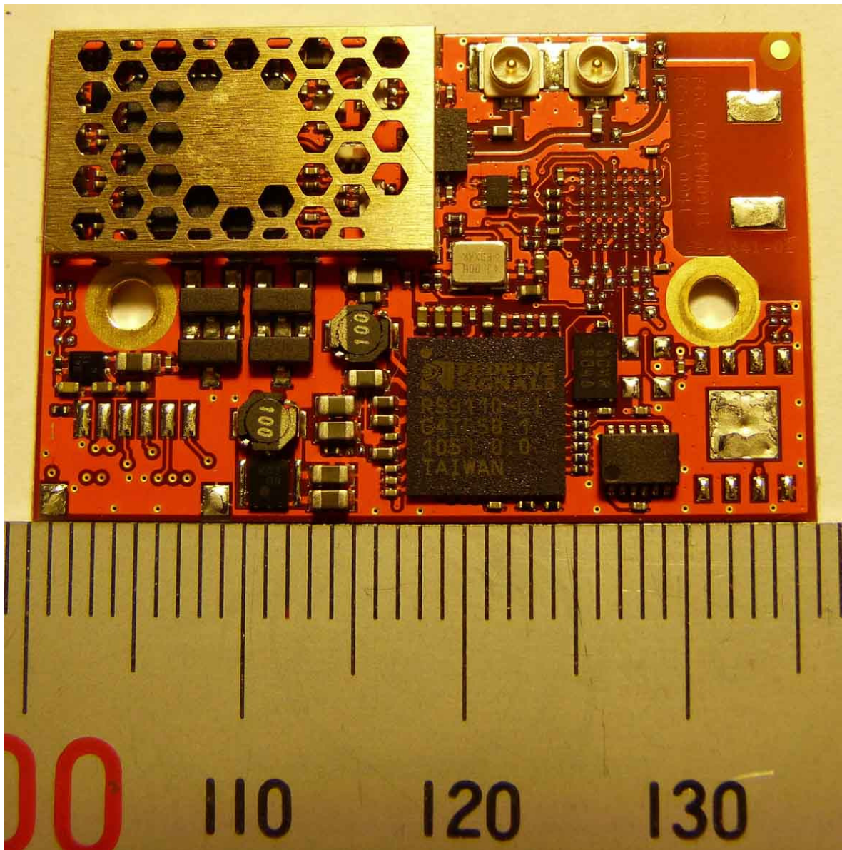
Photo 2 cB-0941-02 External antenna without CPU and JST connector (OWL253x-04)
