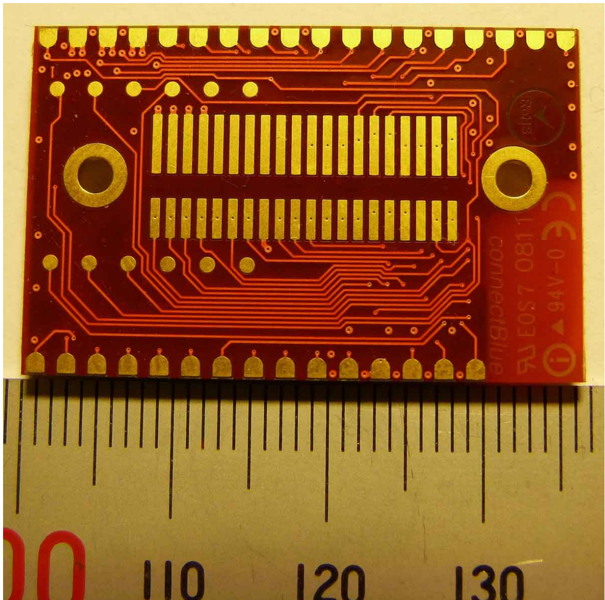
Photo 7 Secondary side of cB-0941-02
