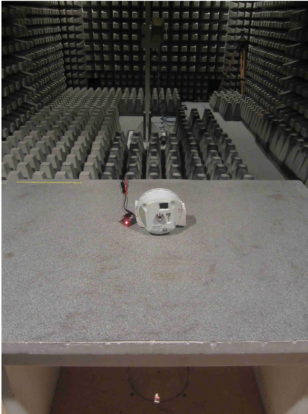
130857_04.JPG: cB-0939 Antenna in housing, test setup fully anechoic chamber, 1 – 12 GHz
