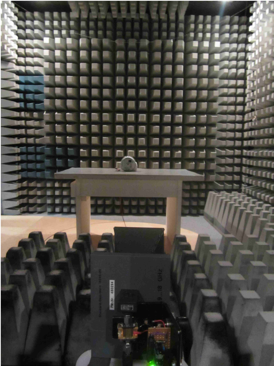
130857_07.JPG: cB-0939 Antenna in housing, test setup fully anechoic chamber, 12 – 18 GHz
