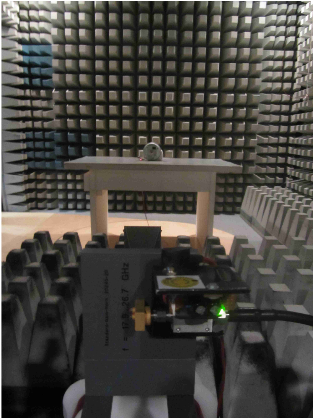
130857_08.JPG: cB-0939 Antenna in housing, test setup fully anechoic chamber, 18 – 25 GHz
