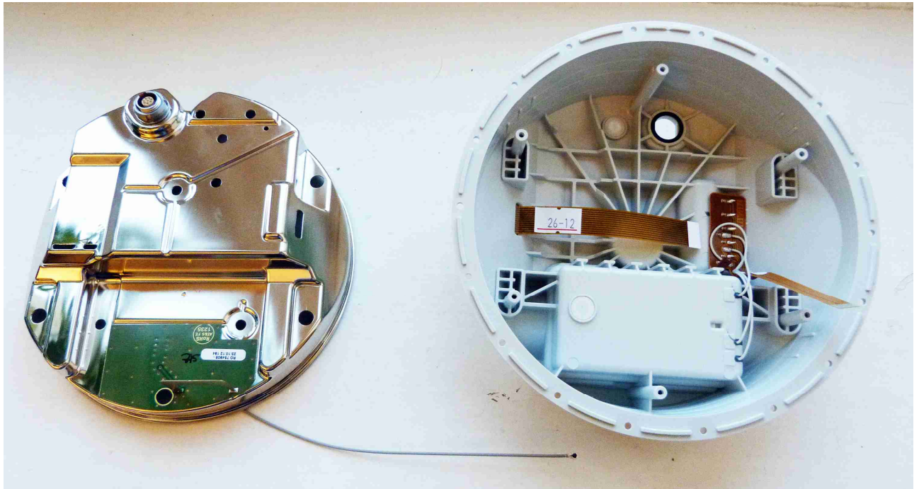
130857_26.JPG: BTAB-2450 Antenna housing – internal view
