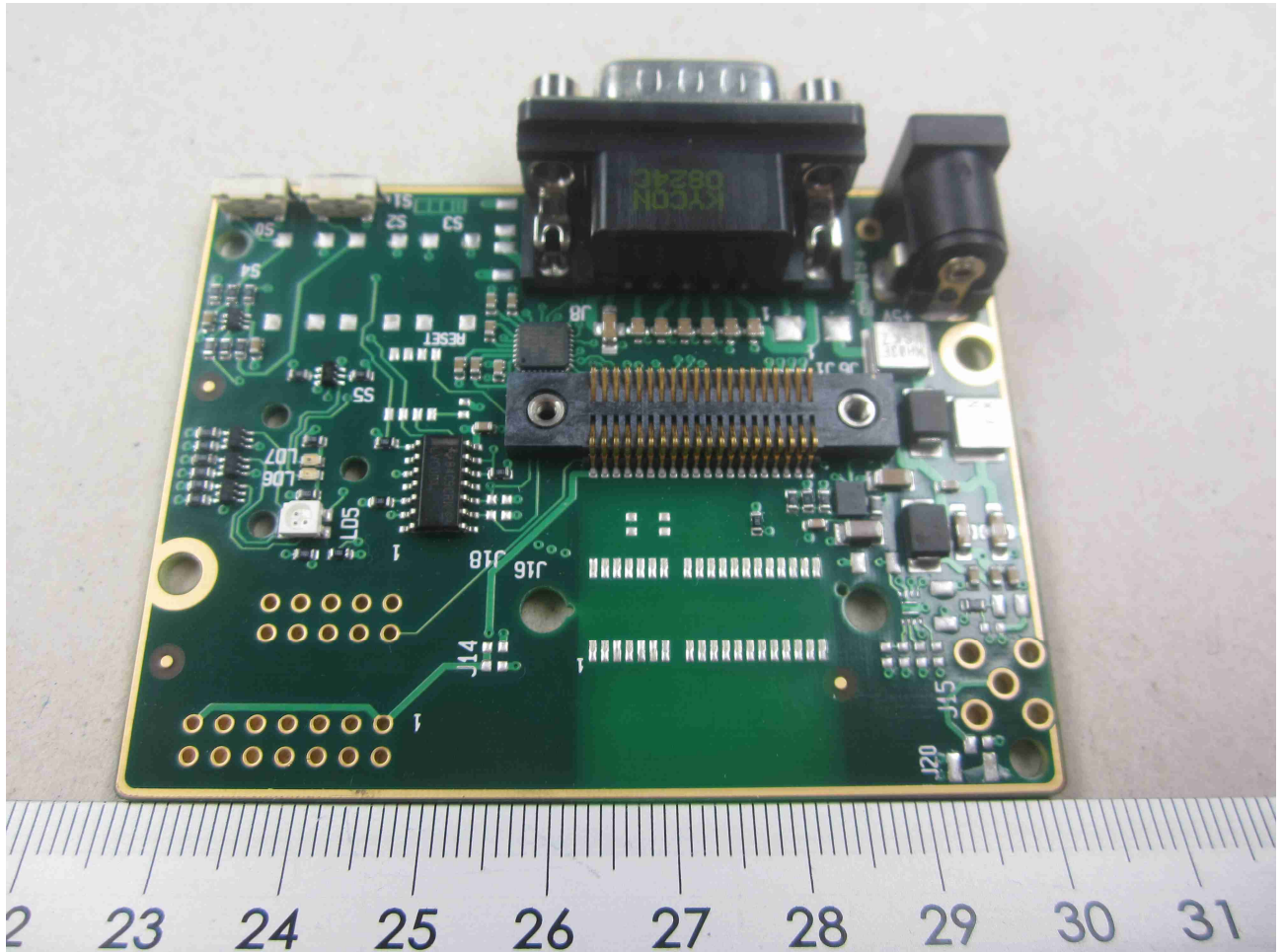
130857_20.JPG: cB-0903-03, top view, cB-0939 removed
