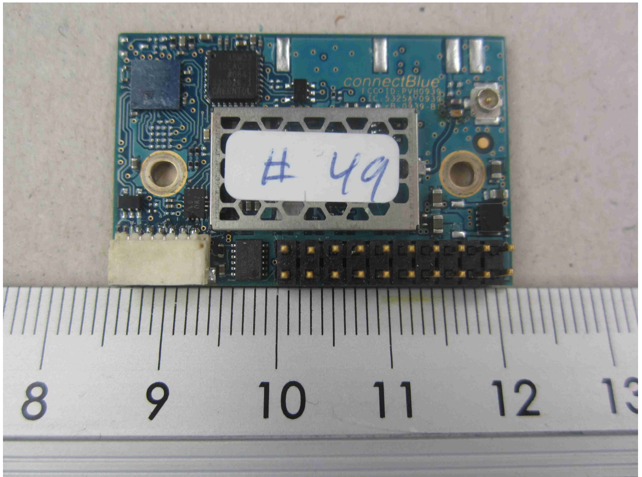
130857_21.JPG: cB-0939, PCB, top view
