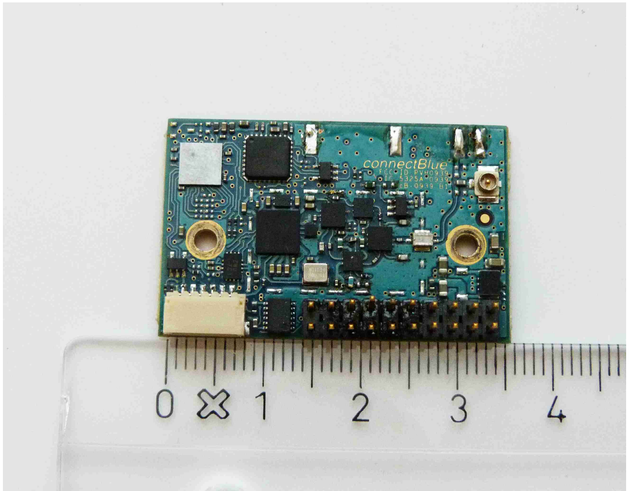
130857_29.JPG: cB-0939, PCB, top view, shielding removed
