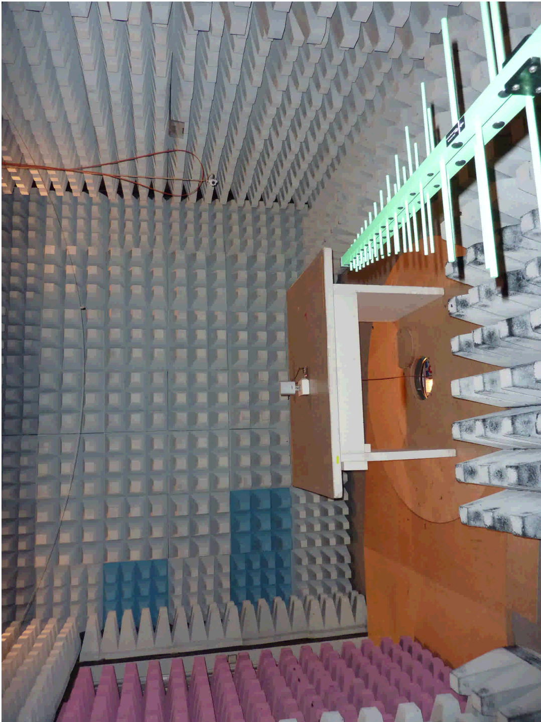
101347_12.jpg: cB-0939-B1-02, test set-up fully anechoic chamber
