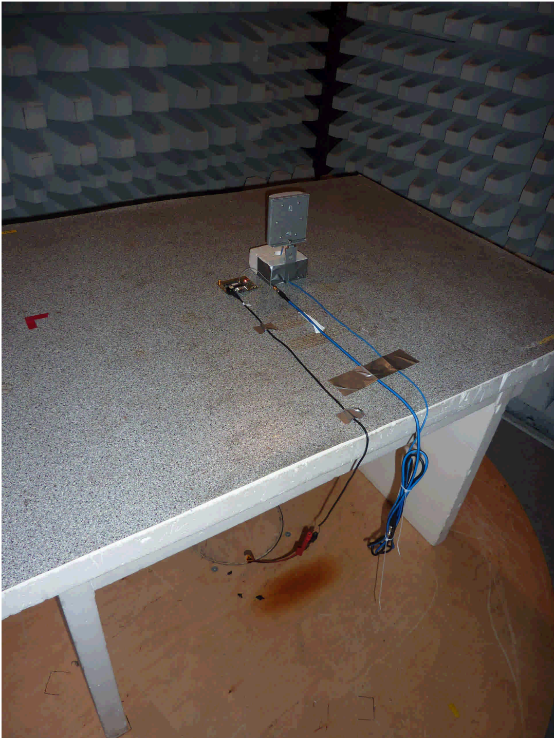
101347_4.jpg: cB-0939-B1-02 with patch antenna, test set-up fully anechoic chamber
