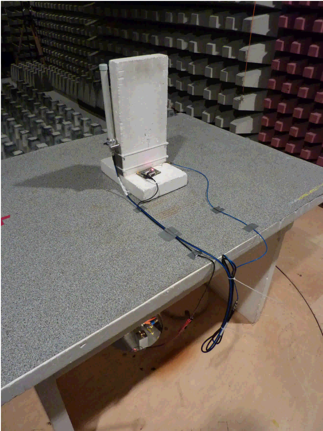
101347_3.jpg: cB-0939-B1-02 with monopole antenna, test set-up fully anechoic chamber
