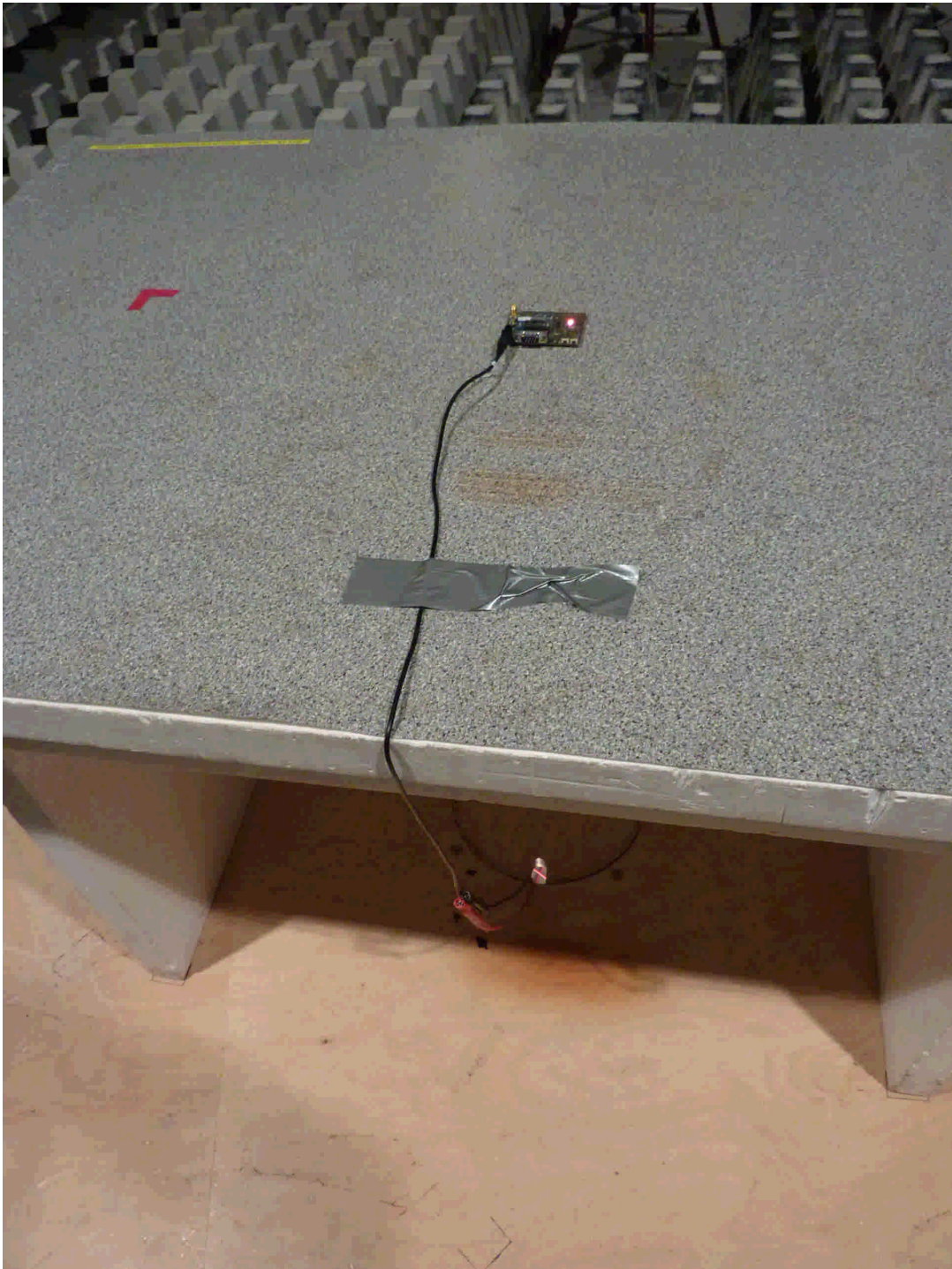
101347_19.jpg: cB-0939-B1-01 with internal antenna, test set-up fully anechoic chamber
