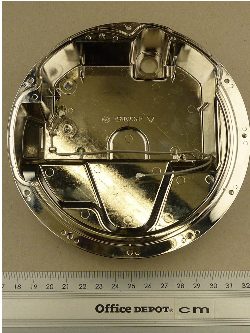
122631_4.jpg Antenna BBL-2450, mounted on chrome plated enclosure, top view
