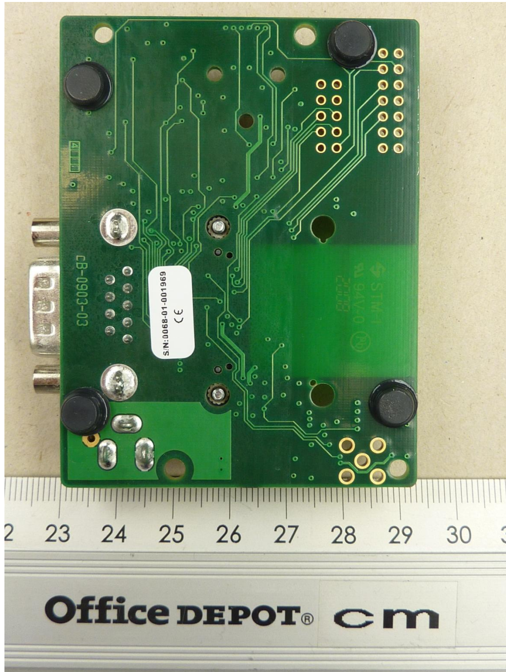
122631_6.jpg cB-0903-03, carrier board, bottom view
