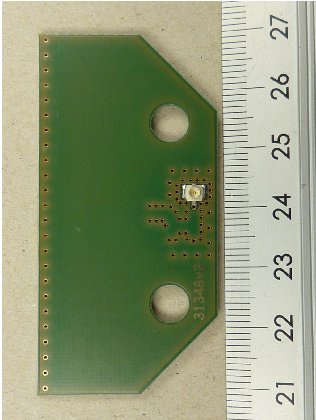
122631_1.jpg Antenna BBL-2450, top view
