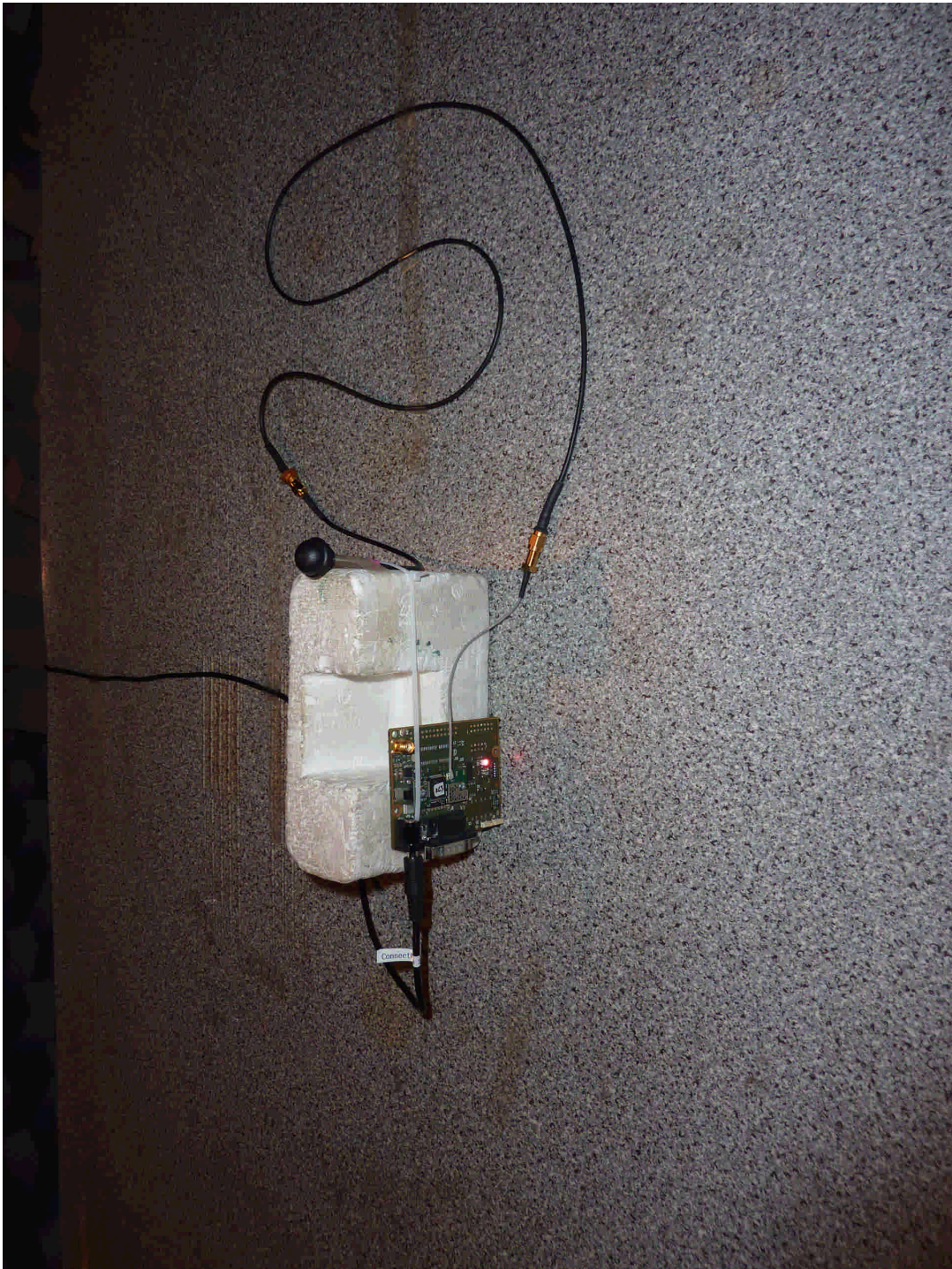
103572_1.jpg cB-0925-01-1-01, test set-up fully anechoic chamber
