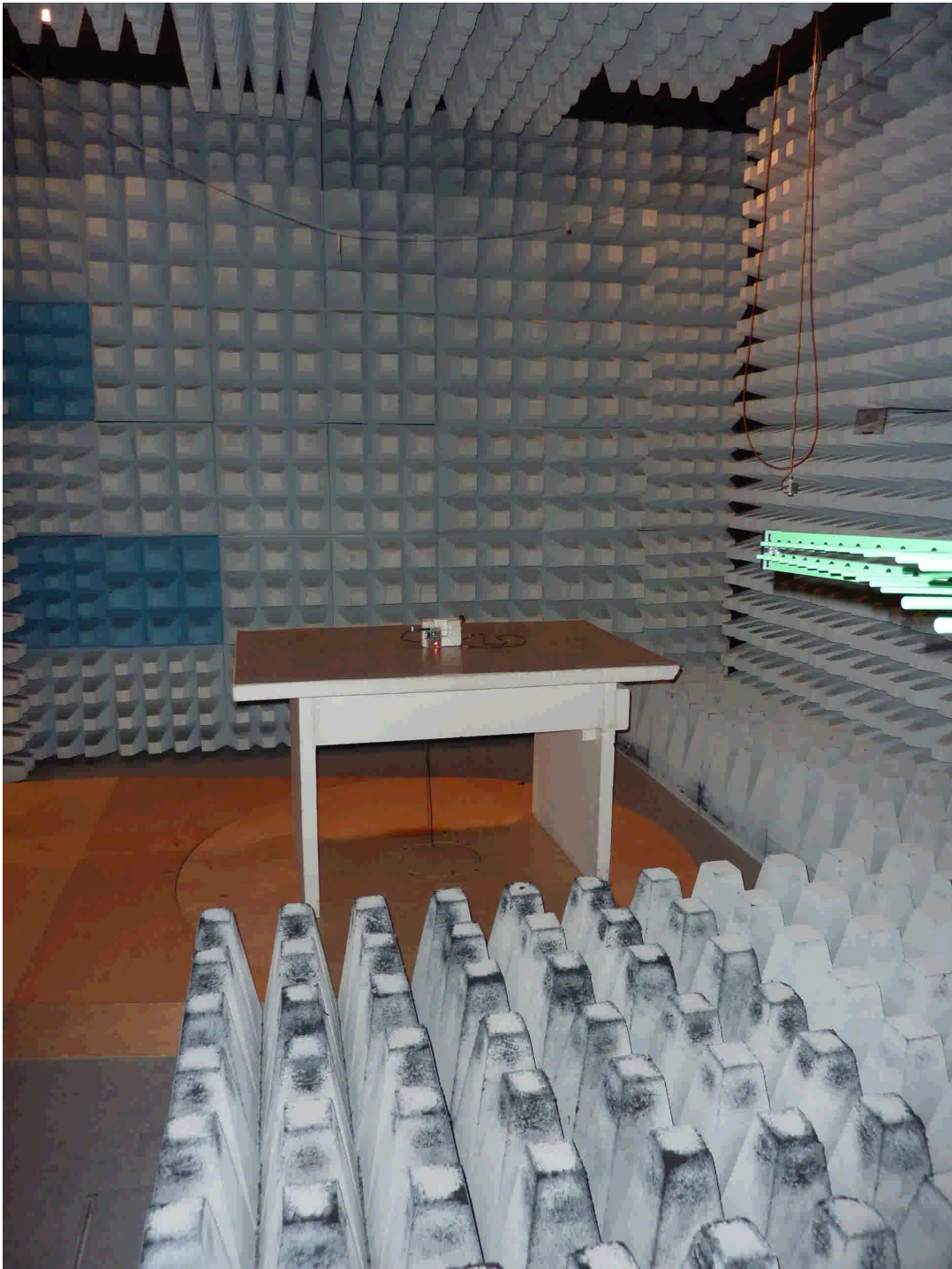
103572_3.jpg cB-0925-01-1-02, test set-up fully anechoic chamber
